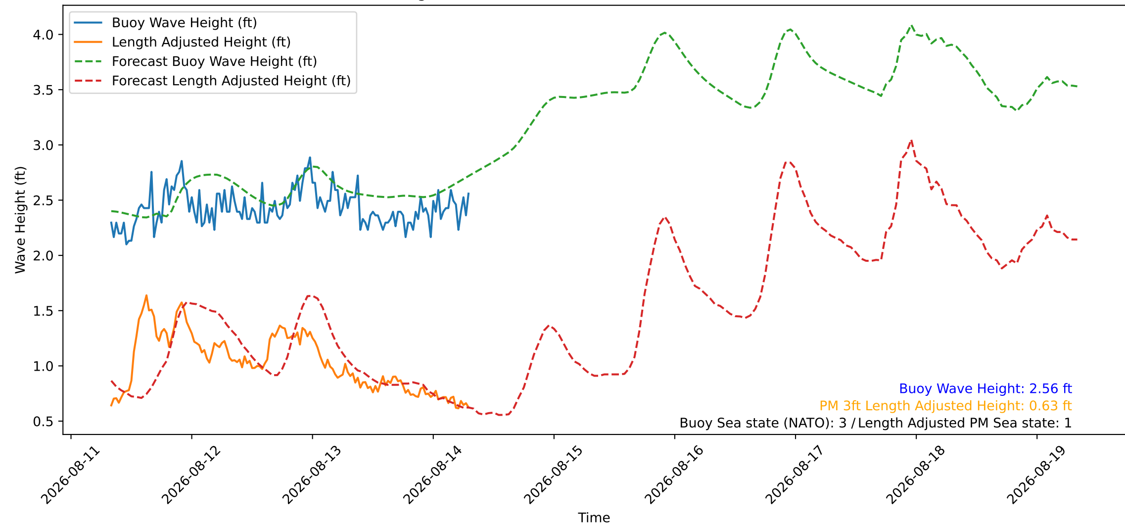
Wave Heights over Time for Red Beach at 2026-08-14 07:40:46
