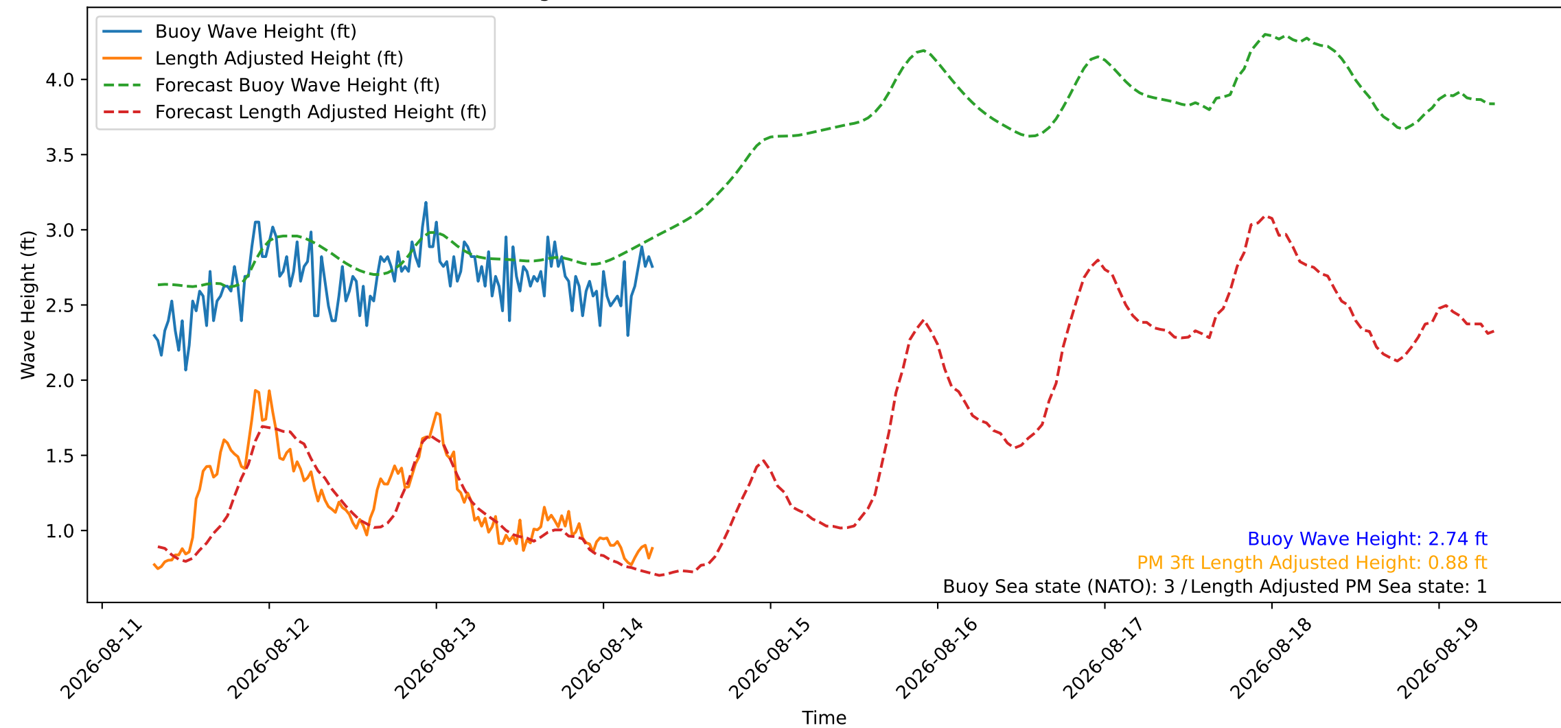
Wave Heights over Time for Oceanside Harbor at 2026-08-14 07:40:27
