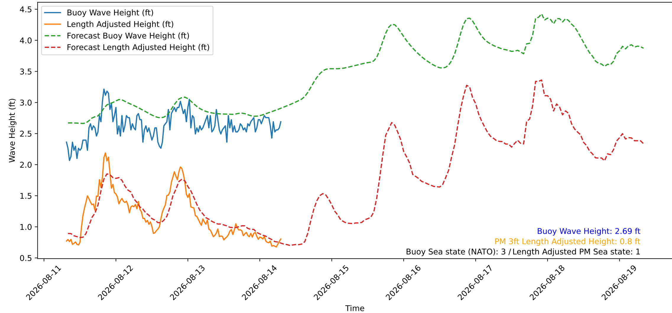
Wave Heights over Time for Green Beach at 2026-08-14 07:41:09
