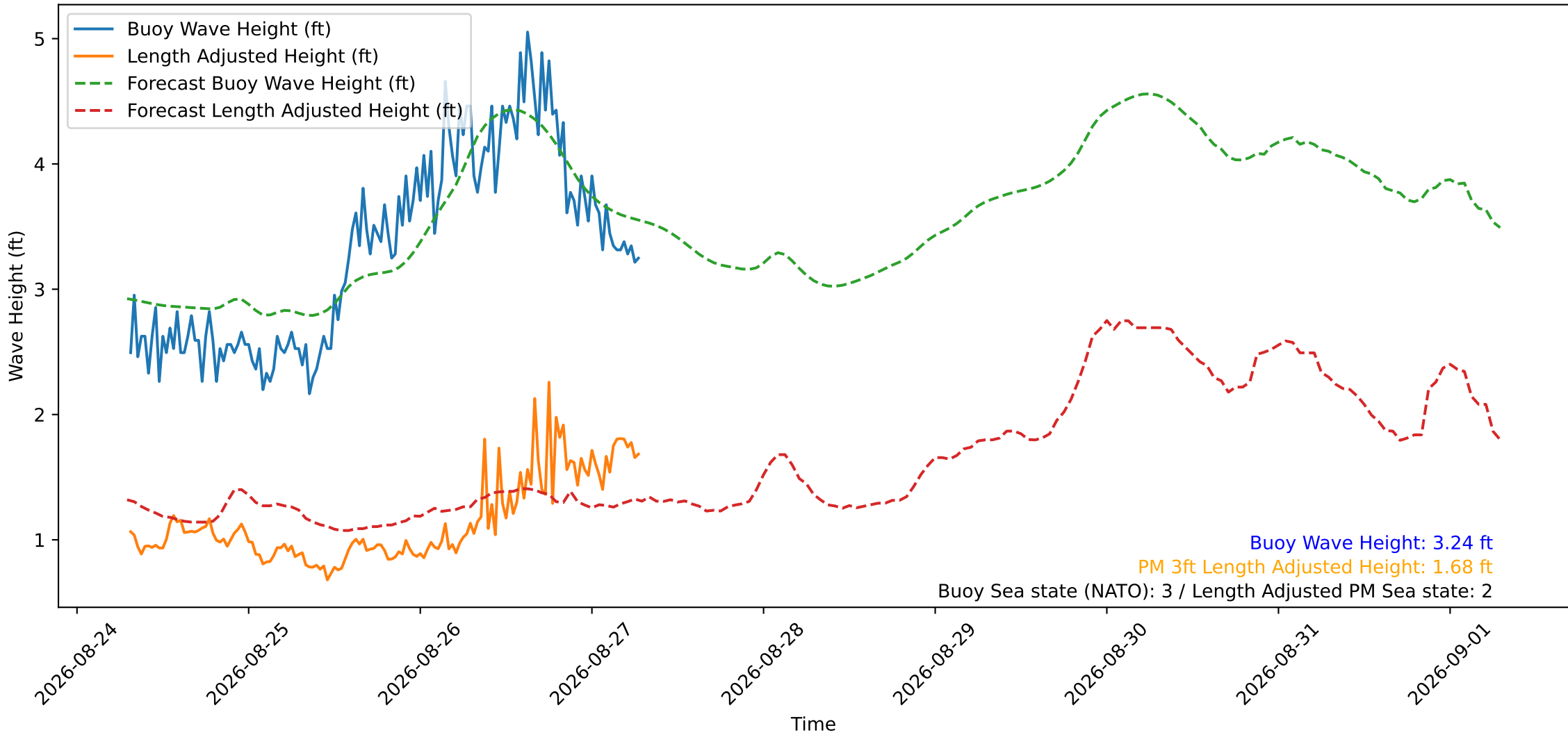
Wave Heights over Time for Red Beach at 2026-08-27 07:20:51
