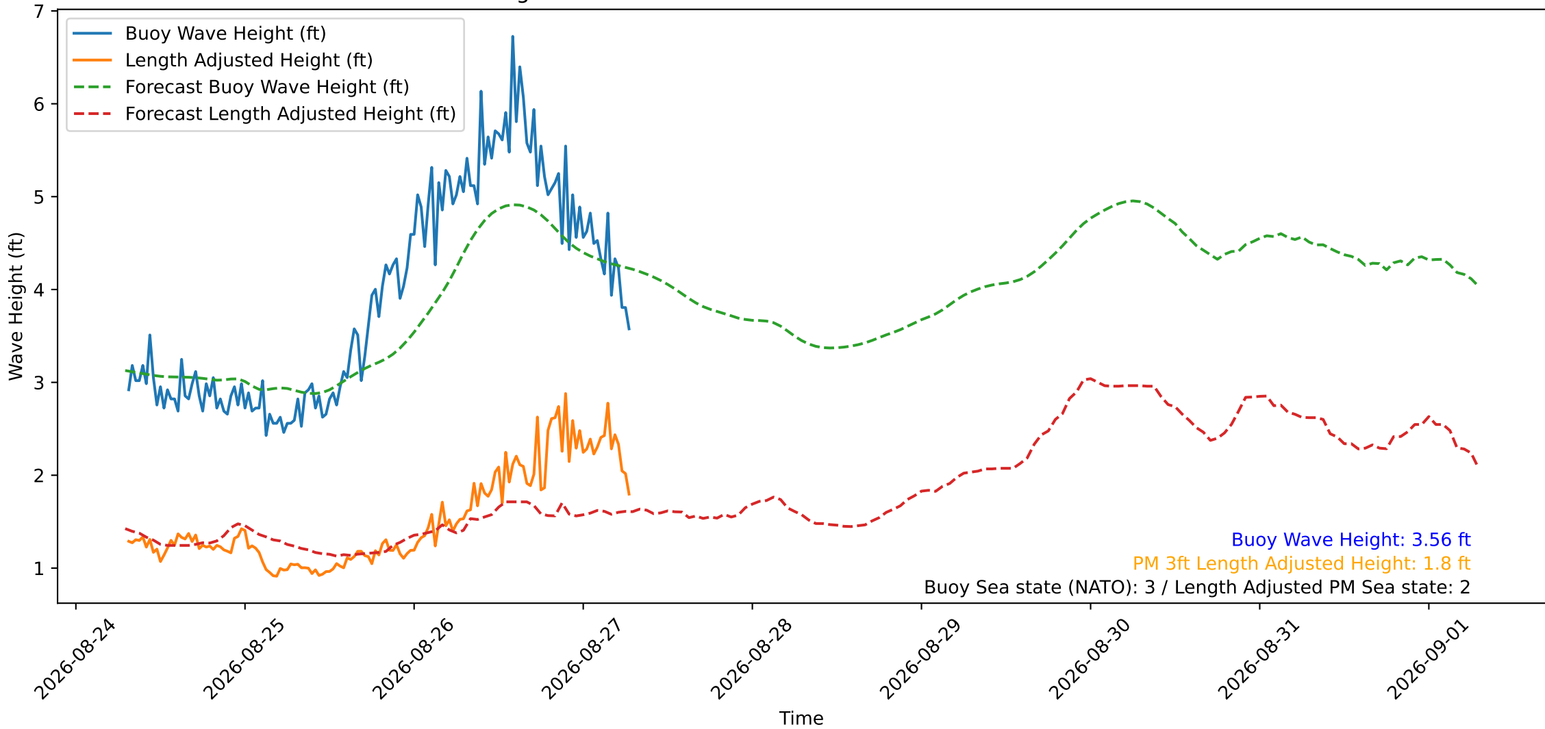
Wave Heights over Time for Oceanside Harbor at 2026-08-27 07:20:30
