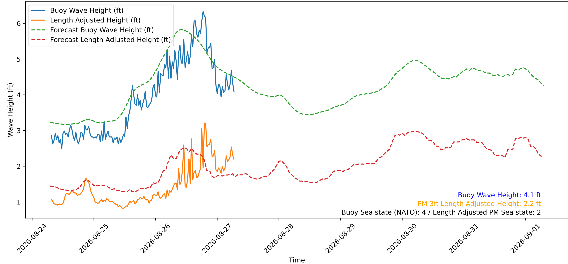
Wave Heights over Time for Green Beach at 2026-08-27 07:21:15
