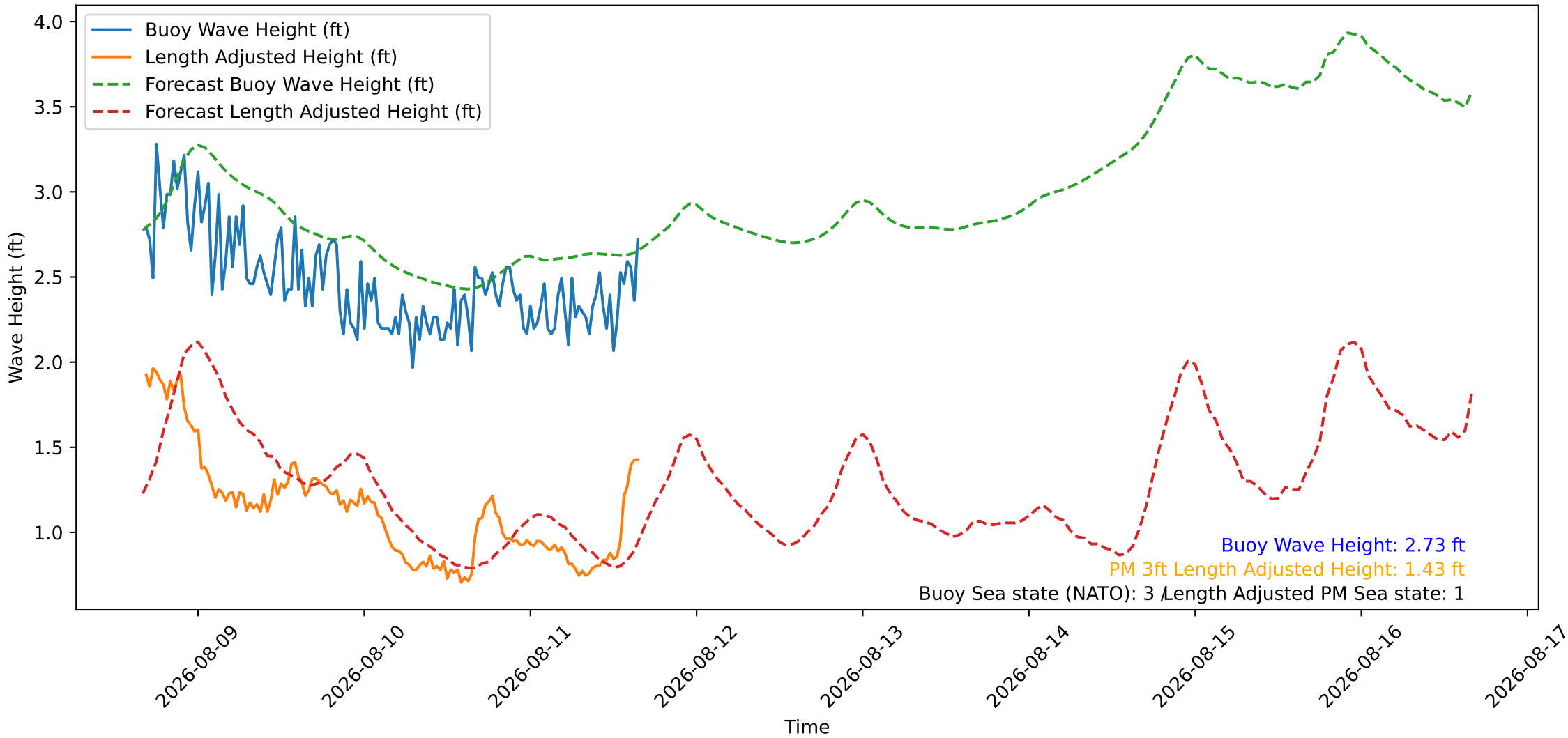
Wave Heights over Time for Oceanside Harbor at 2026-08-11 16:20:26
