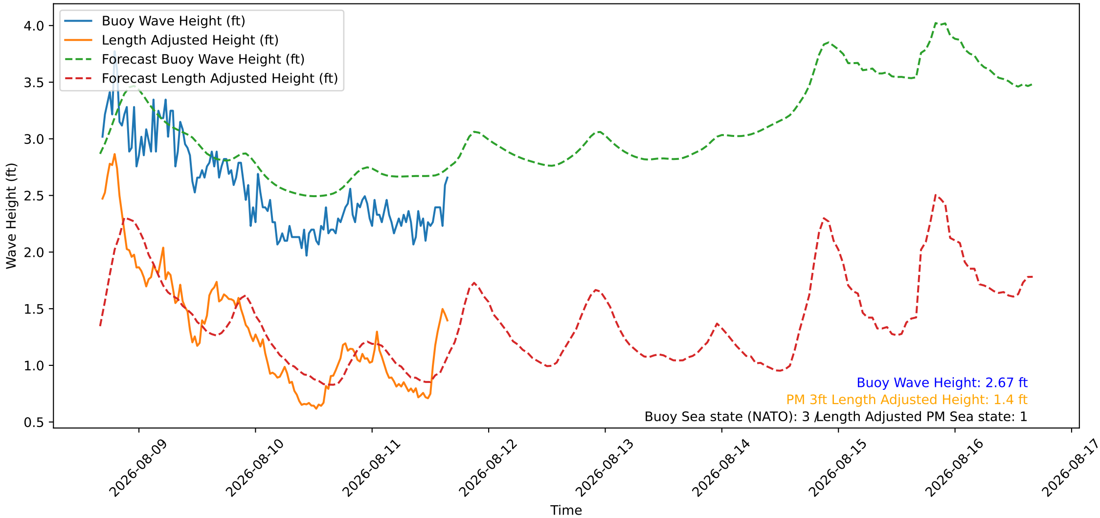
Wave Heights over Time for Green Beach at 2026-08-11 16:21:10
