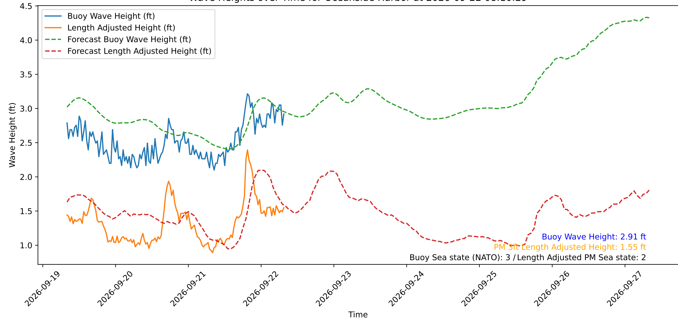
Wave Heights over Time for Oceanside Harbor at 2026-09-22 08:10:29
