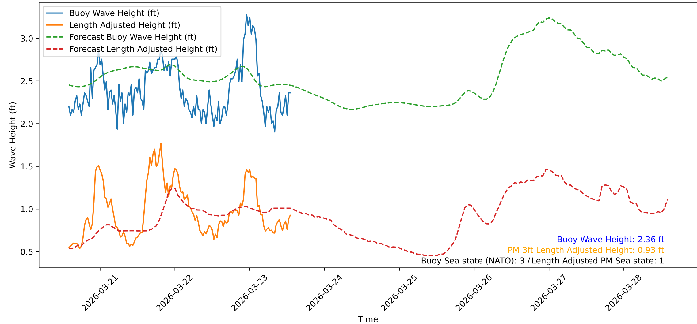
Wave Heights over Time for Green Beach at 2026-03-23 13:51:09
