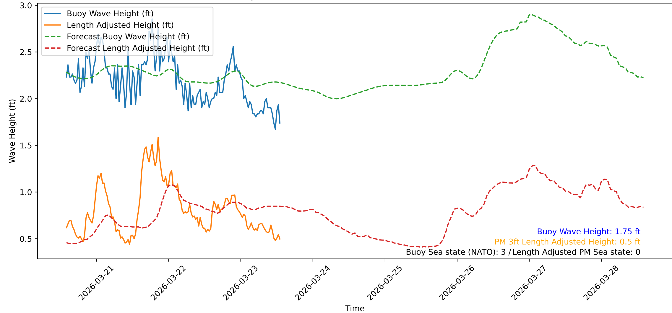
Wave Heights over Time for Red Beach at 2026-03-23 13:50:47
