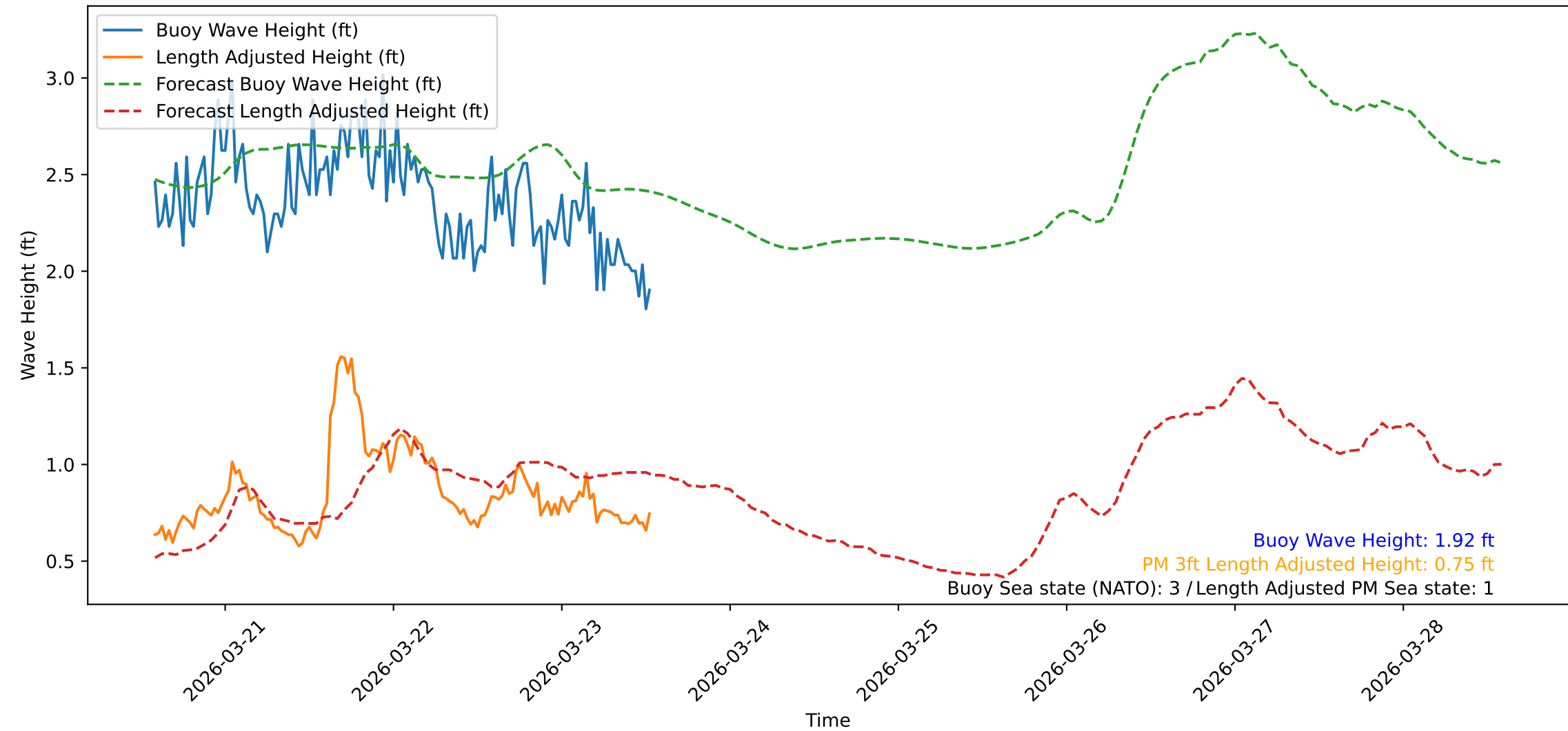
Wave Heights over Time for Oceanside Harbor at 2026-03-23 13:50:31
