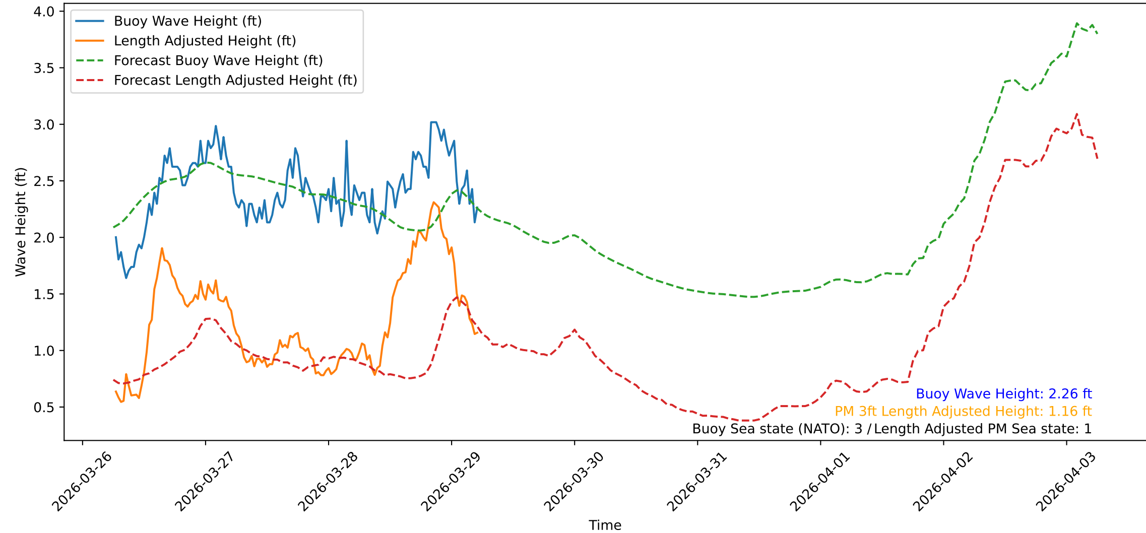
Wave Heights over Time for Red Beach at 2026-03-29 06:00:47
