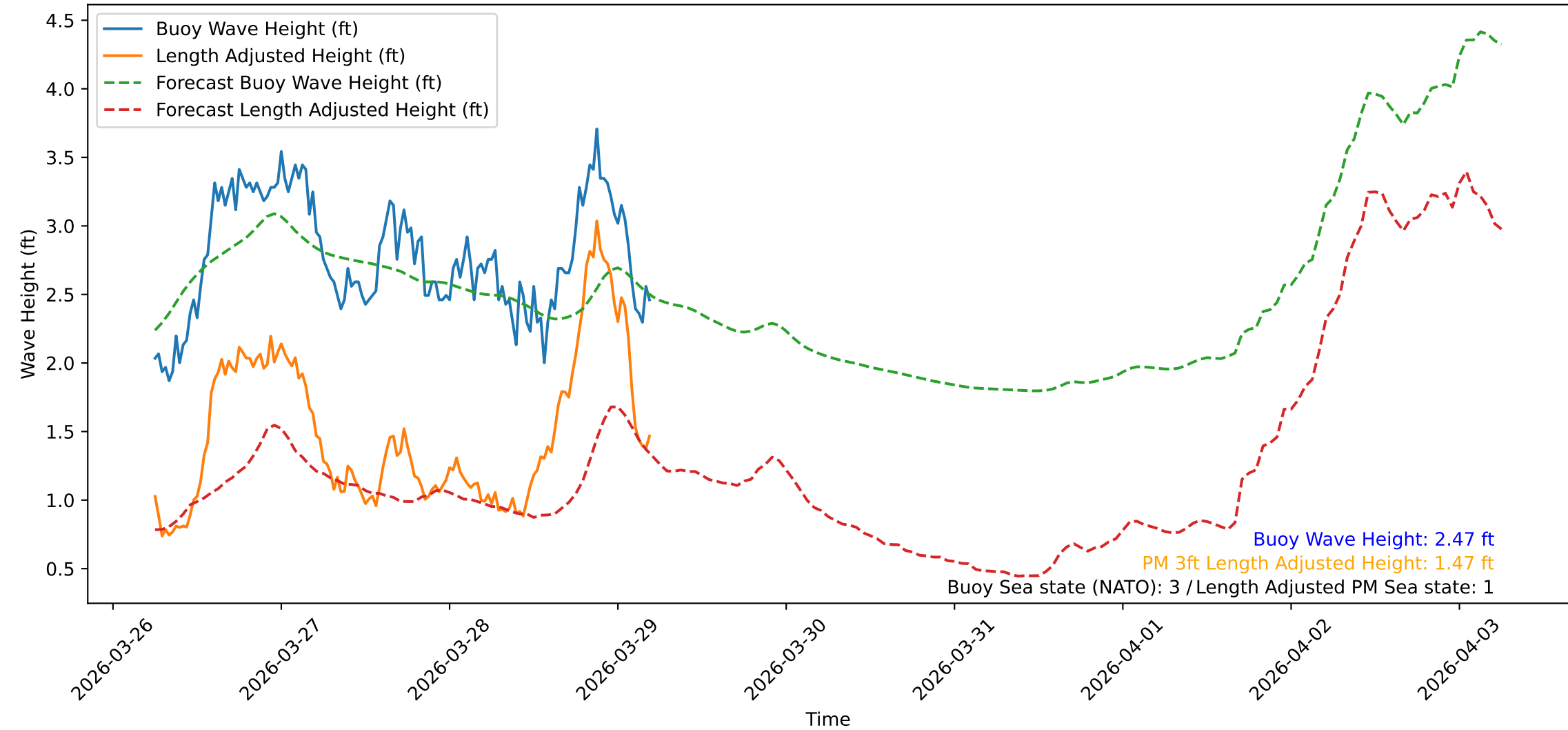
Wave Heights over Time for Green Beach at 2026-03-29 06:01:09
