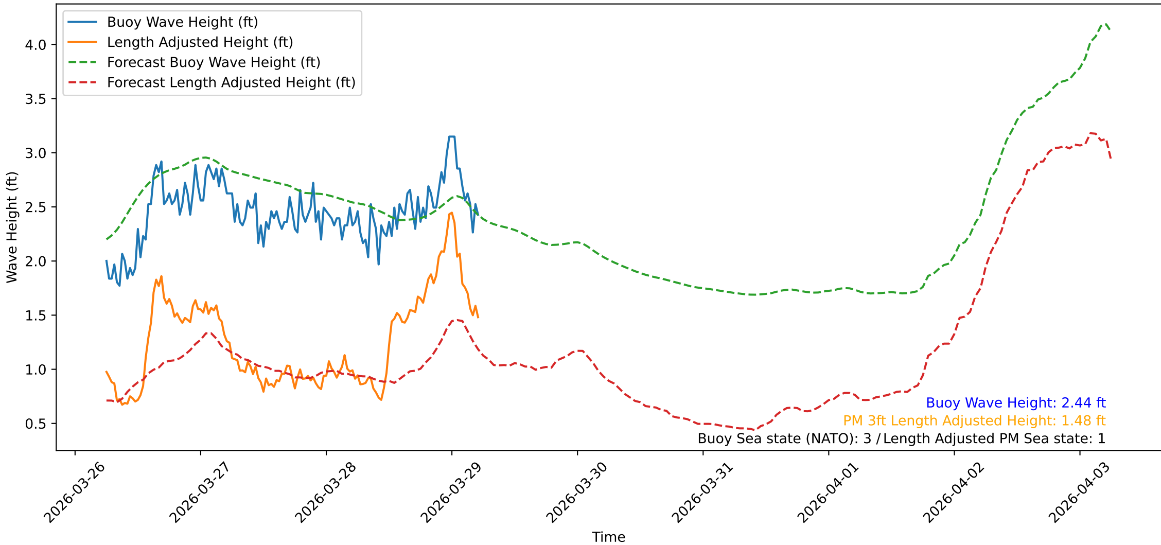
Wave Heights over Time for Oceanside Harbor at 2026-03-29 06:00:31
