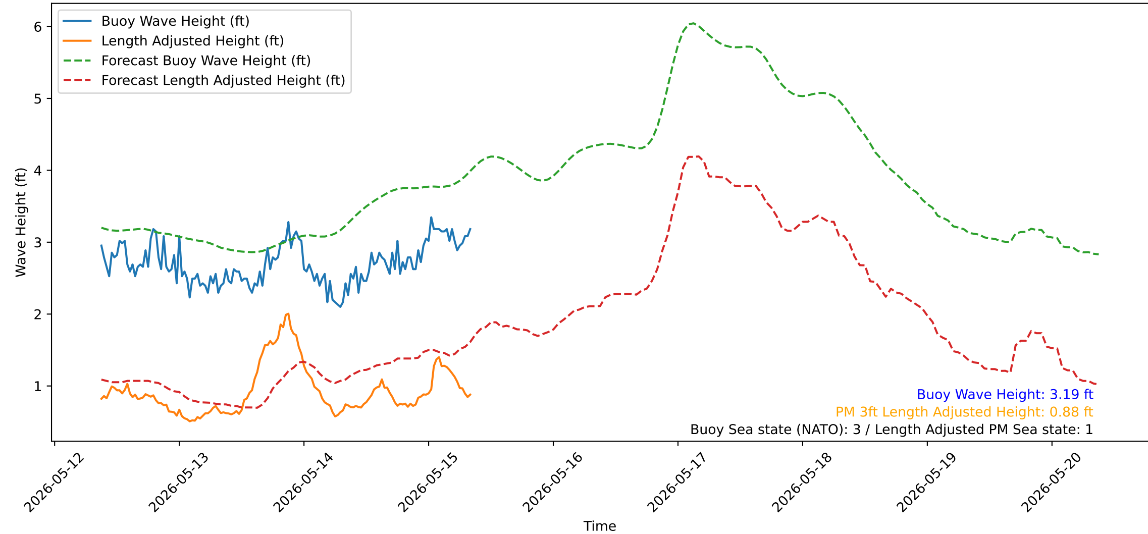
Wave Heights over Time for Green Beach at 2026-05-15 09:01:13
