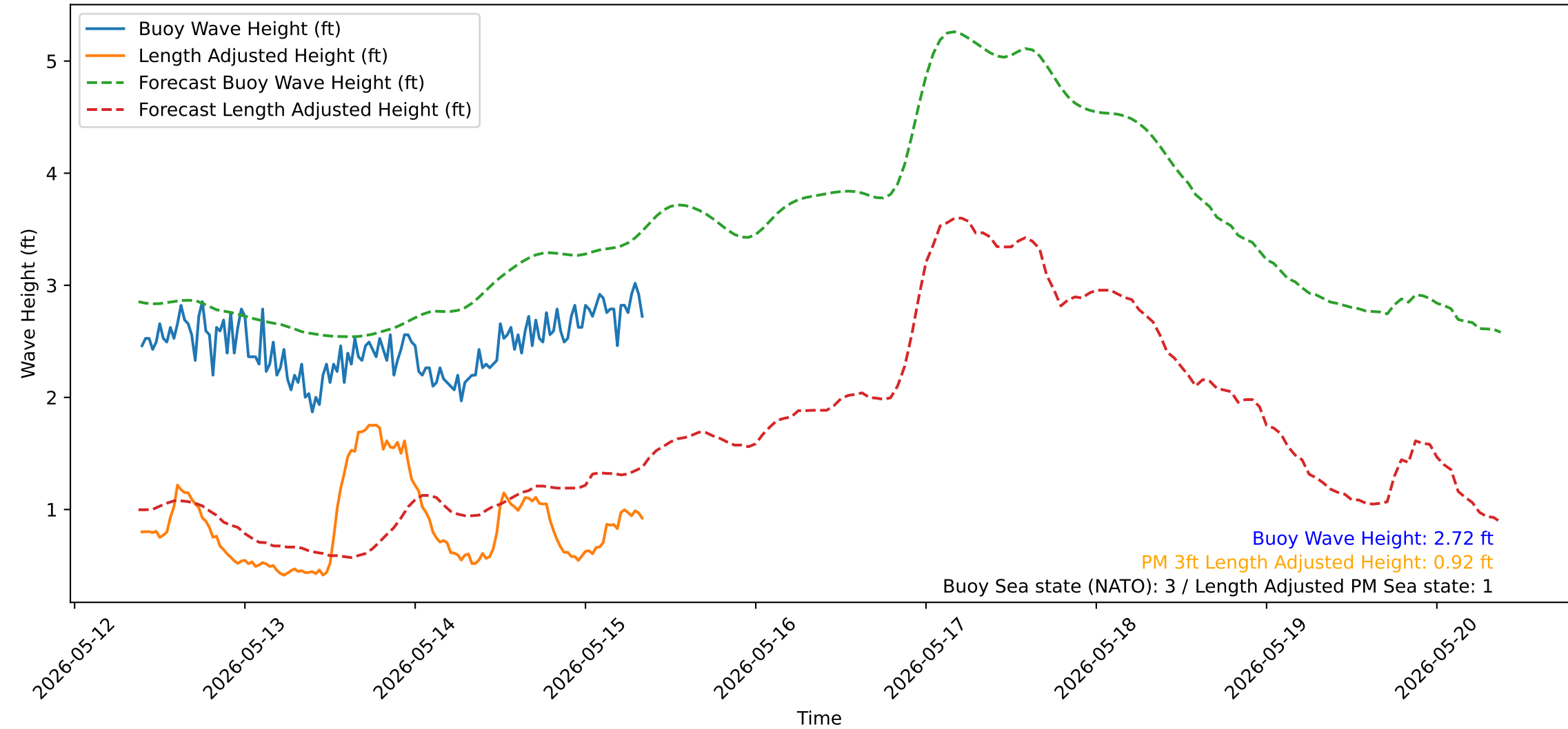
Wave Heights over Time for Red Beach at 2026-05-15 09:00:51
