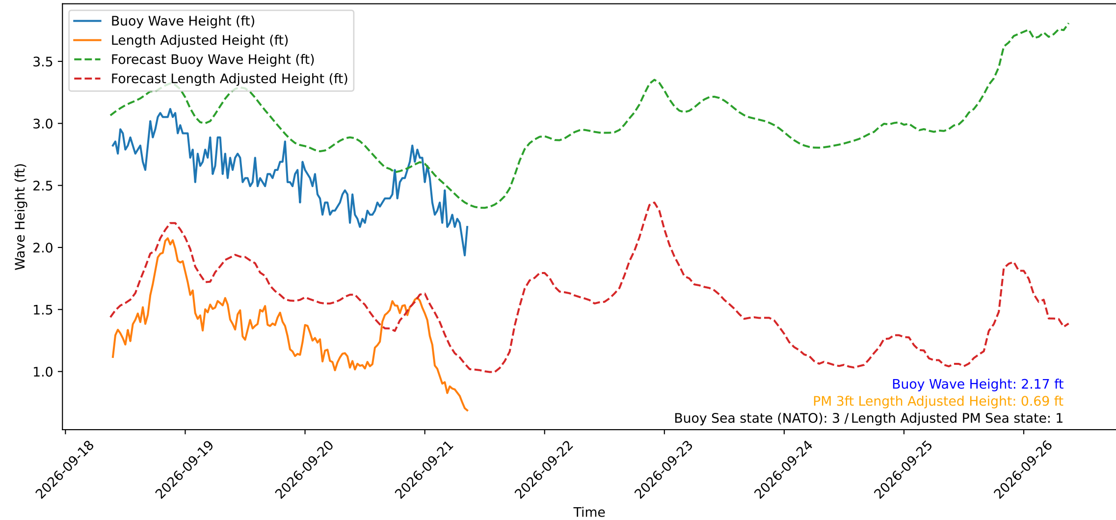
Wave Heights over Time for Green Beach at 2026-09-21 09:21:14
