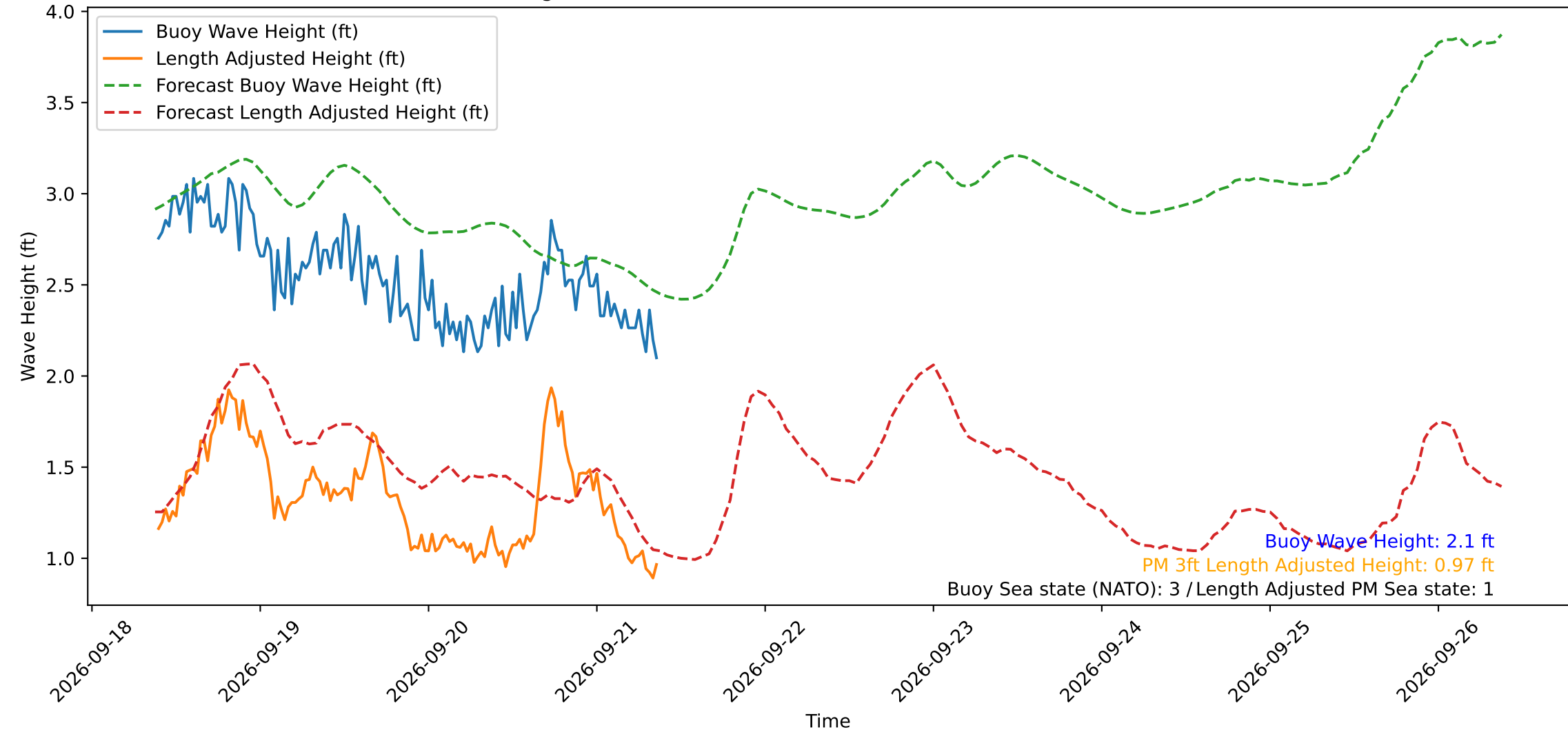
Wave Heights over Time for Oceanside Harbor at 2026-09-21 09:20:30
