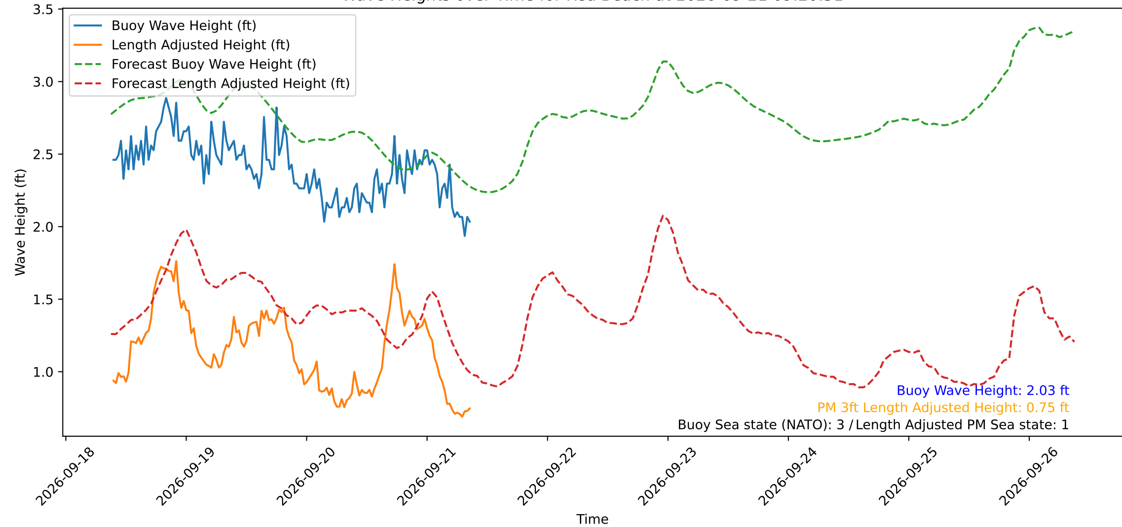
Wave Heights over Time for Red Beach at 2026-09-21 09:20:51
