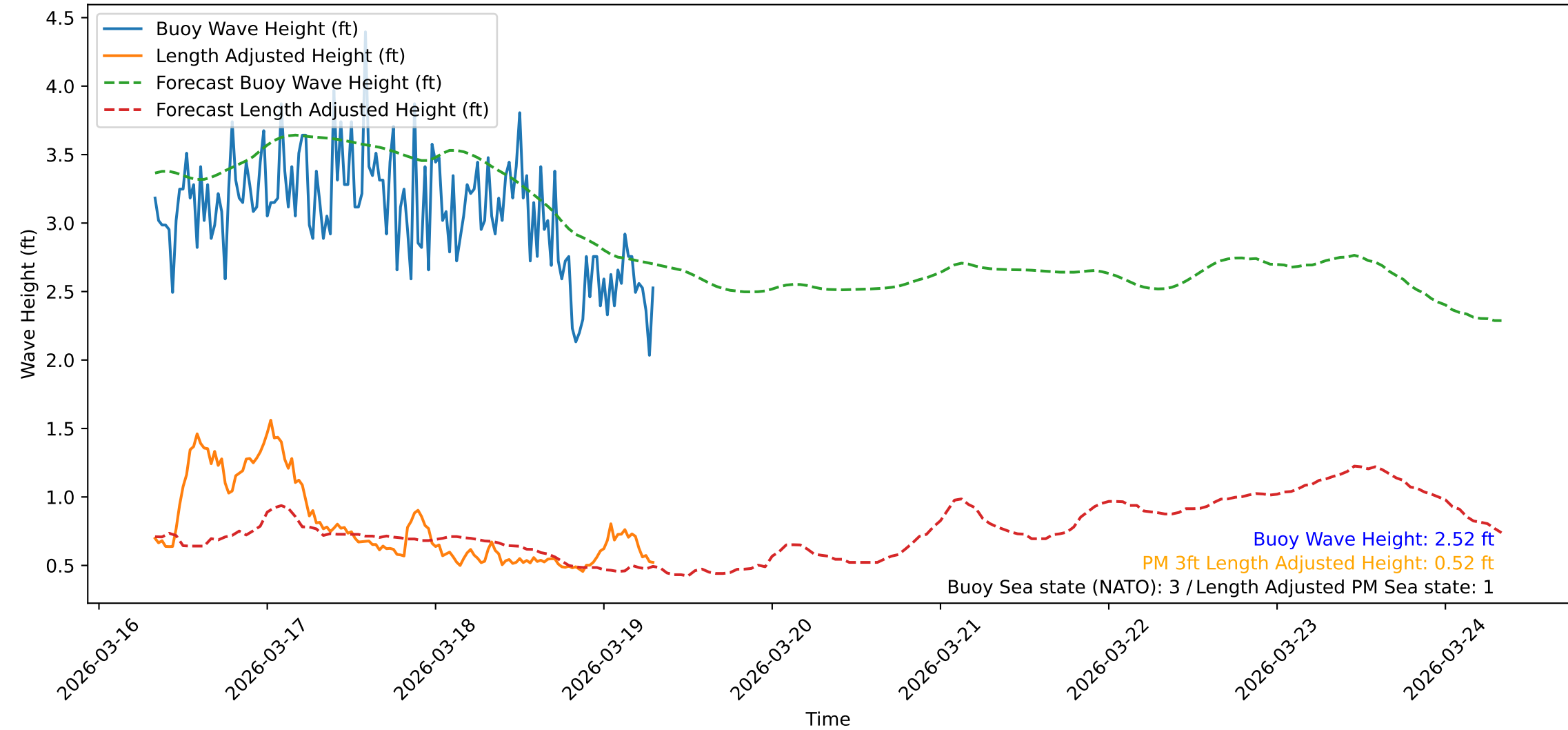
Wave Heights over Time for Oceanside Harbor at 2026-03-19 08:00:31
