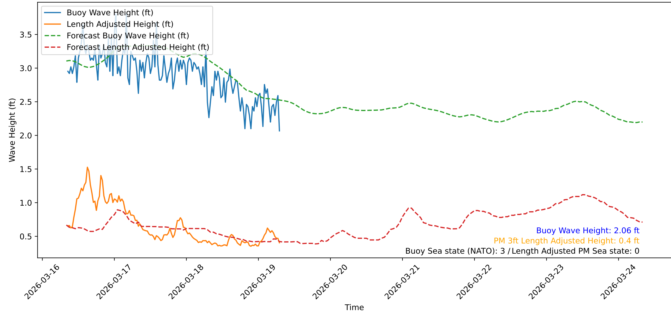
Wave Heights over Time for Red Beach at 2026-03-19 08:00:47
