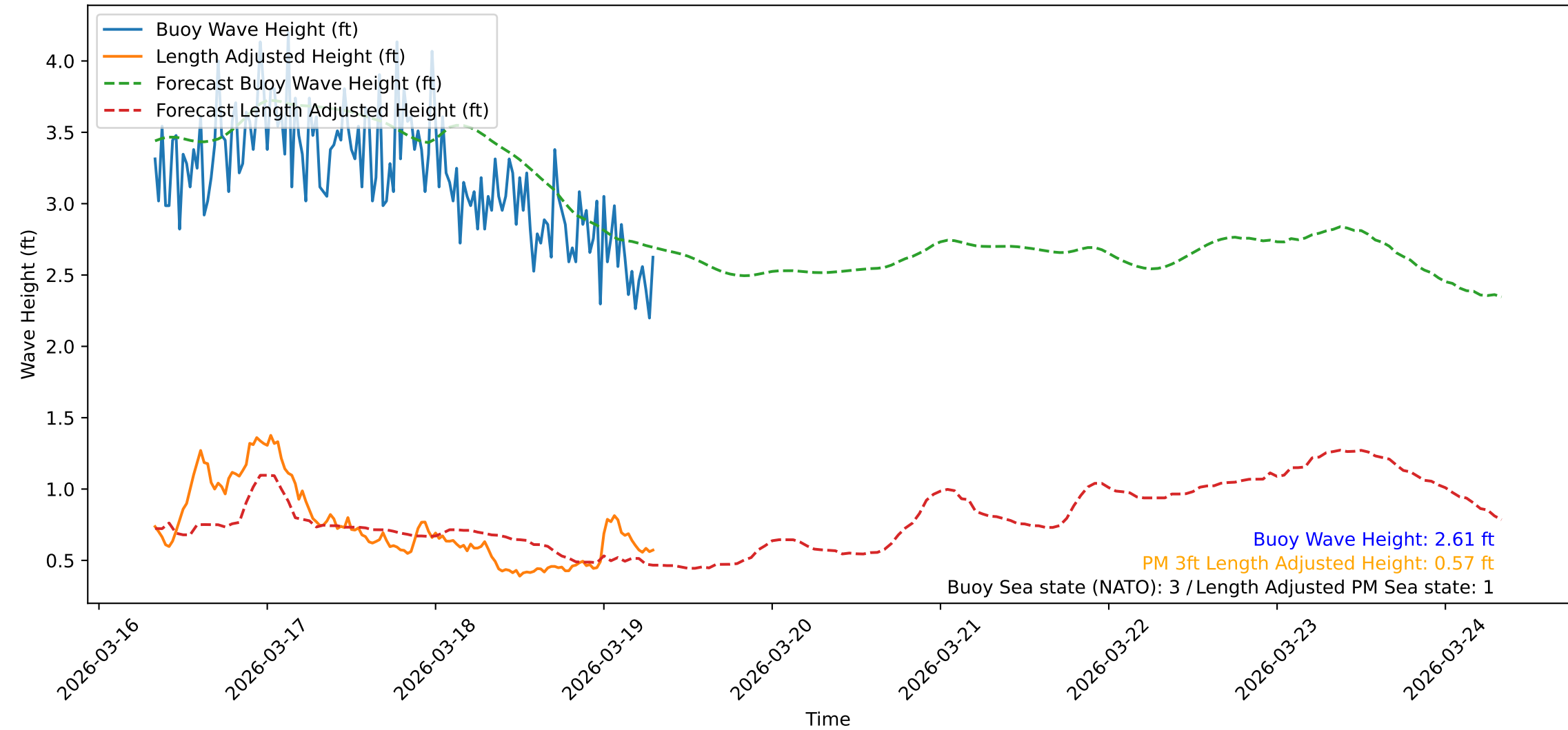
Wave Heights over Time for Green Beach at 2026-03-19 08:01:10
