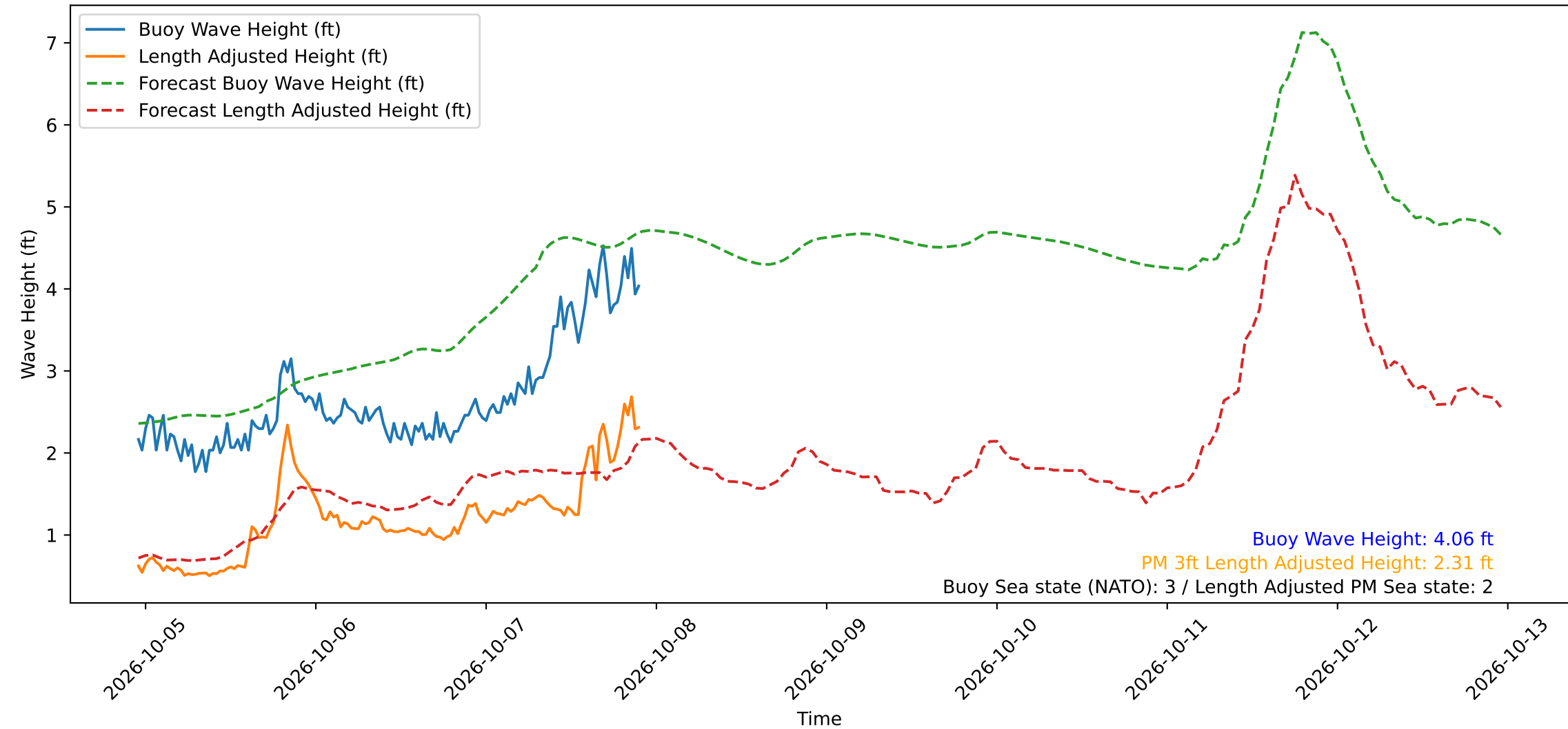
Wave Heights over Time for Green Beach at 2026-10-07 22:31:12
