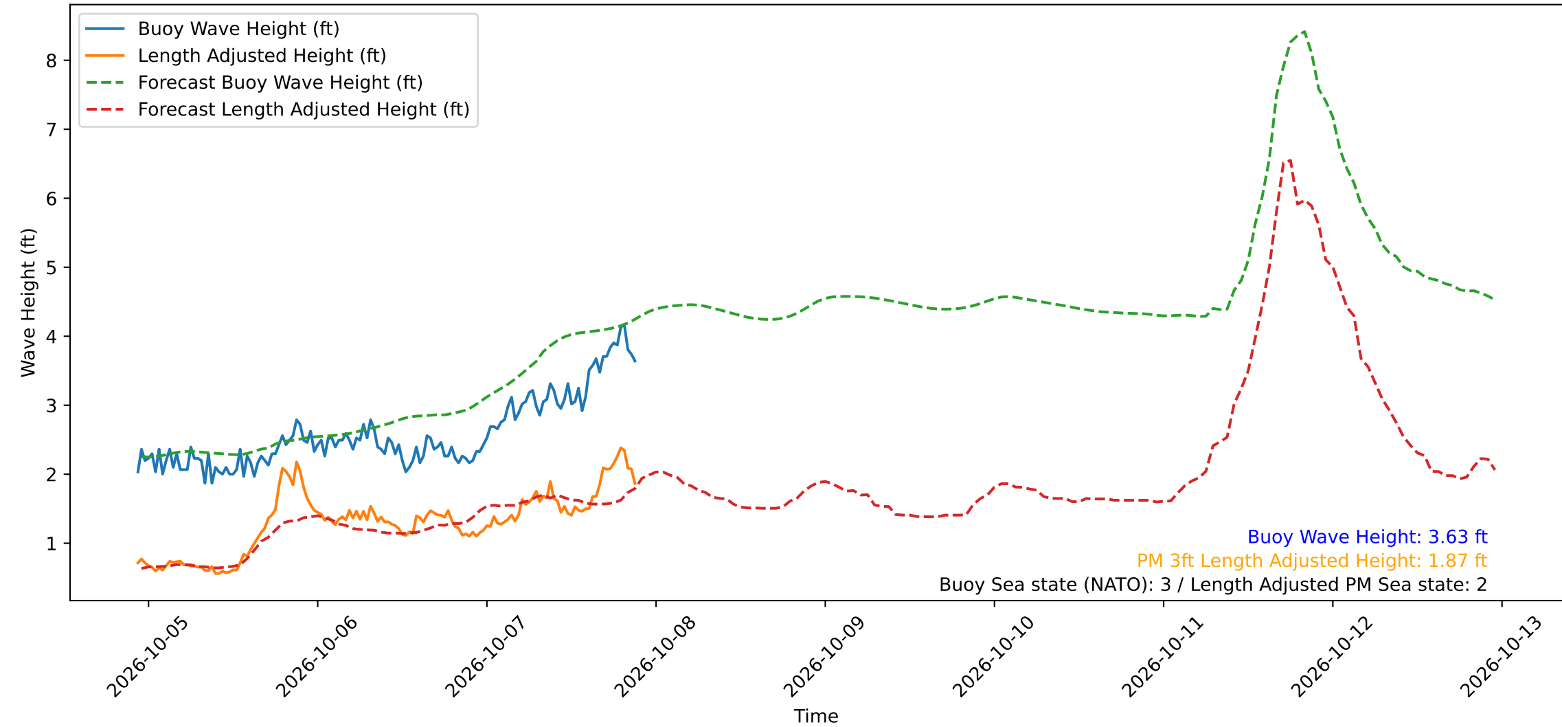
Wave Heights over Time for Oceanside Harbor at 2026-10-07 22:30:29
