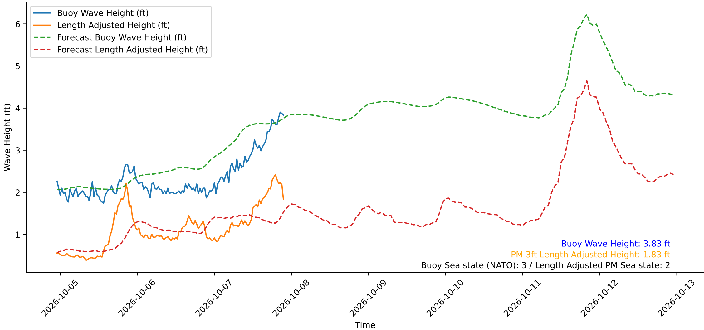
Wave Heights over Time for Red Beach at 2026-10-07 22:30:49
