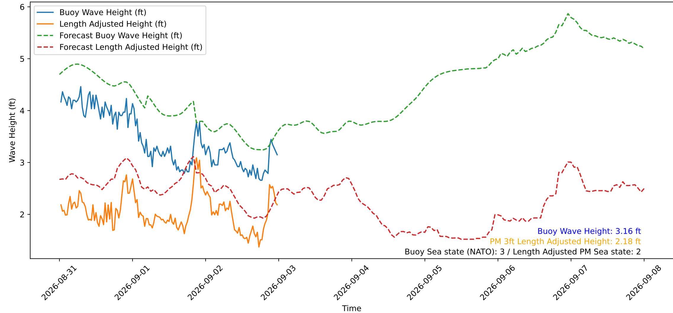
Wave Heights over Time for Green Beach at 2026-09-03 00:11:11
