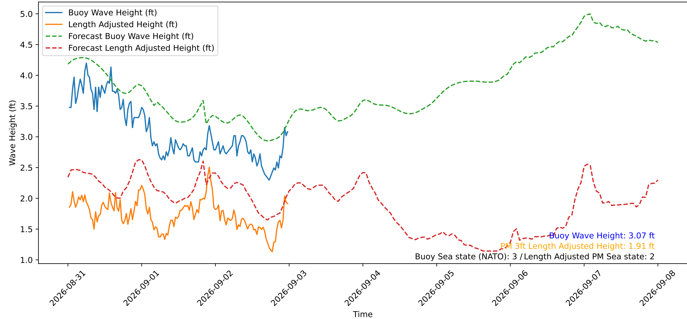
Wave Heights over Time for Red Beach at 2026-09-03 00:10:49
