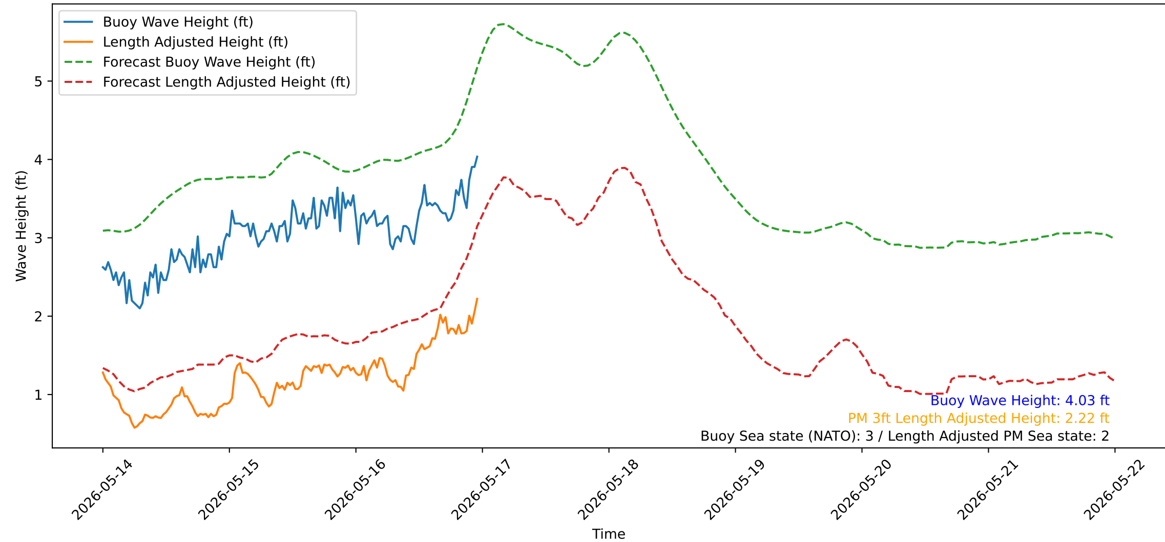
Wave Heights over Time for Green Beach at 2026-05-17 00:01:13
