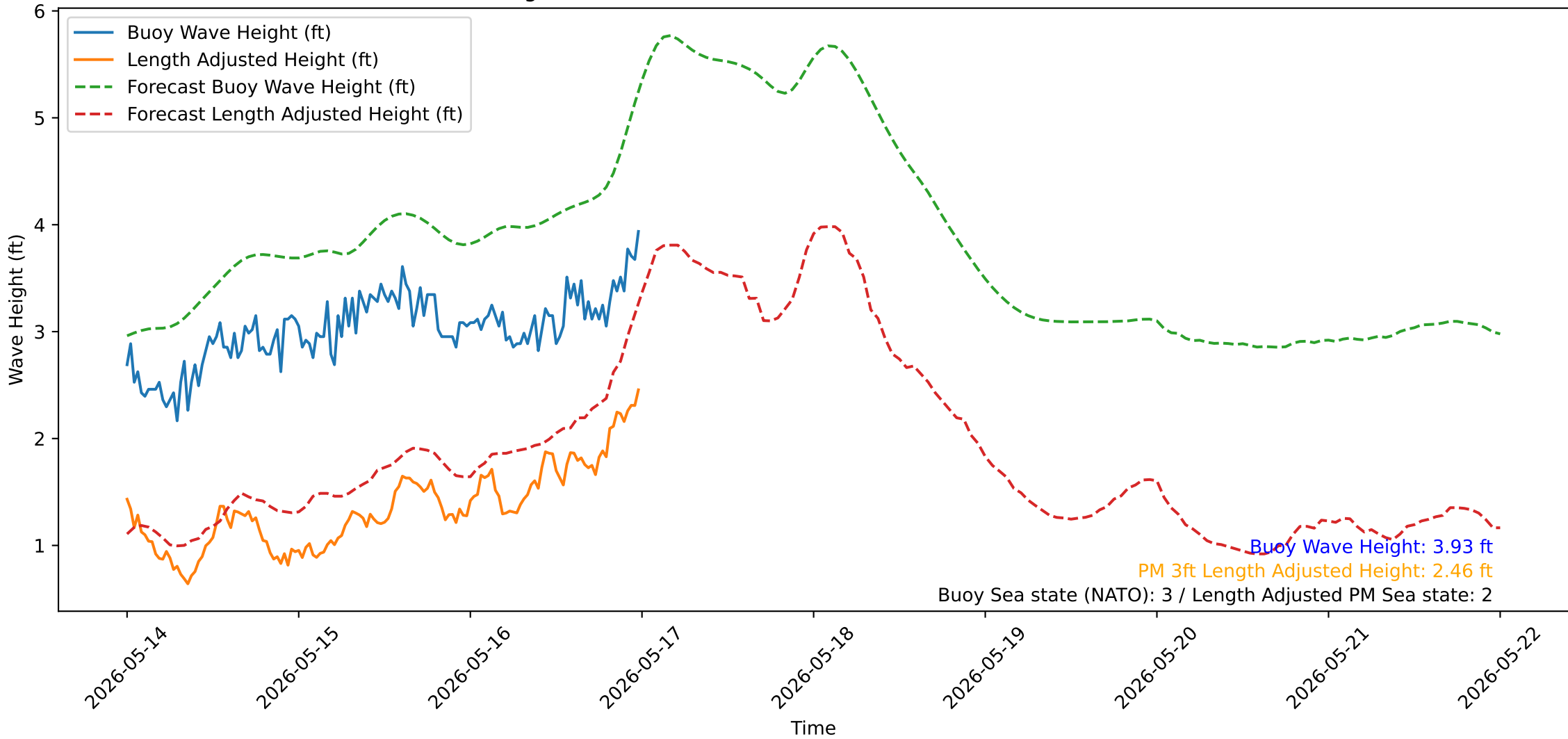
Wave Heights over Time for Oceanside Harbor at 2026-05-17 00:00:32
