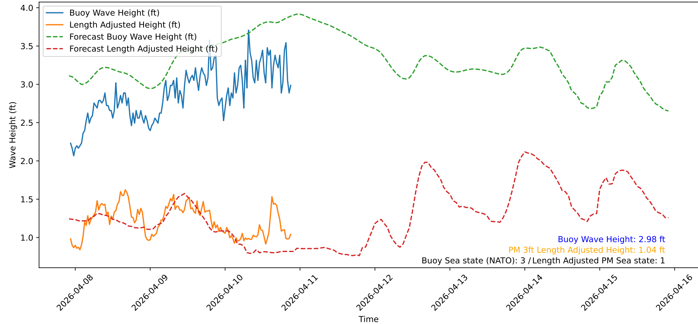
Wave Heights over Time for Red Beach at 2026-04-10 22:00:51
