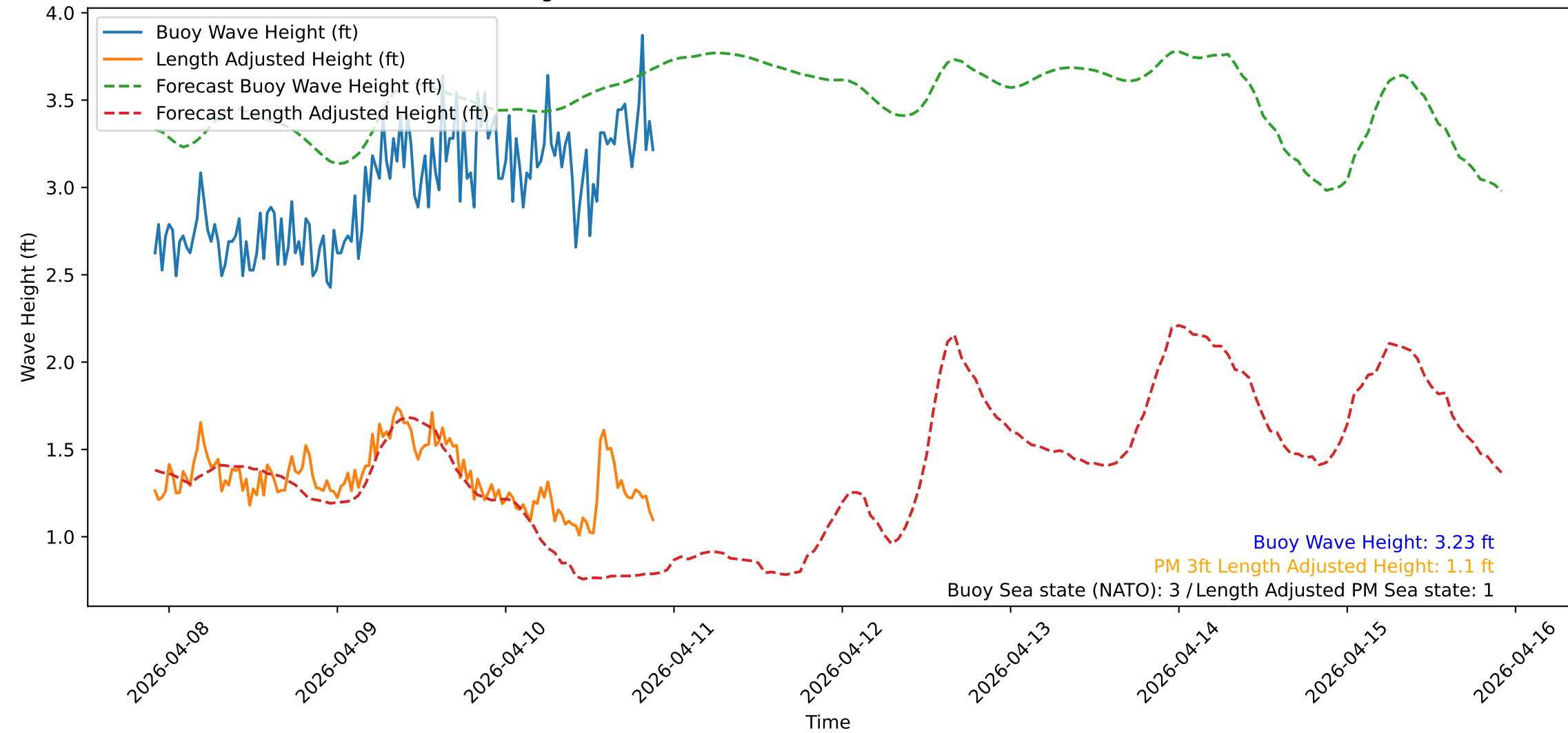
Wave Heights over Time for Oceanside Harbor at 2026-04-10 22:00:32
