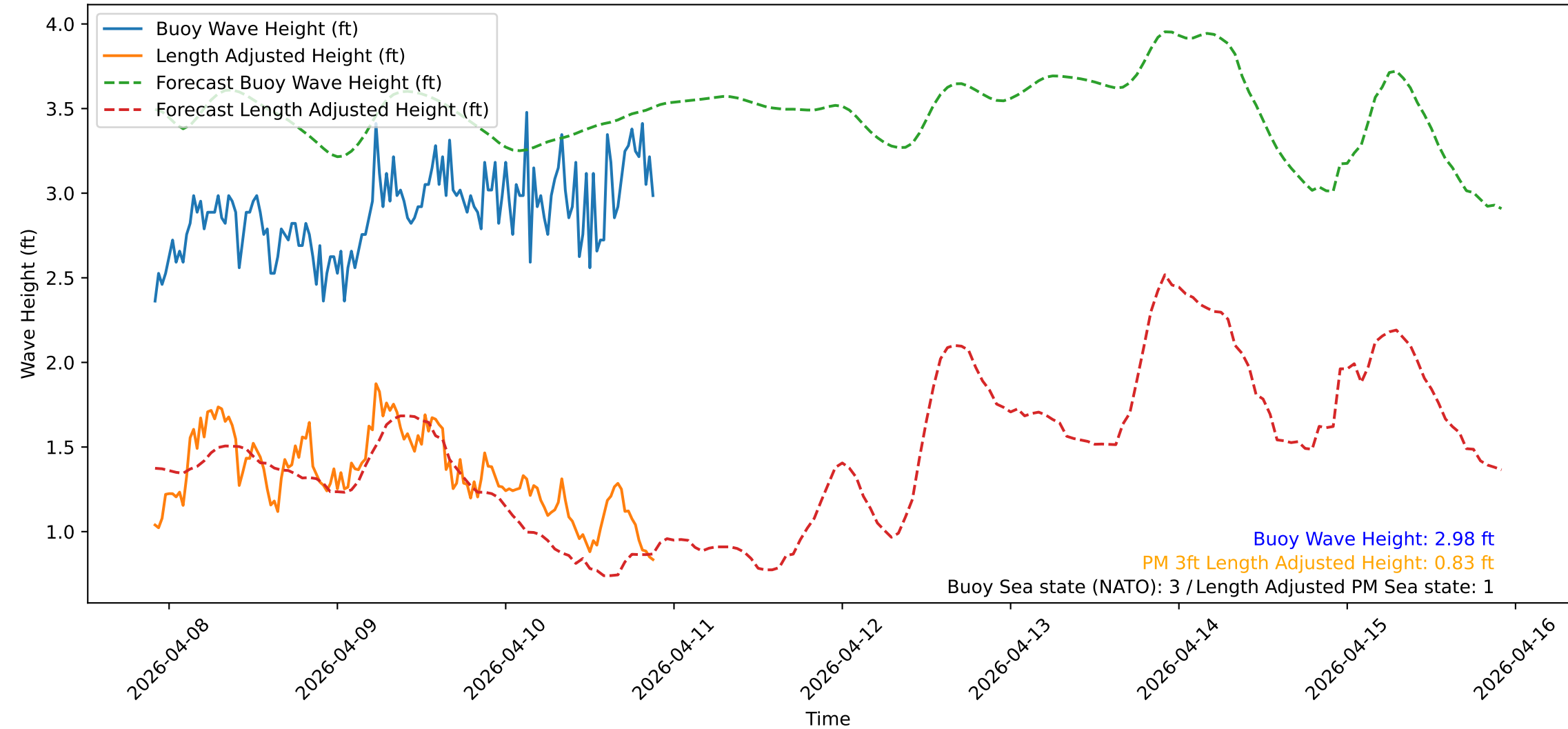
Wave Heights over Time for Green Beach at 2026-04-10 22:01:13
