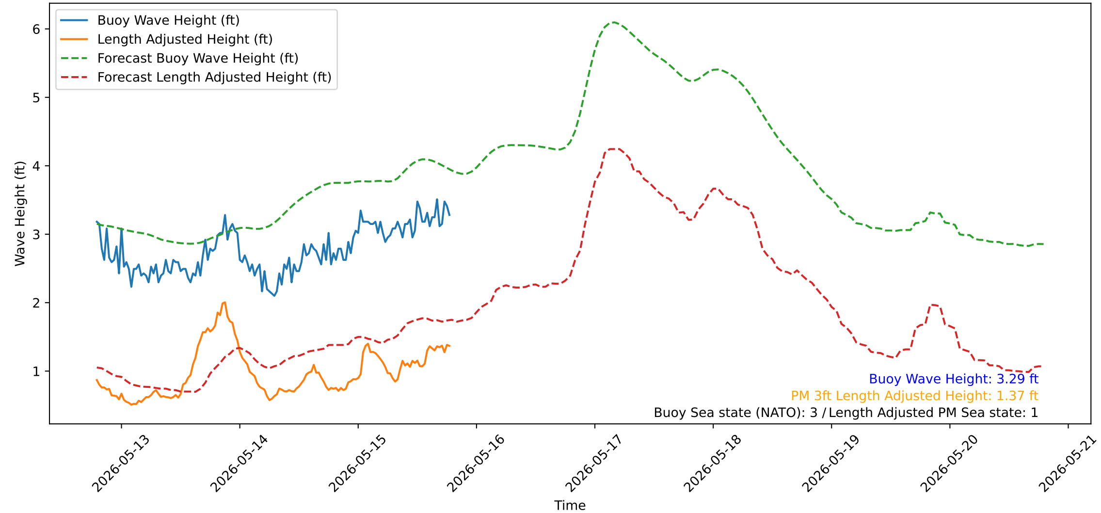
Wave Heights over Time for Green Beach at 2026-05-15 19:11:14
