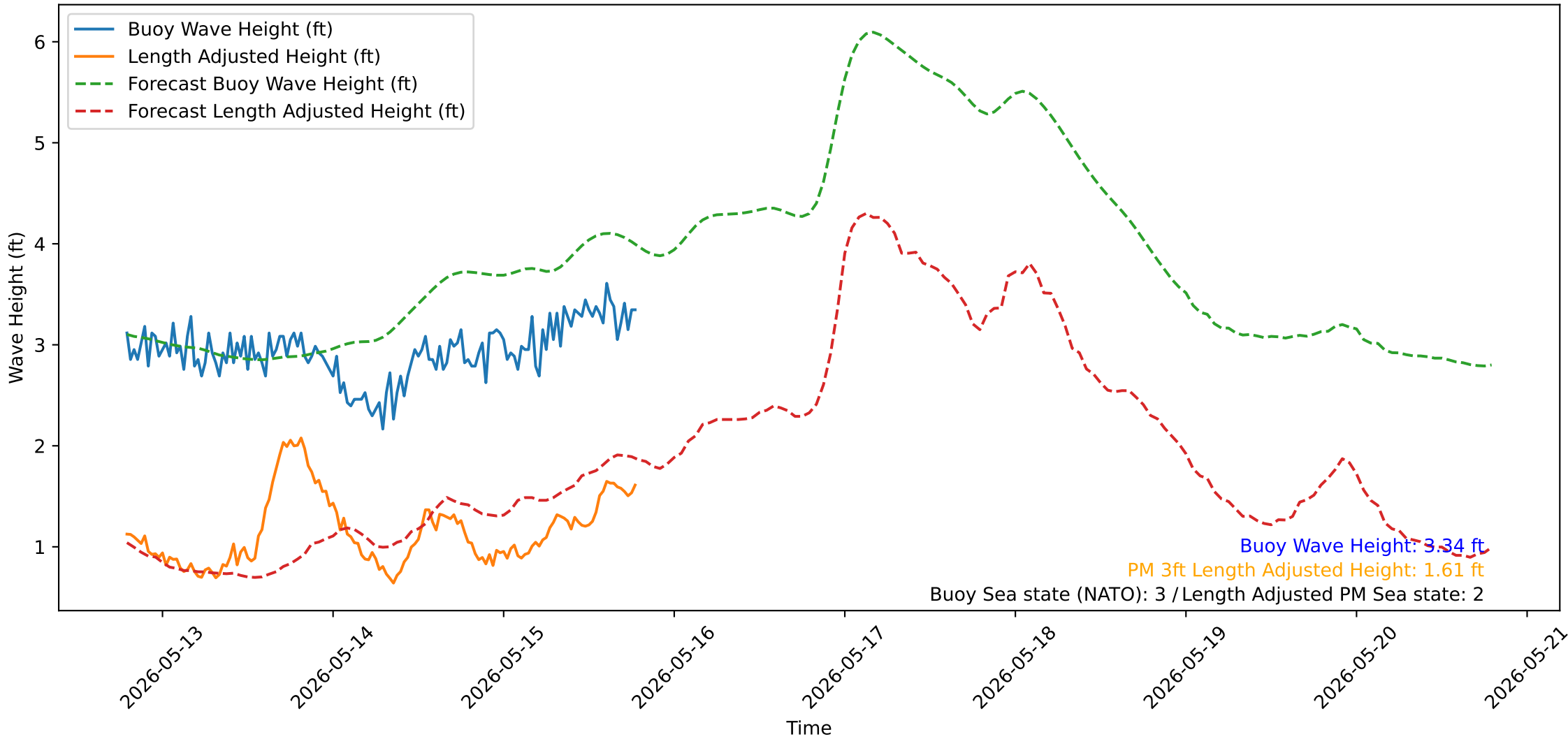
Wave Heights over Time for Oceanside Harbor at 2026-05-15 19:10:32
