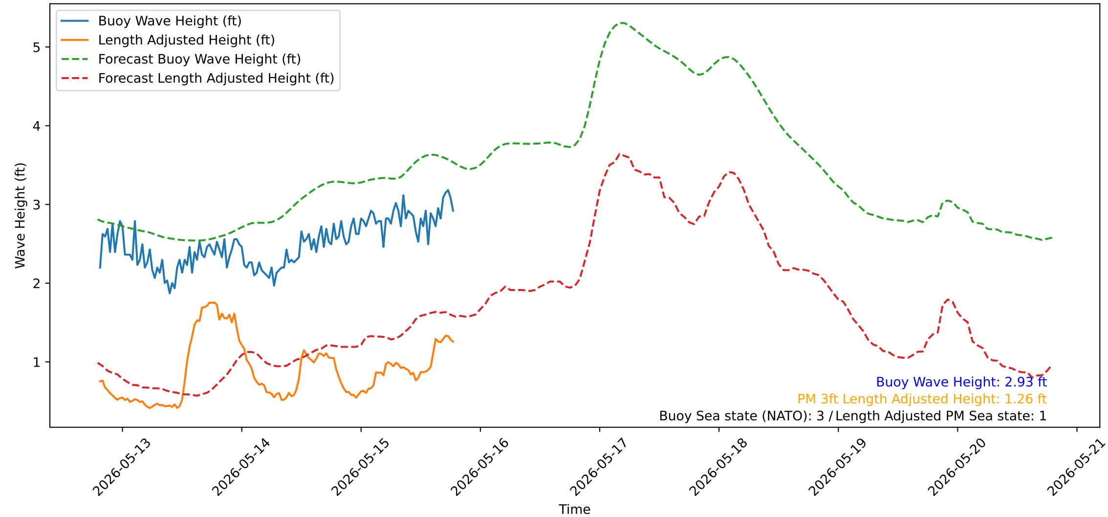
Wave Heights over Time for Red Beach at 2026-05-15 19:10:51
