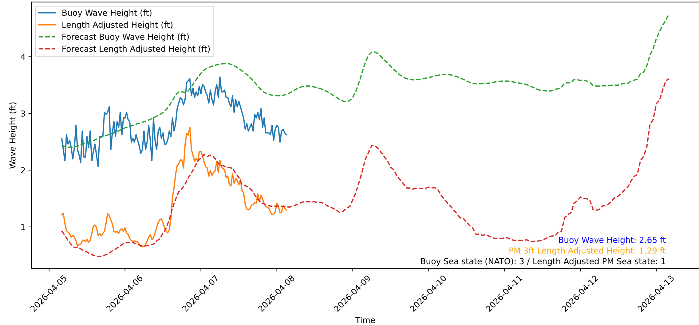
Wave Heights over Time for Oceanside Harbor at 2026-04-08 03:50:31
