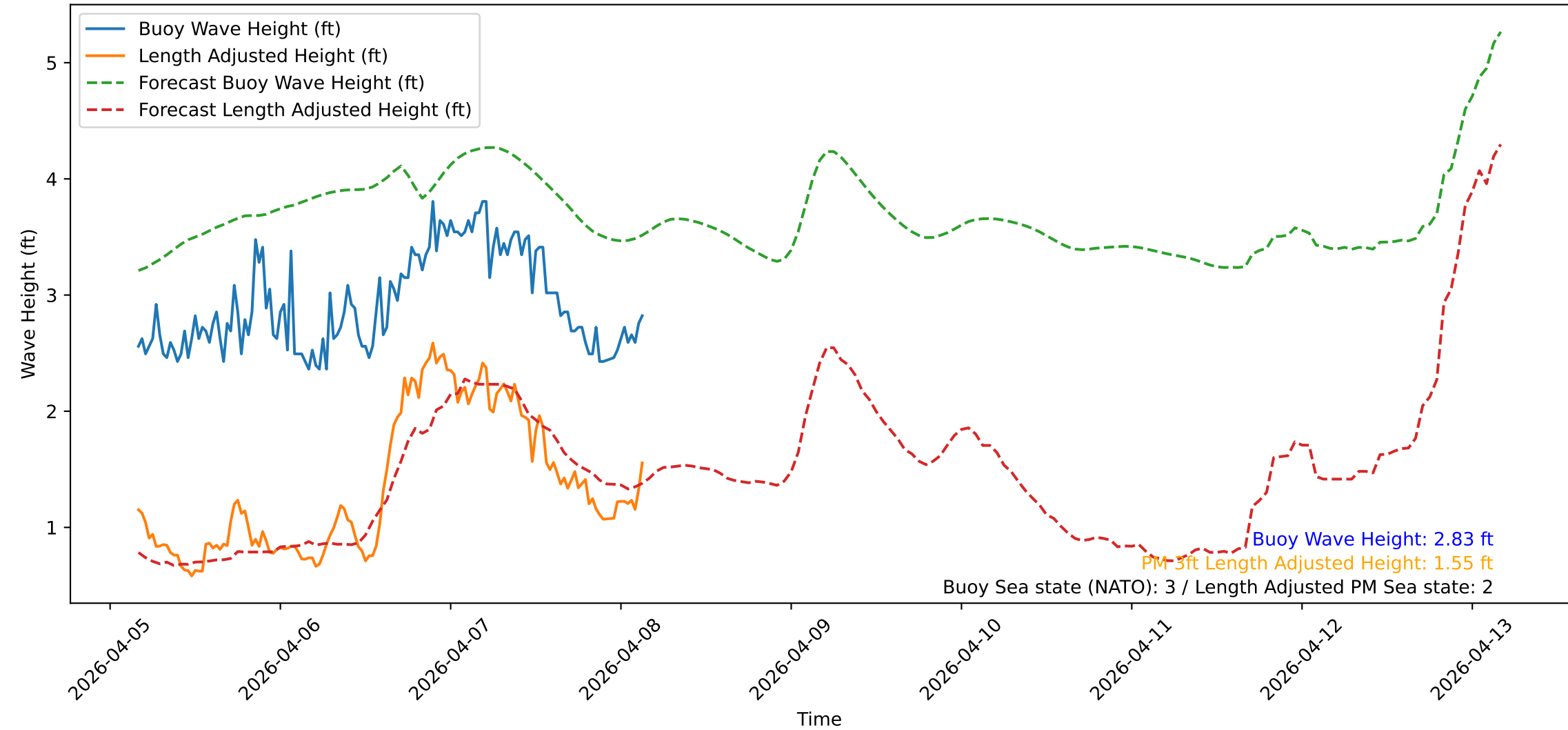
Wave Heights over Time for Green Beach at 2026-04-08 03:51:10
