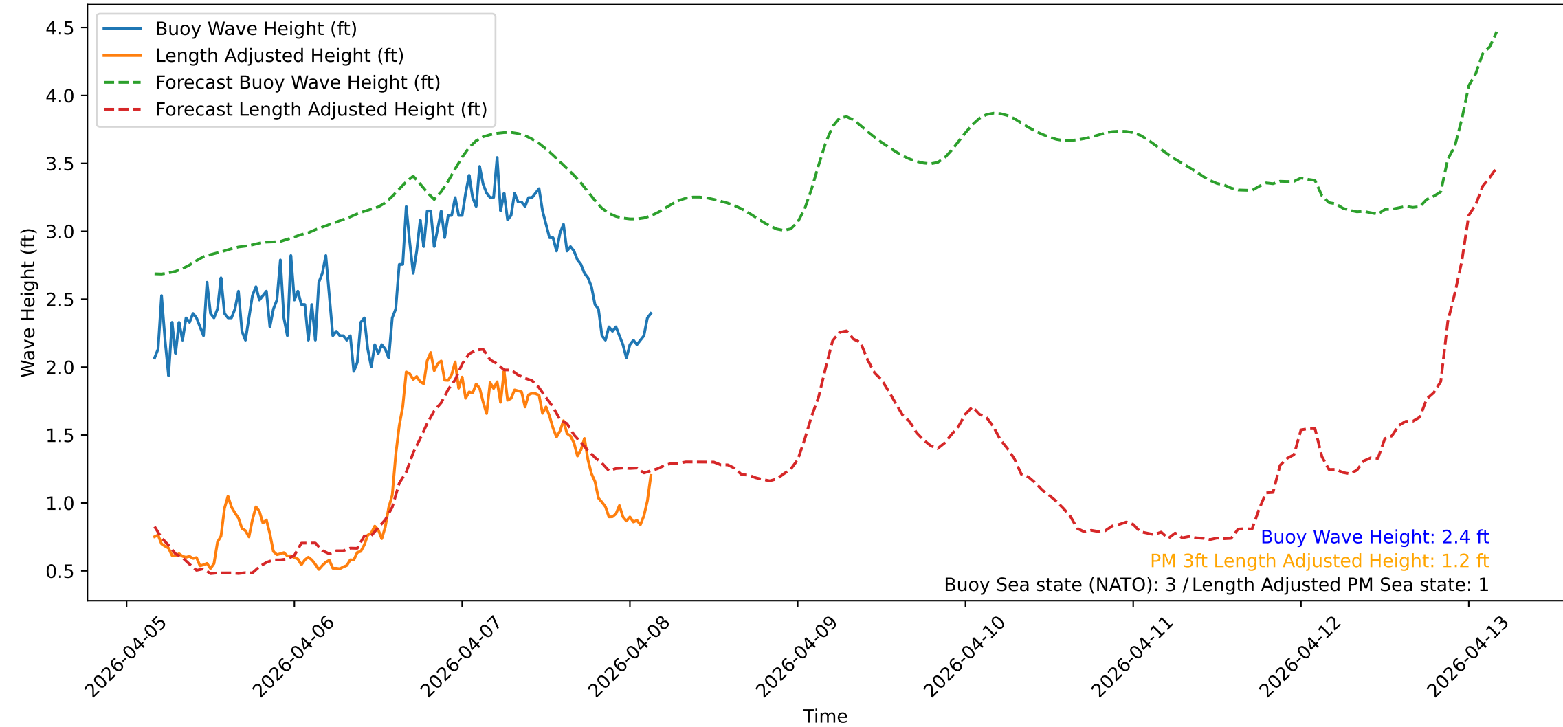
Wave Heights over Time for Red Beach at 2026-04-08 03:50:47
