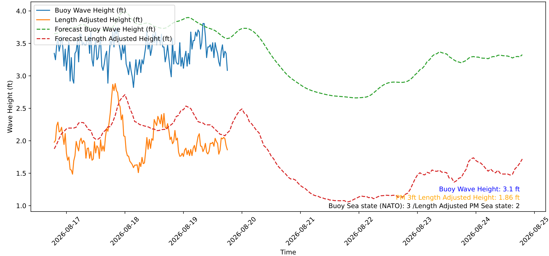
Wave Heights over Time for Oceanside Harbor at 2026-08-19 18:50:26
