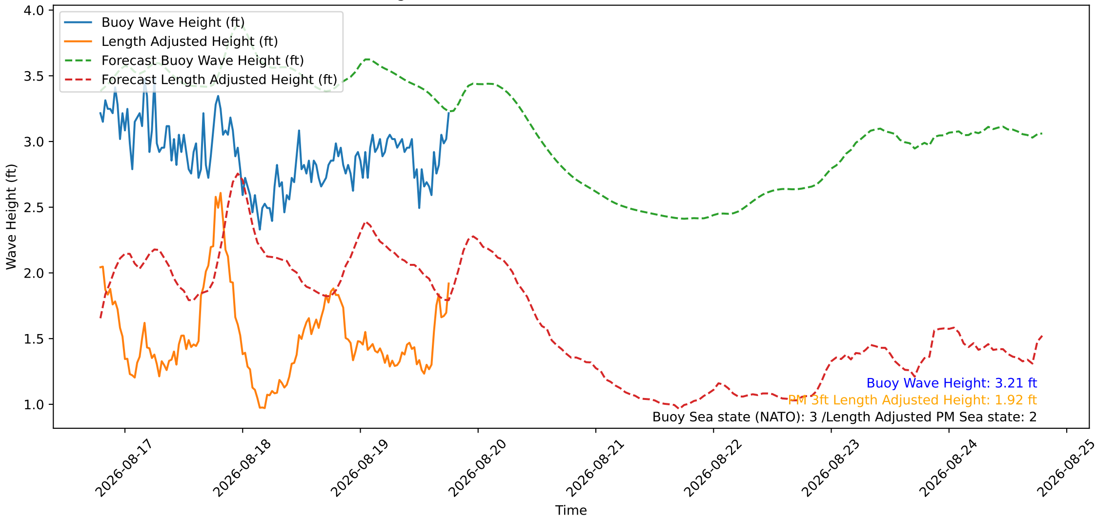
Wave Heights over Time for Red Beach at 2026-08-19 18:50:47
