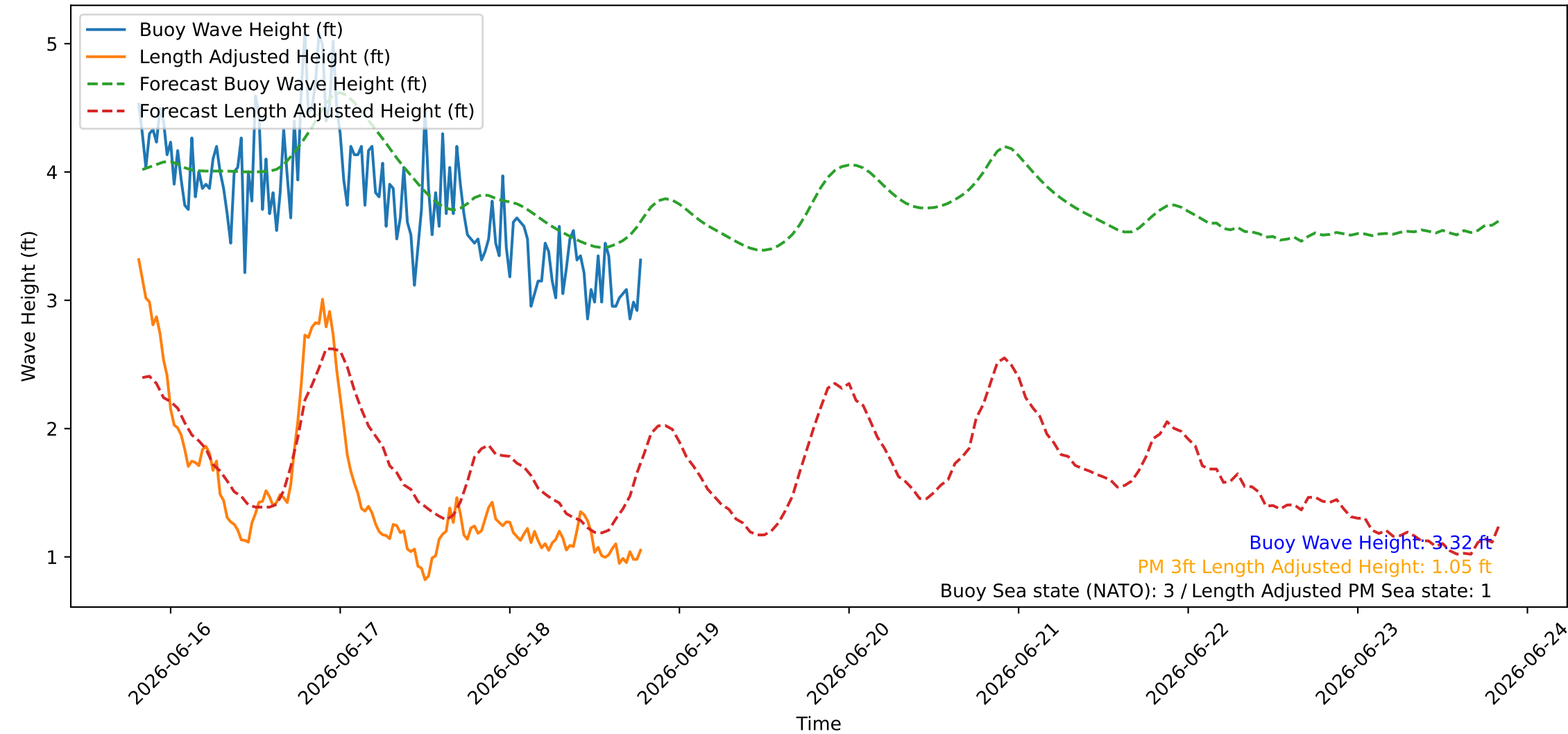
Wave Heights over Time for Green Beach at 2026-06-18 19:31:08
