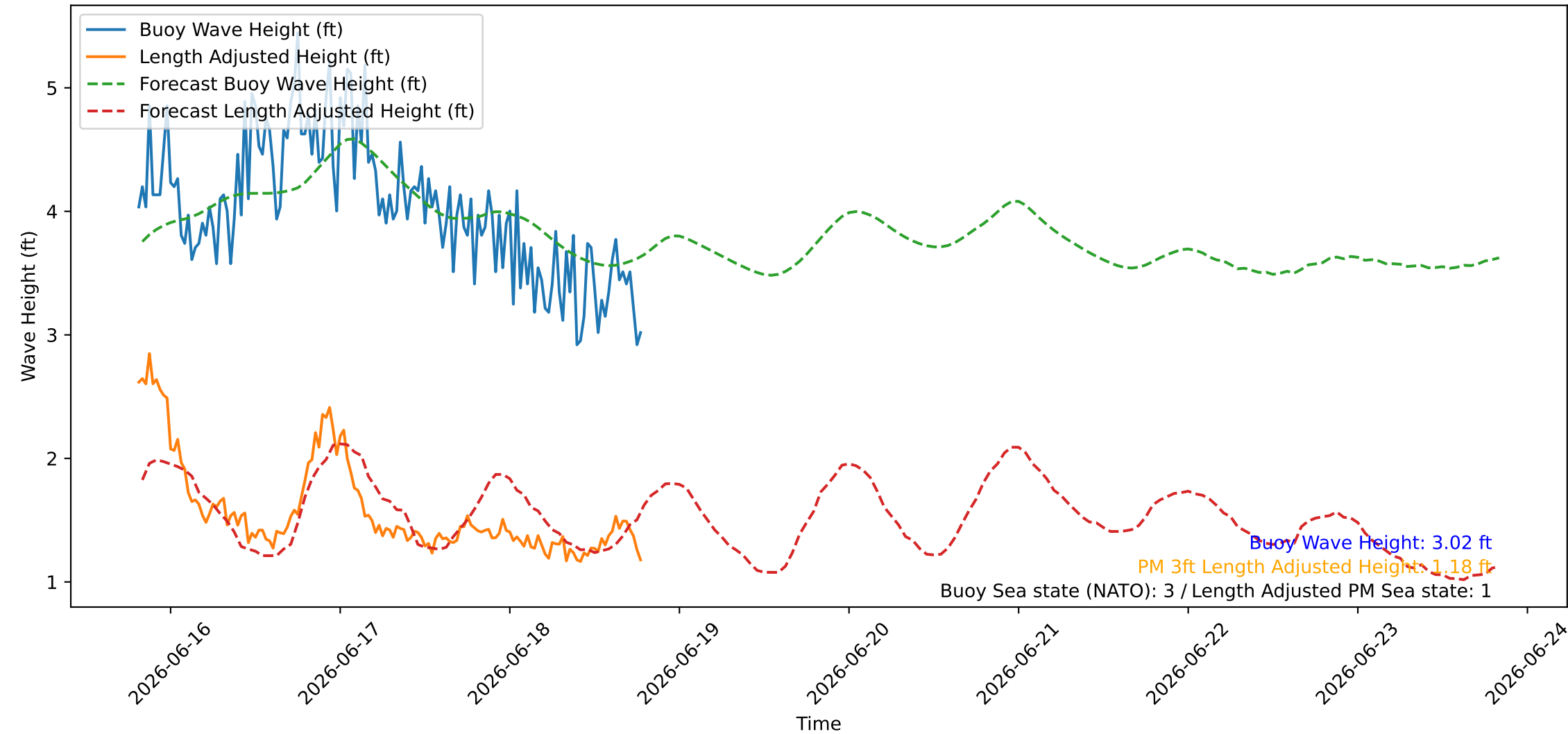
Wave Heights over Time for Oceanside Harbor at 2026-06-18 19:30:26
