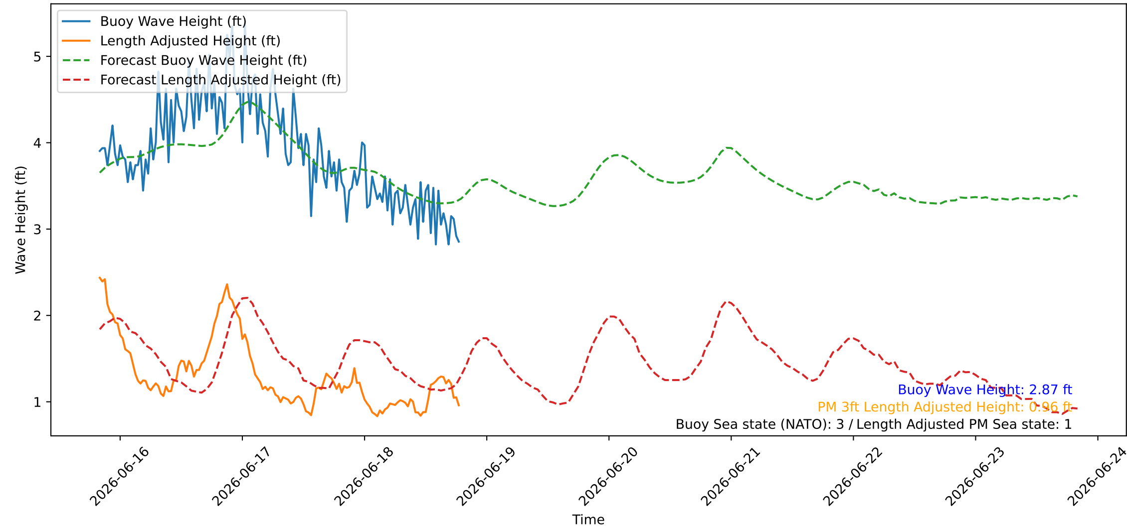
Wave Heights over Time for Red Beach at 2026-06-18 19:30:46
