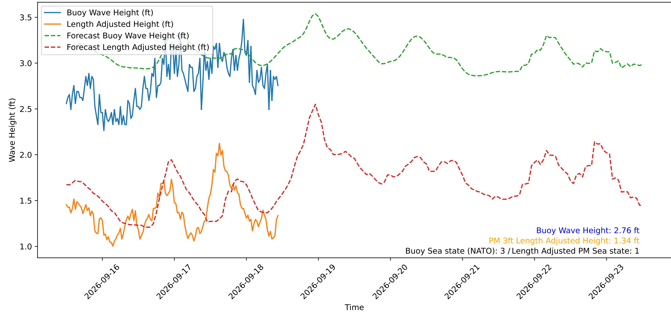
Wave Heights over Time for Green Beach at 2026-09-18 11:31:11
