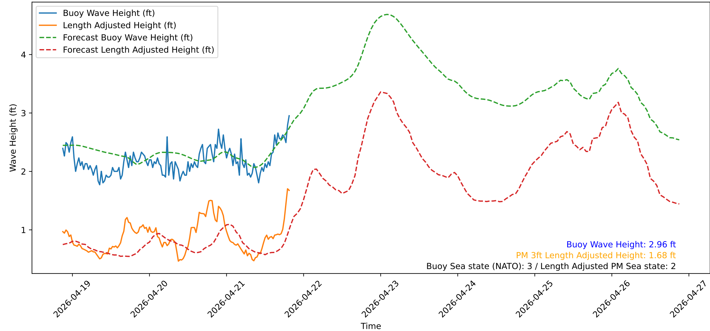
Wave Heights over Time for Red Beach at 2026-04-21 20:30:50
