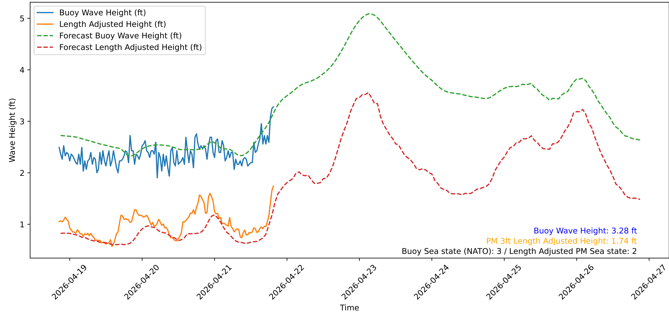
Wave Heights over Time for Oceanside Harbor at 2026-04-21 20:30:31
