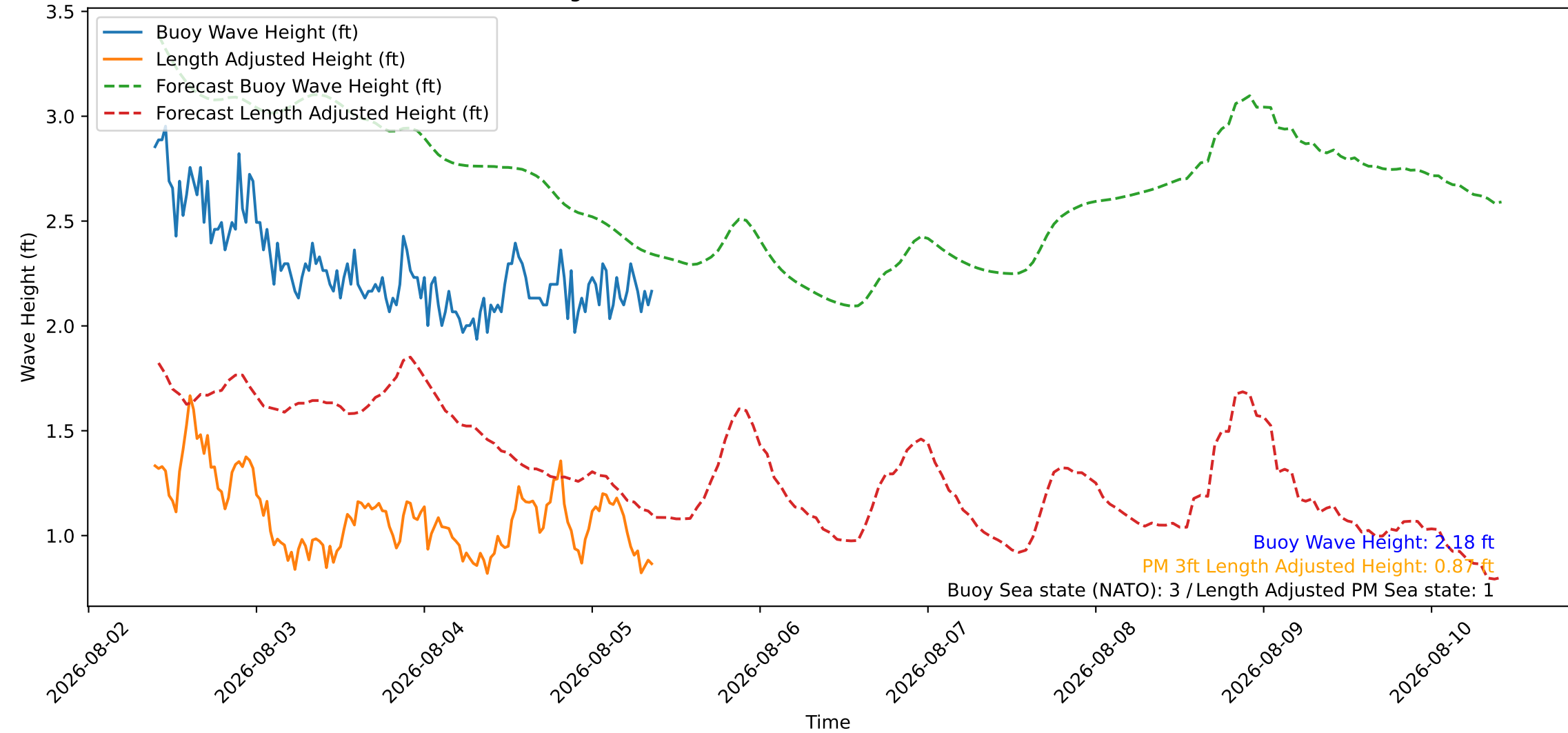
Wave Heights over Time for Green Beach at 2026-08-05 09:31:08
