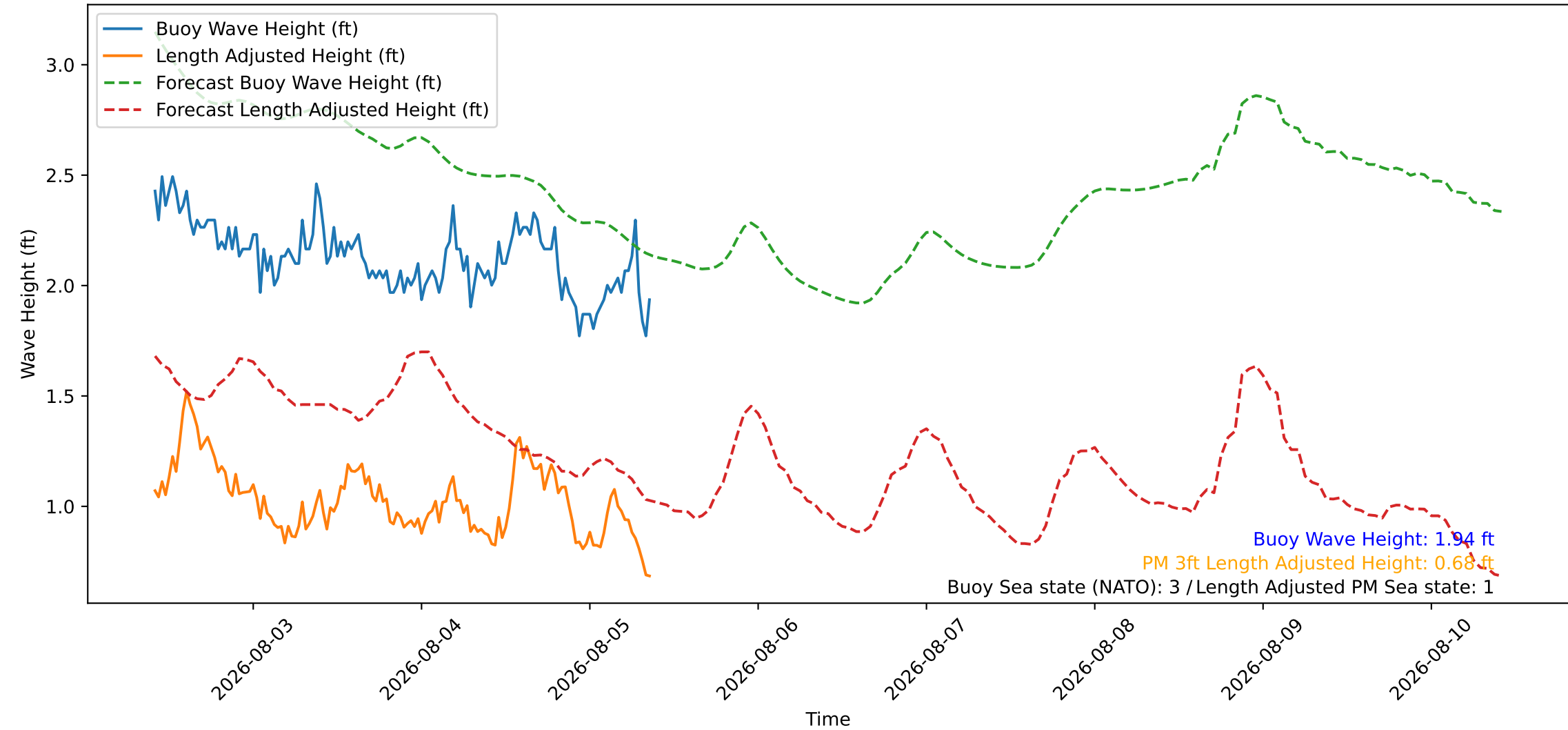
Wave Heights over Time for Red Beach at 2026-08-05 09:30:46
