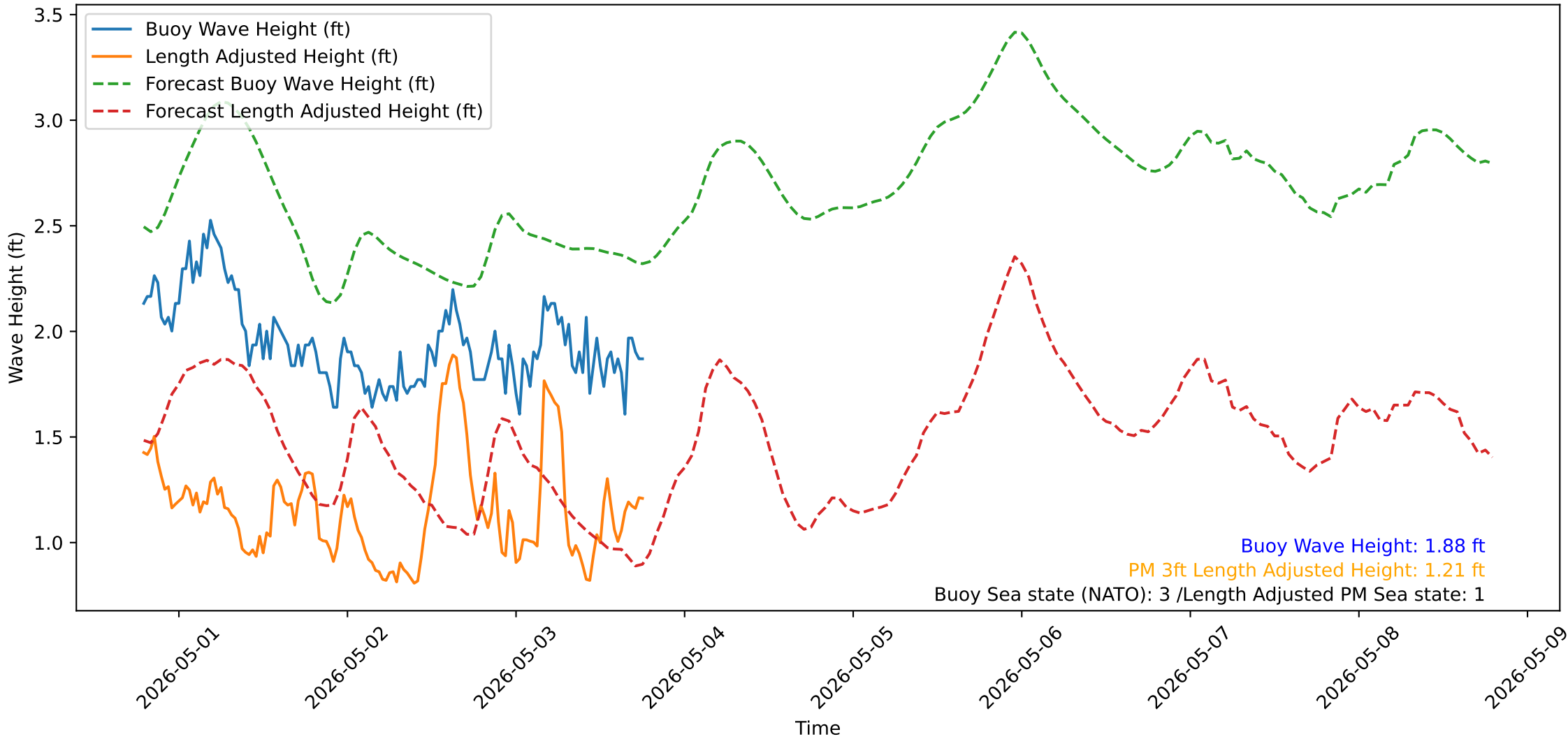
Wave Heights over Time for Red Beach at 2026-05-03 18:40:51
