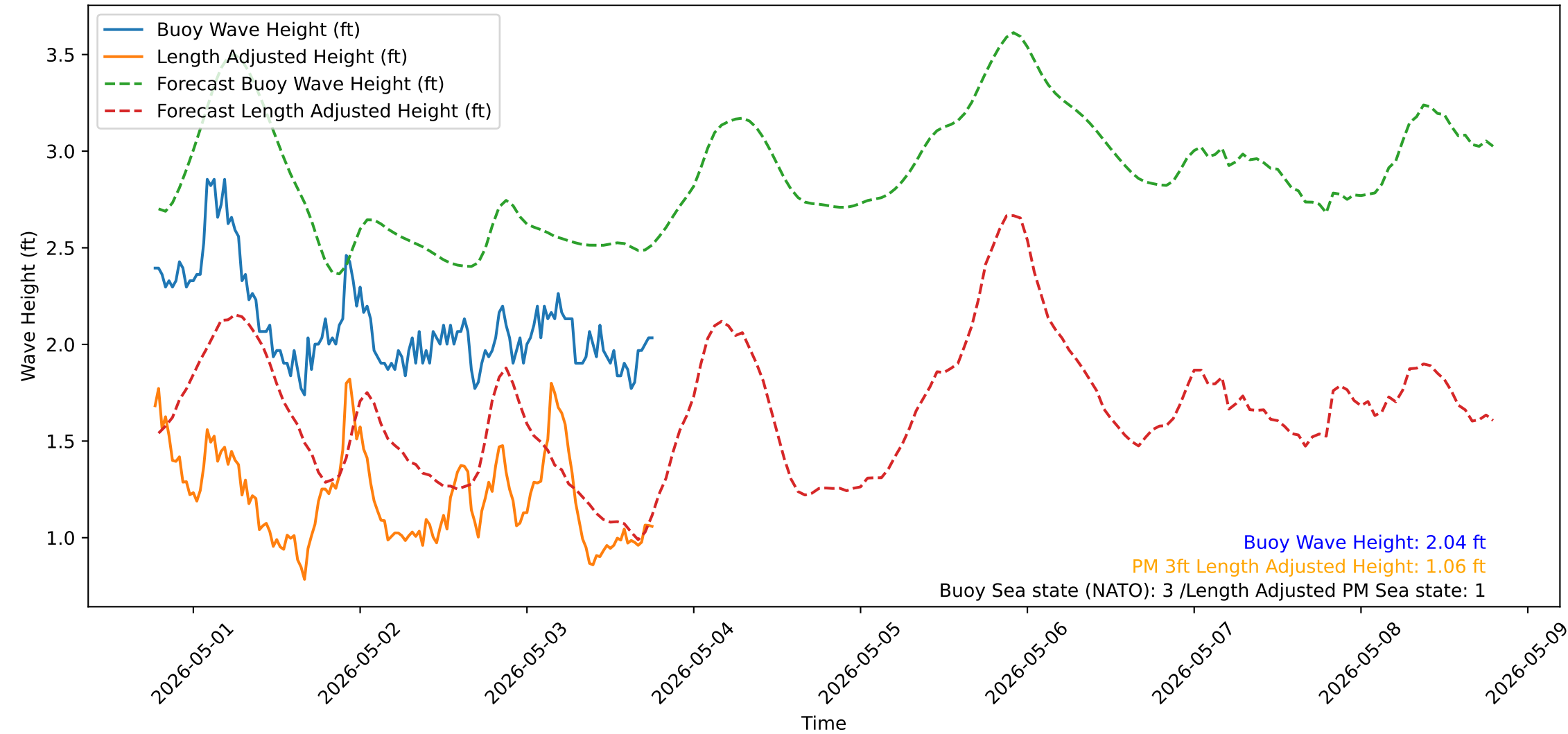
Wave Heights over Time for Green Beach at 2026-05-03 18:41:13
