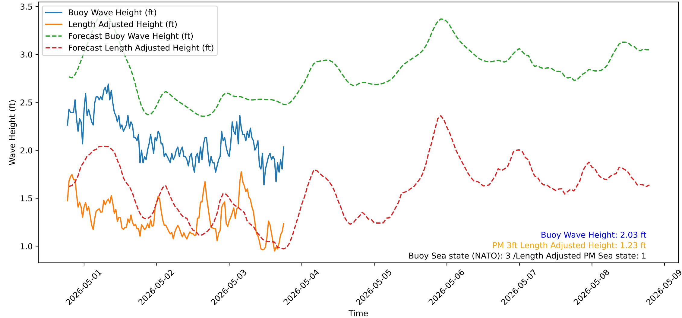
Wave Heights over Time for Oceanside Harbor at 2026-05-03 18:40:32
