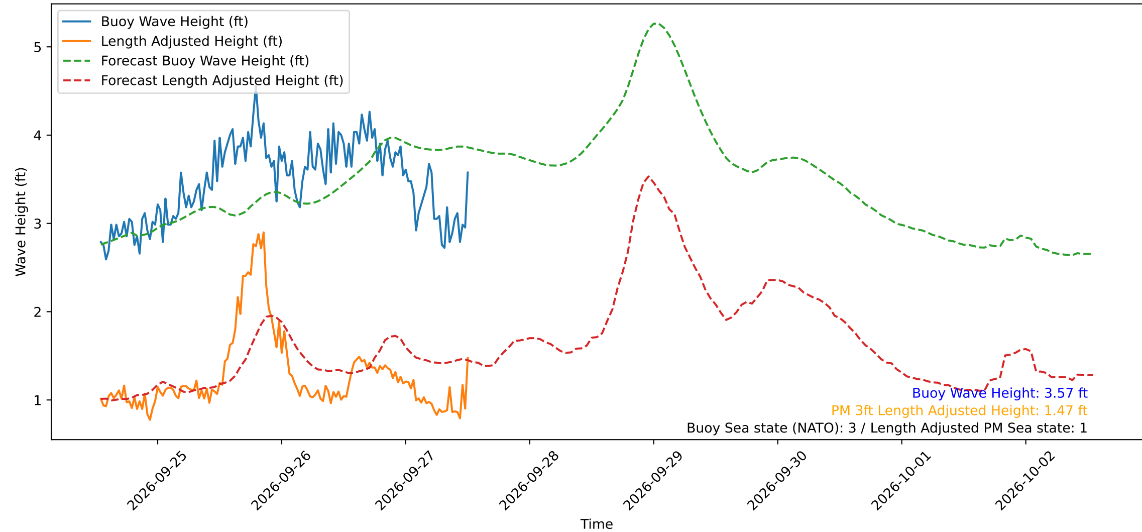
Wave Heights over Time for Green Beach at 2026-09-27 12:41:12
