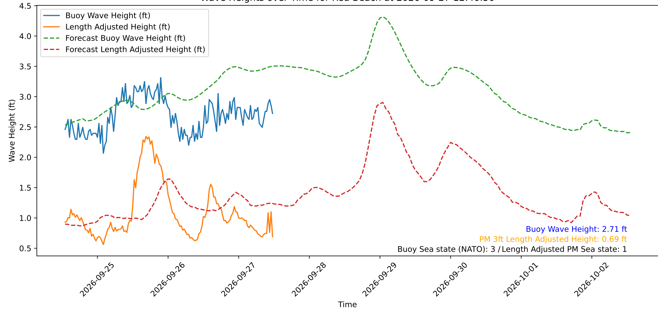
Wave Heights over Time for Red Beach at 2026-09-27 12:40:50
