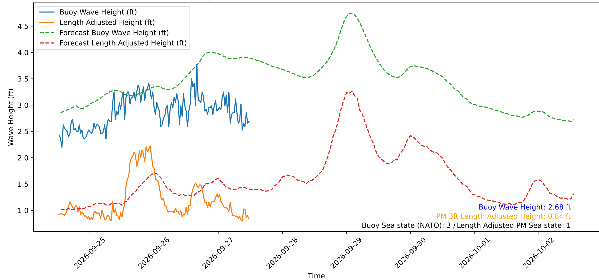
Wave Heights over Time for Oceanside Harbor at 2026-09-27 12:40:30
