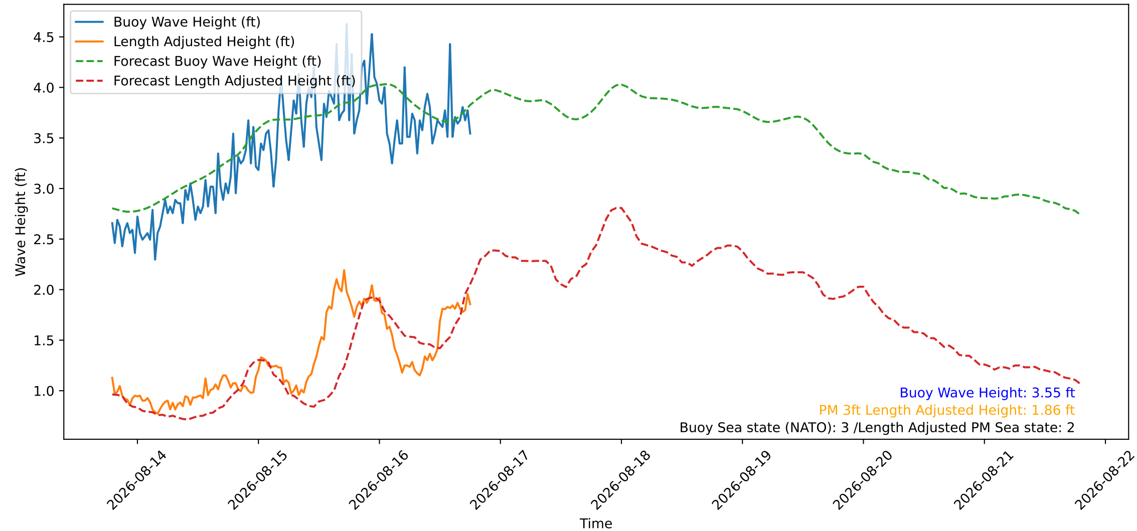
Wave Heights over Time for Oceanside Harbor at 2026-08-16 19:00:26
