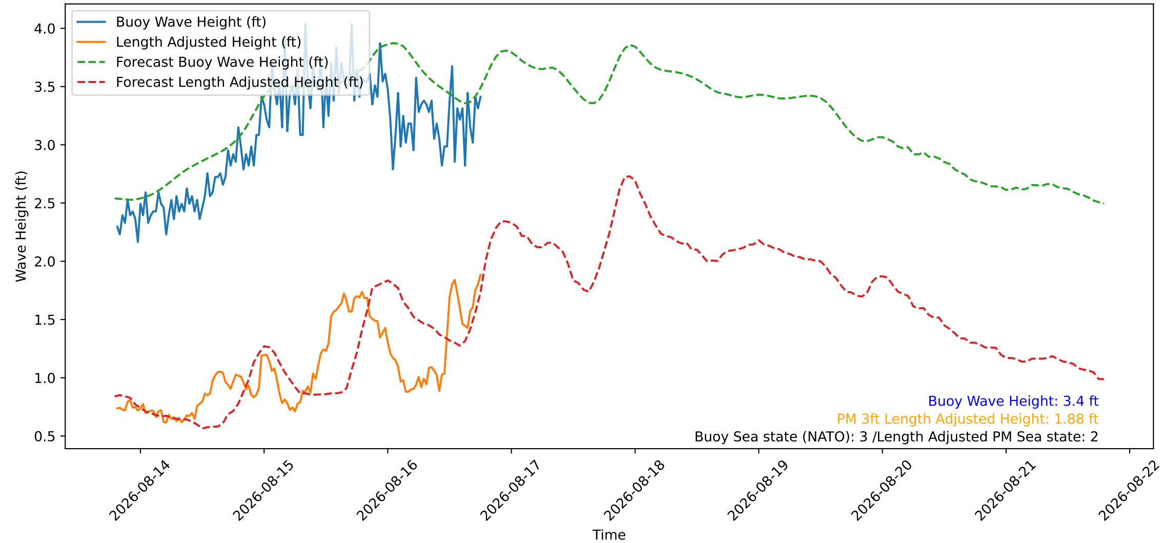
Wave Heights over Time for Red Beach at 2026-08-16 19:00:45
