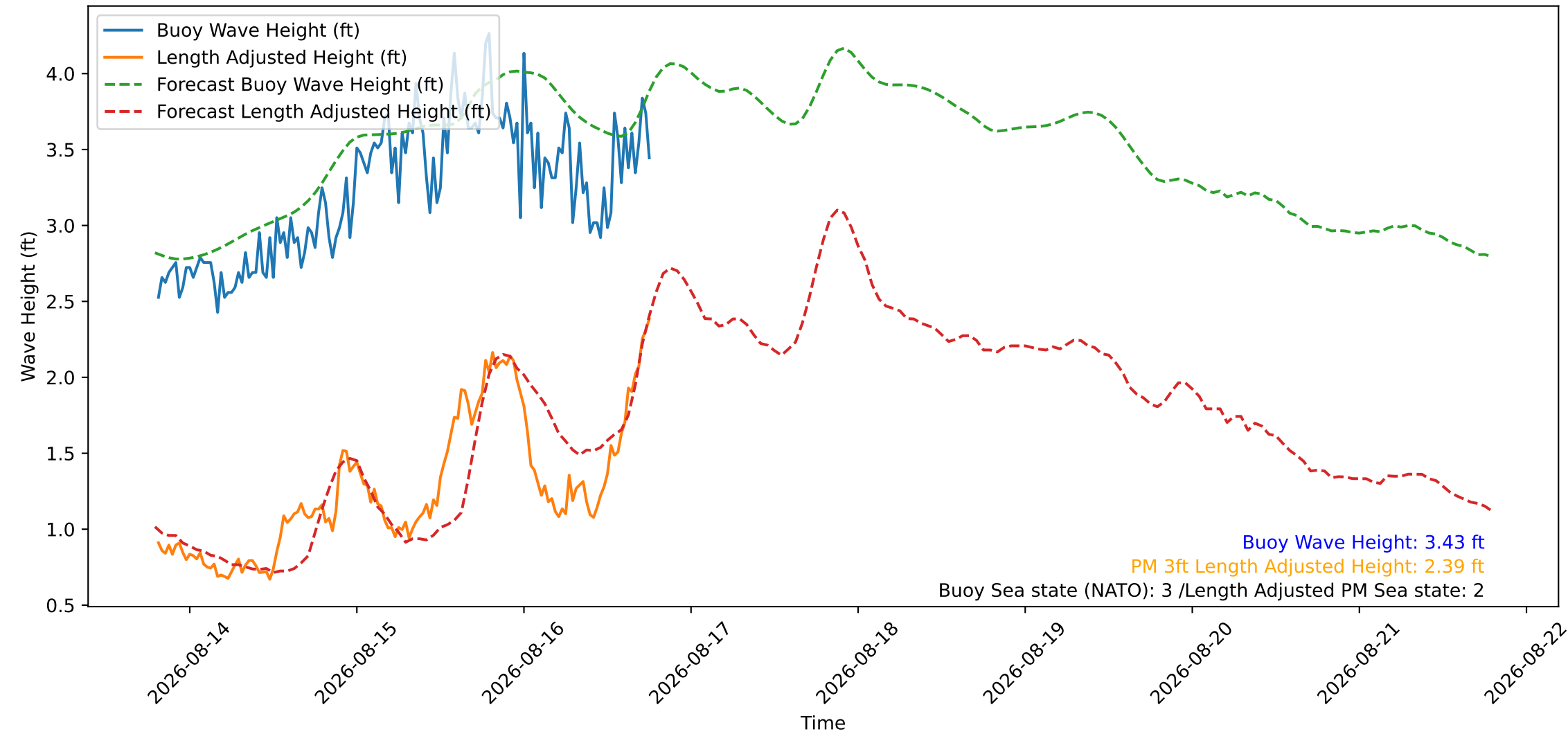
Wave Heights over Time for Green Beach at 2026-08-16 19:01:07
