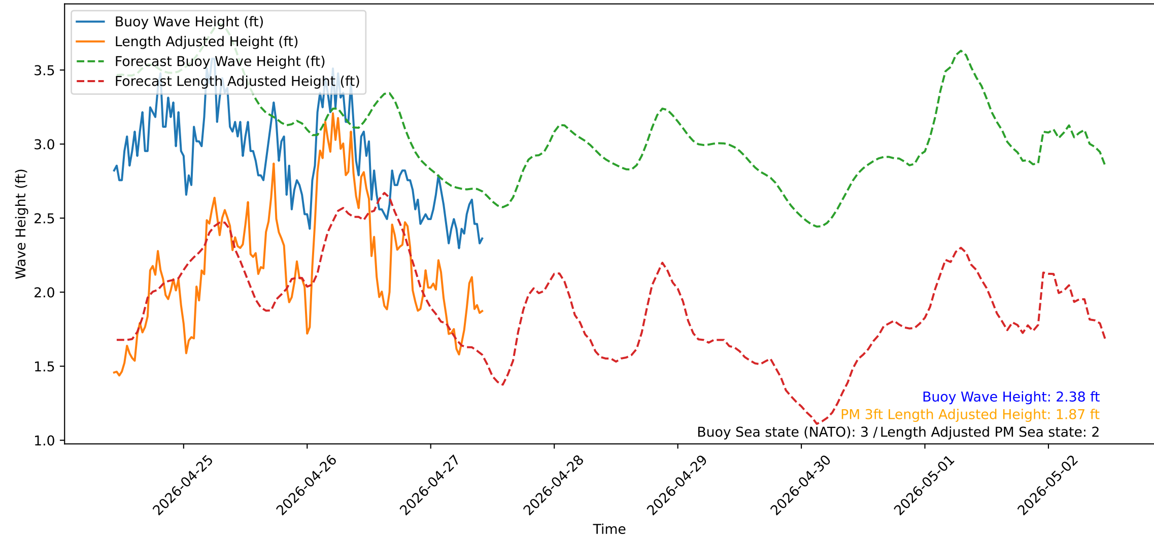
Wave Heights over Time for Green Beach at 2026-04-27 10:41:12
