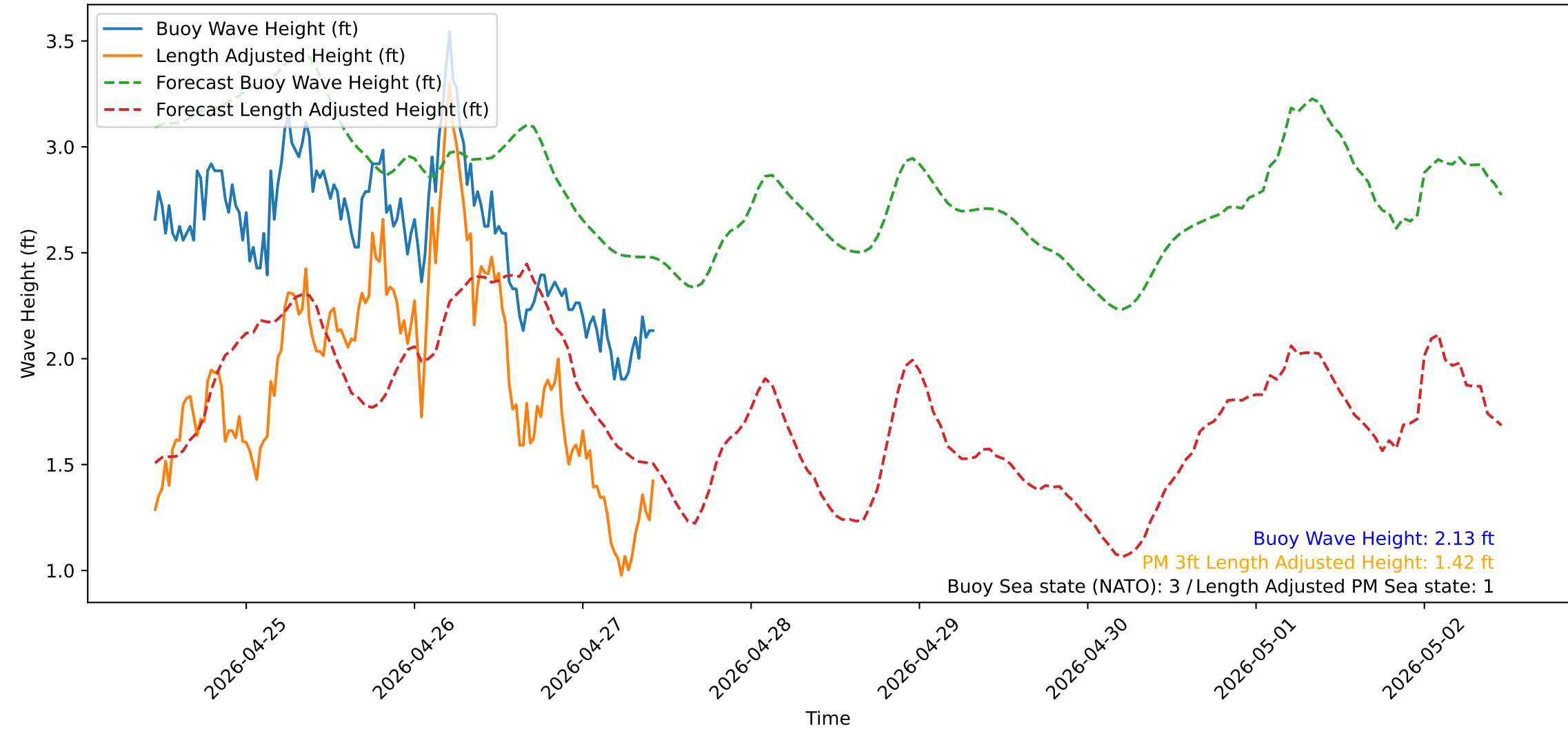
Wave Heights over Time for Red Beach at 2026-04-27 10:40:50
