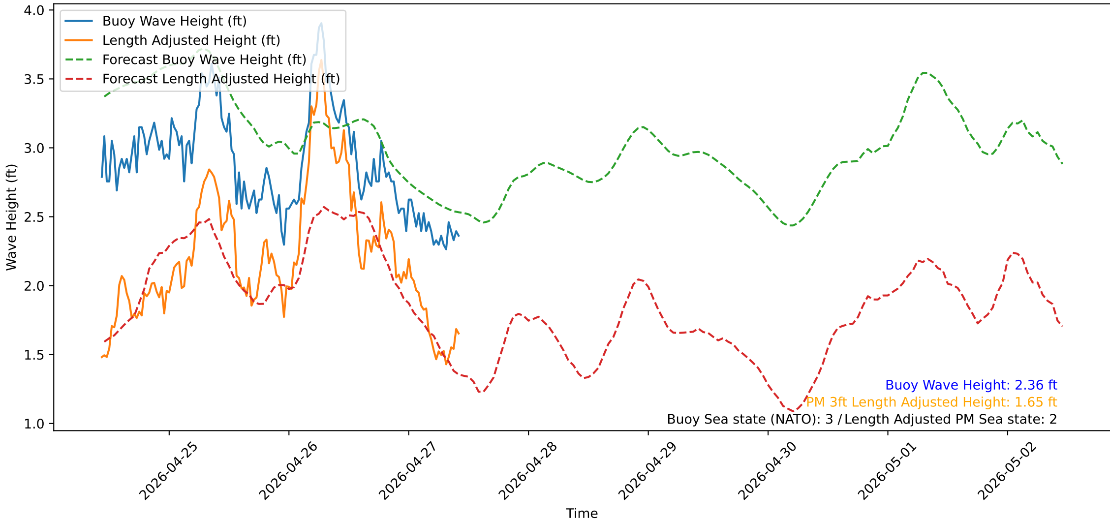
Wave Heights over Time for Oceanside Harbor at 2026-04-27 10:40:31
