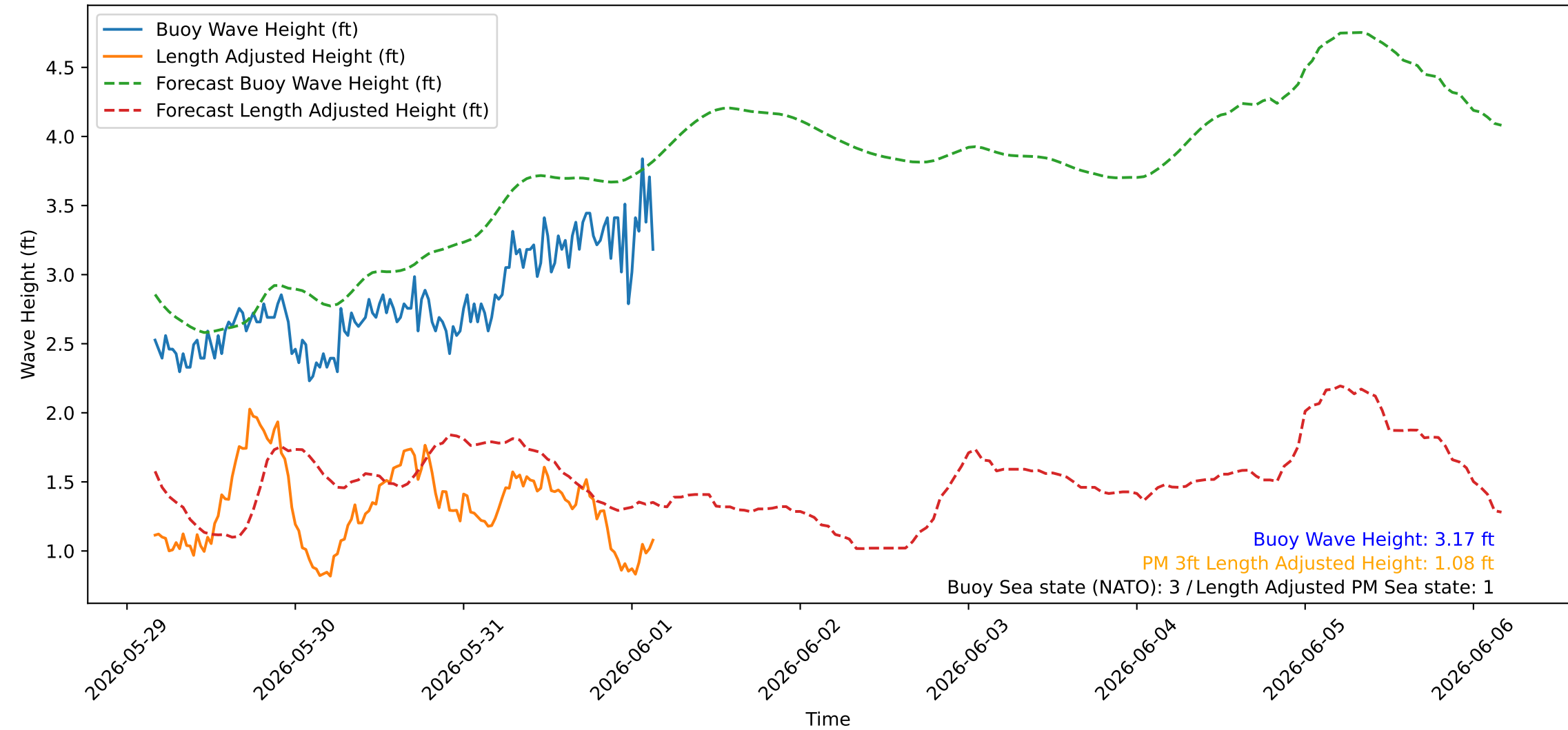
Wave Heights over Time for Red Beach at 2026-06-01 03:40:44
