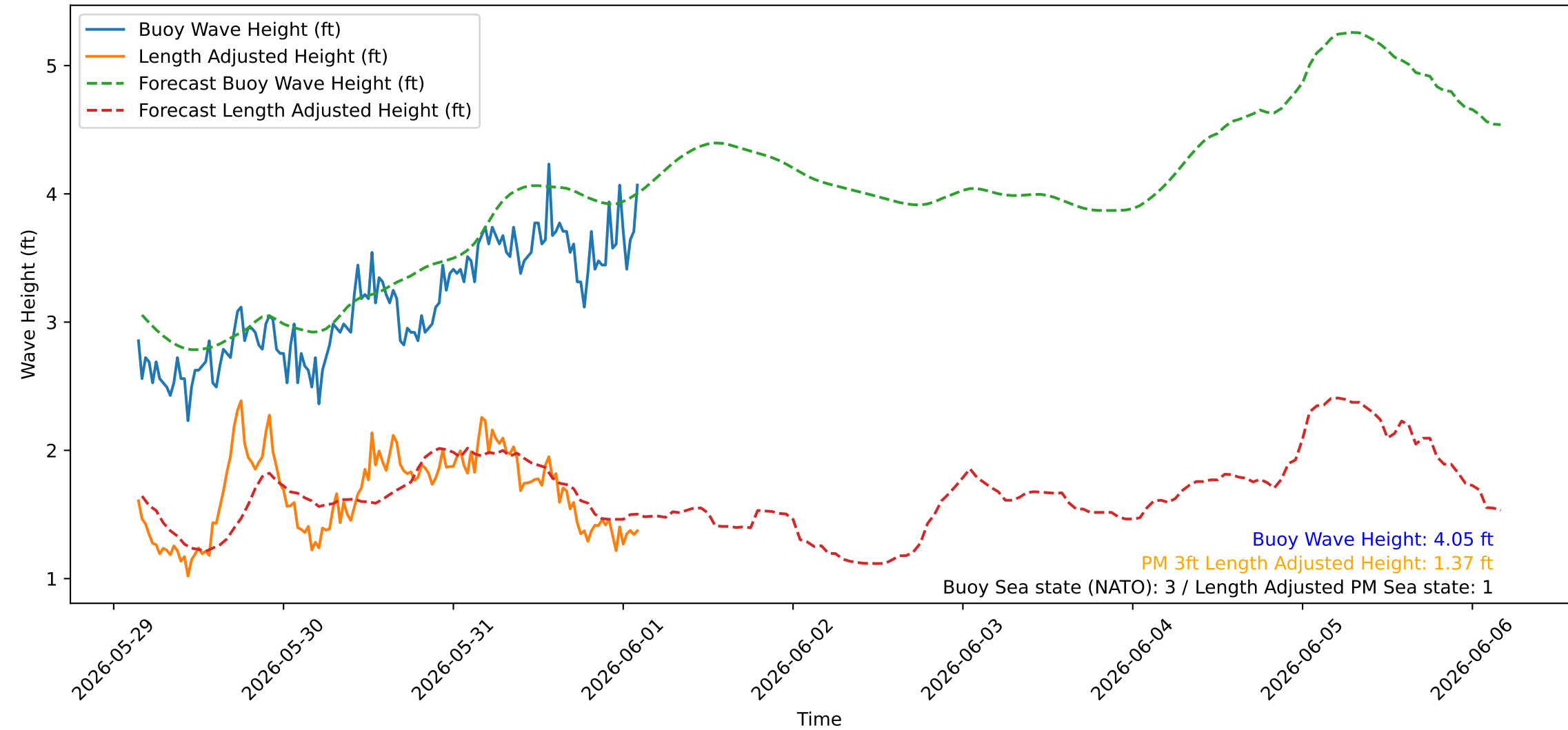
Wave Heights over Time for Oceanside Harbor at 2026-06-01 03:40:25
