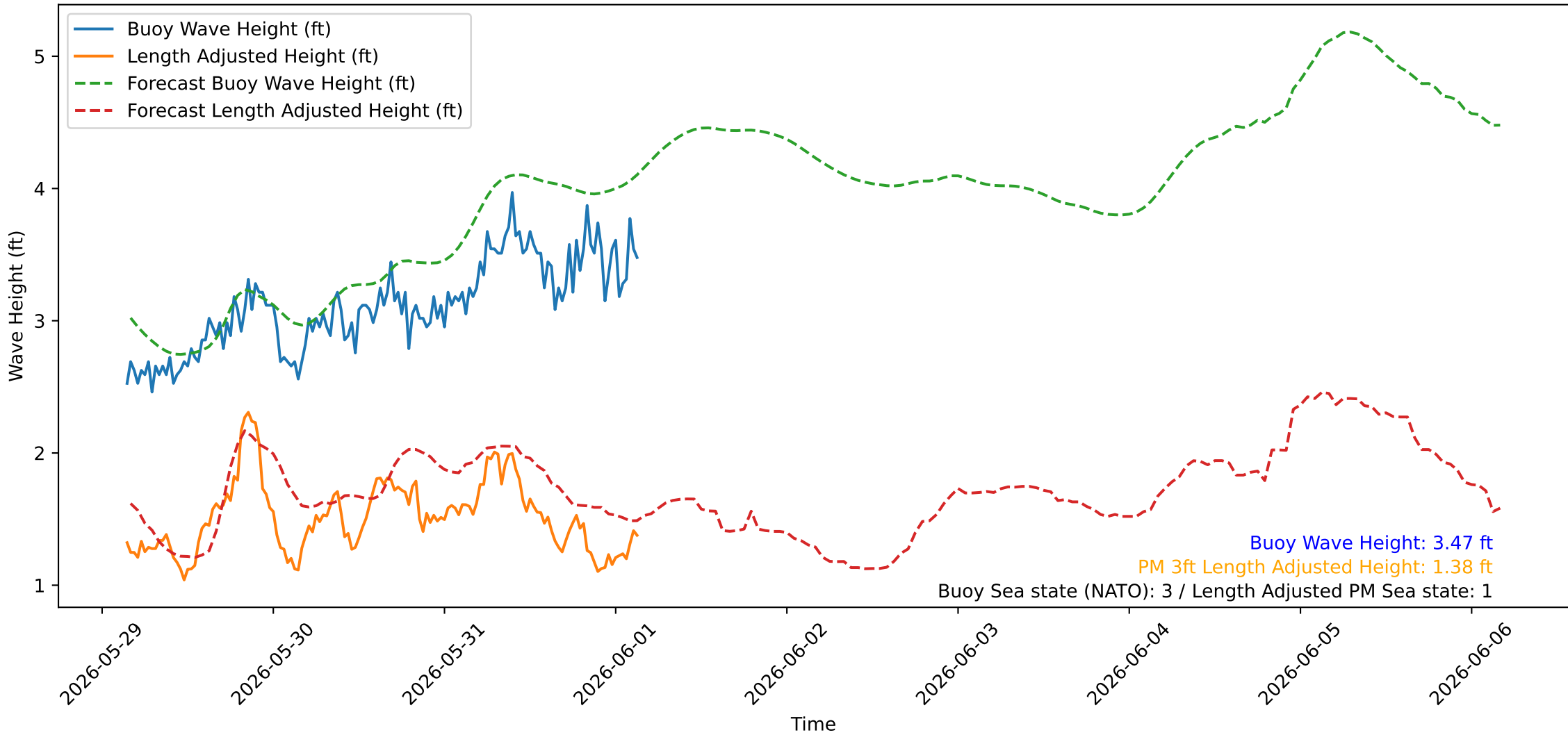
Wave Heights over Time for Green Beach at 2026-06-01 03:41:07
