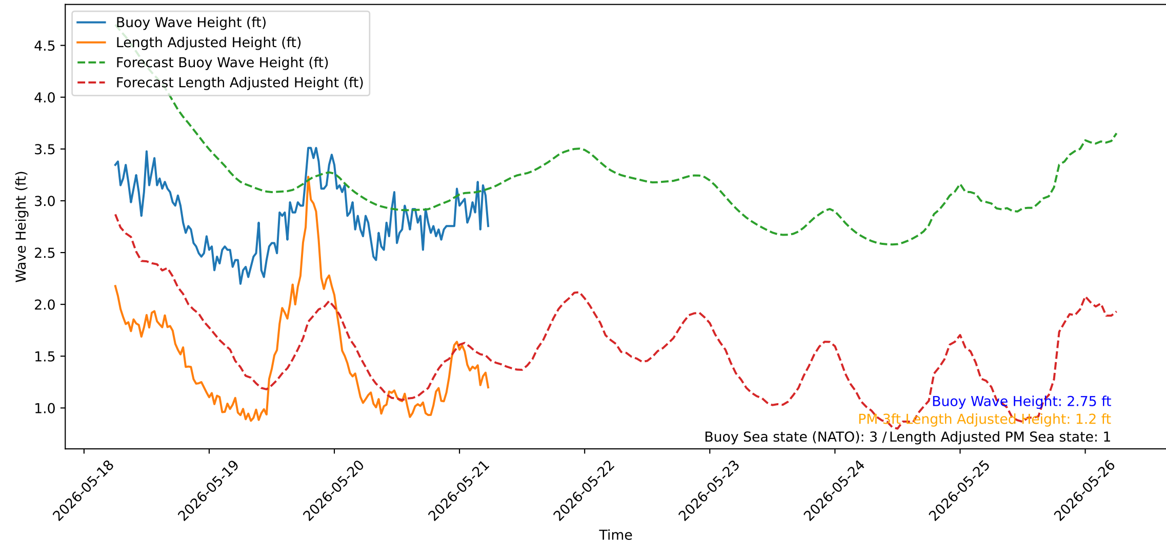
Wave Heights over Time for Oceanside Harbor at 2026-05-21 06:10:31
