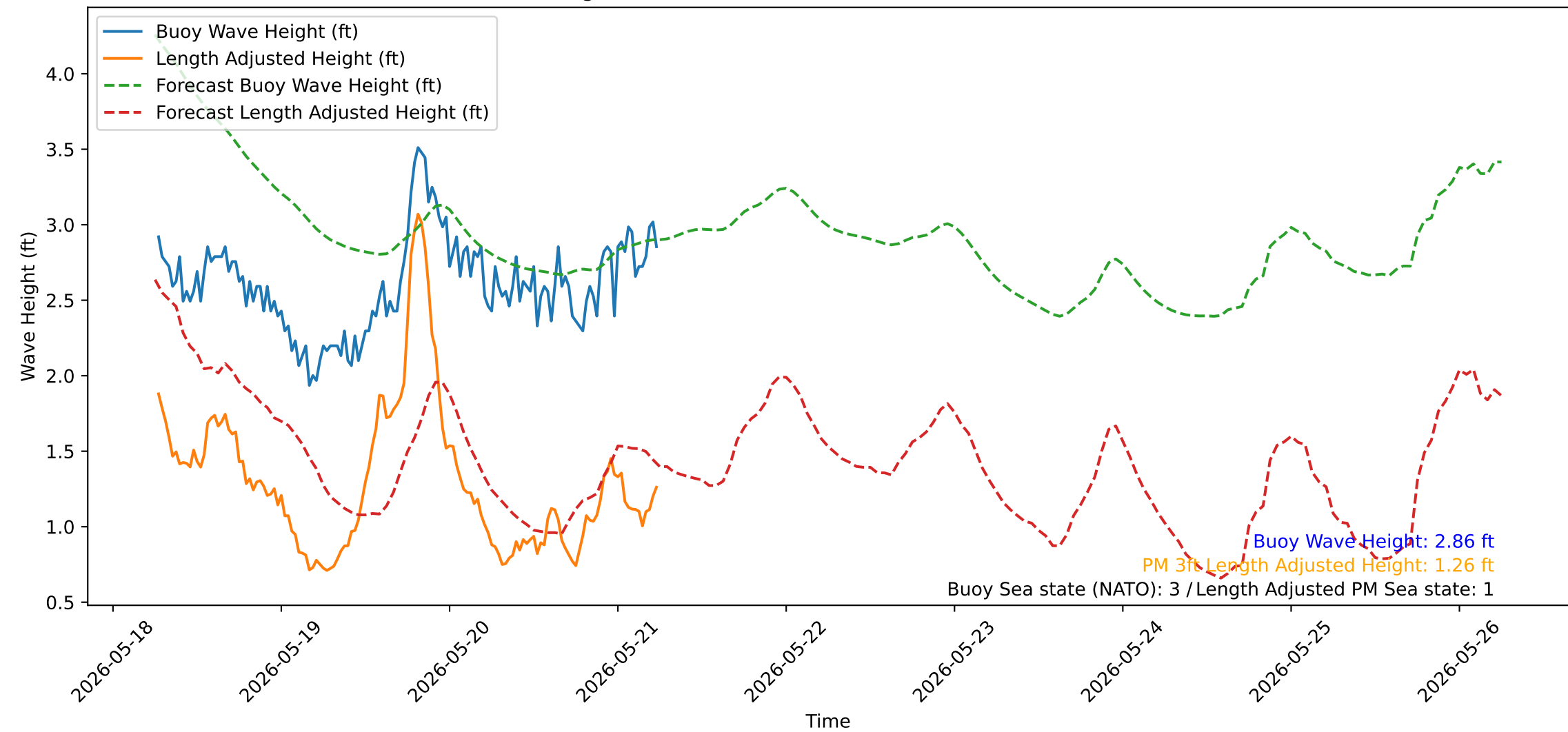
Wave Heights over Time for Red Beach at 2026-05-21 06:10:51
