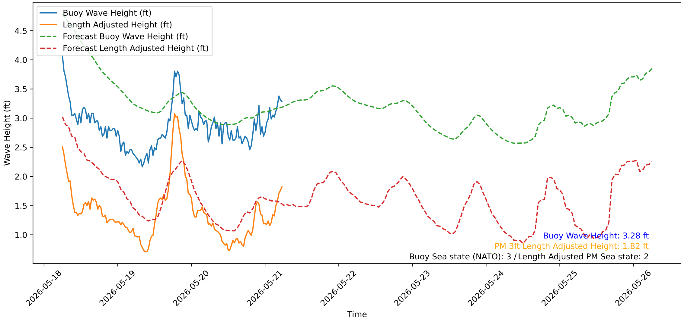
Wave Heights over Time for Green Beach at 2026-05-21 06:11:13
