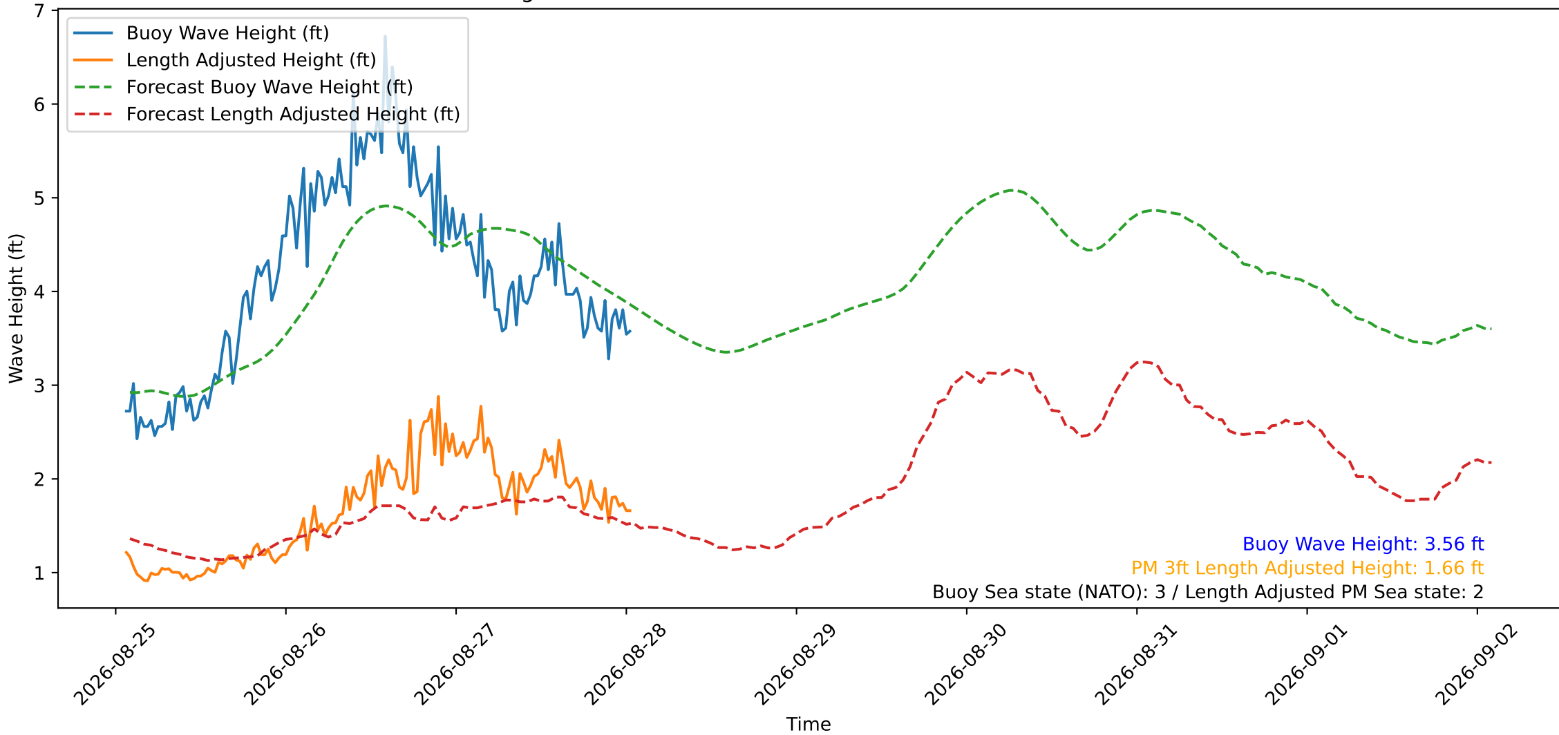
Wave Heights over Time for Oceanside Harbor at 2026-08-28 01:30:29
