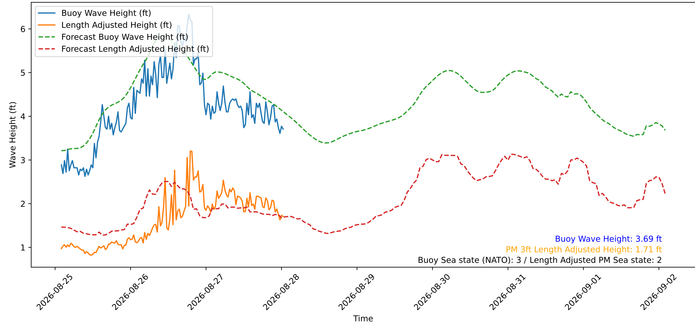
Wave Heights over Time for Green Beach at 2026-08-28 01:31:12
