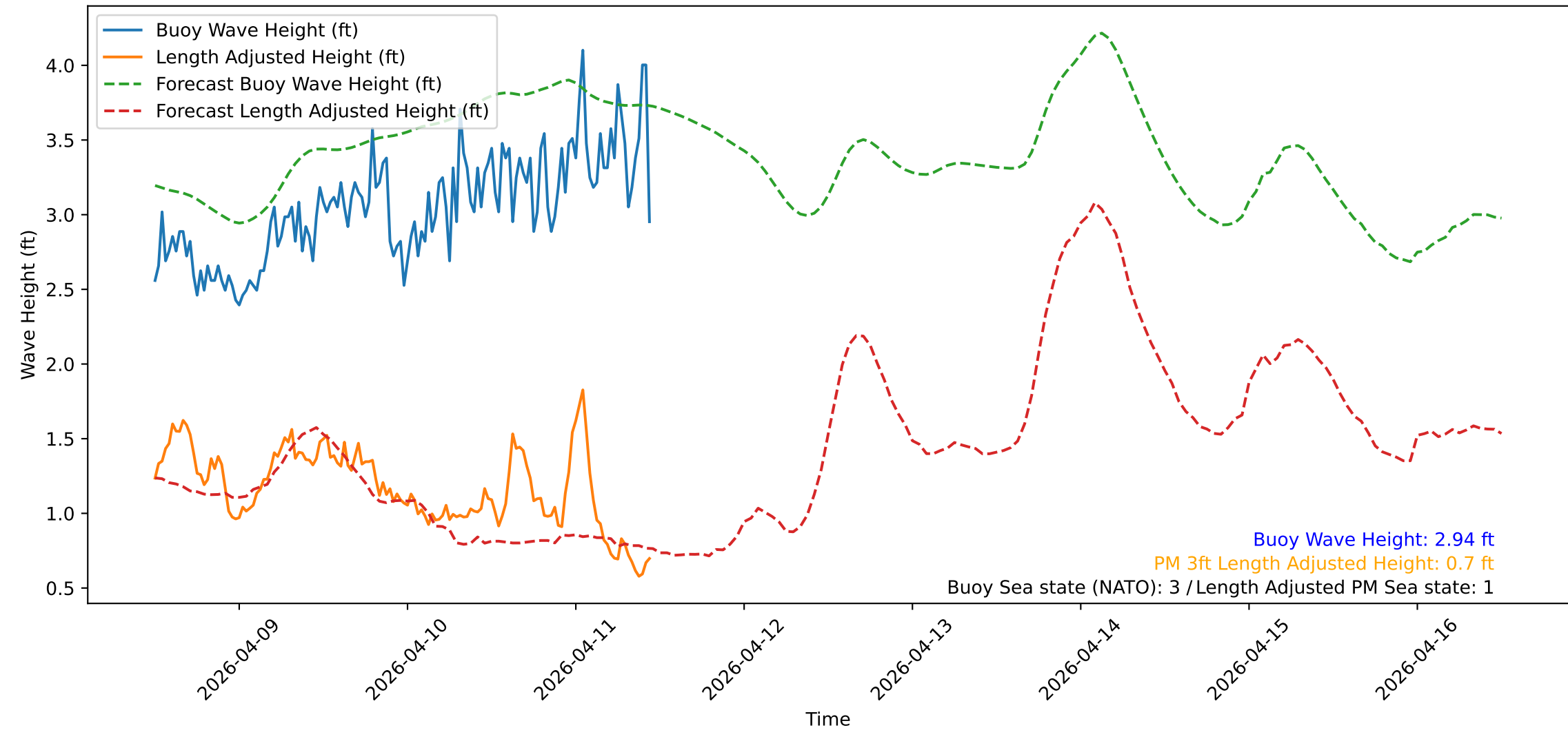
Wave Heights over Time for Red Beach at 2026-04-11 11:50:51
