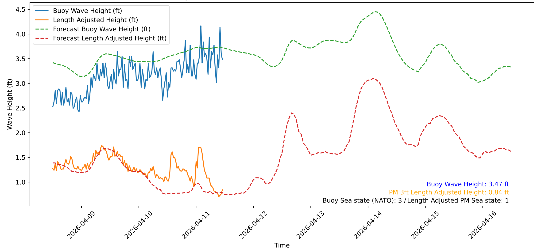
Wave Heights over Time for Oceanside Harbor at 2026-04-11 11:50:31
