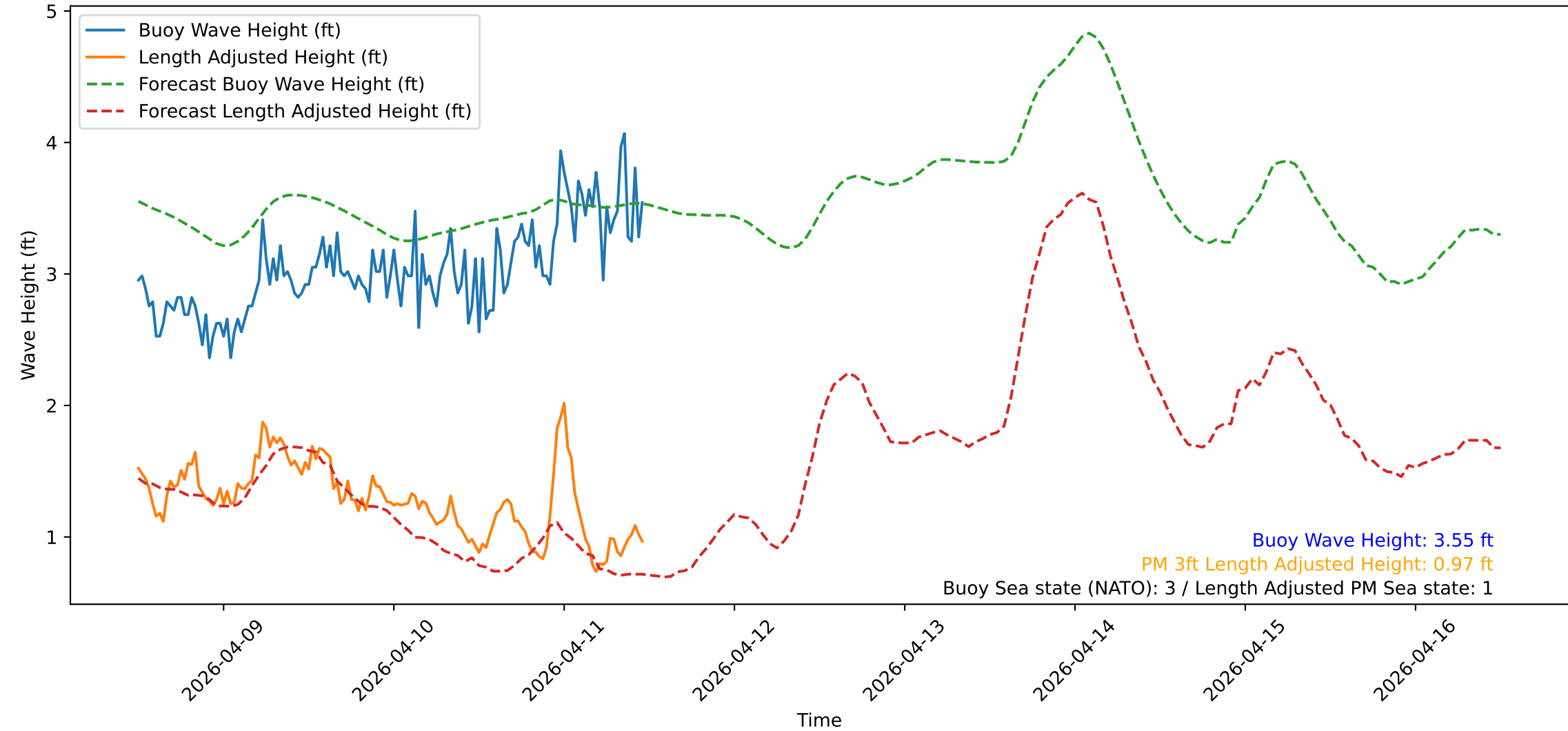
Wave Heights over Time for Green Beach at 2026-04-11 11:51:14
