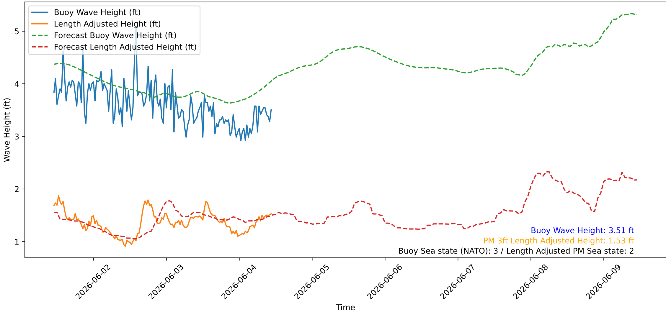
Wave Heights over Time for Oceanside Harbor at 2026-06-04 11:10:26
