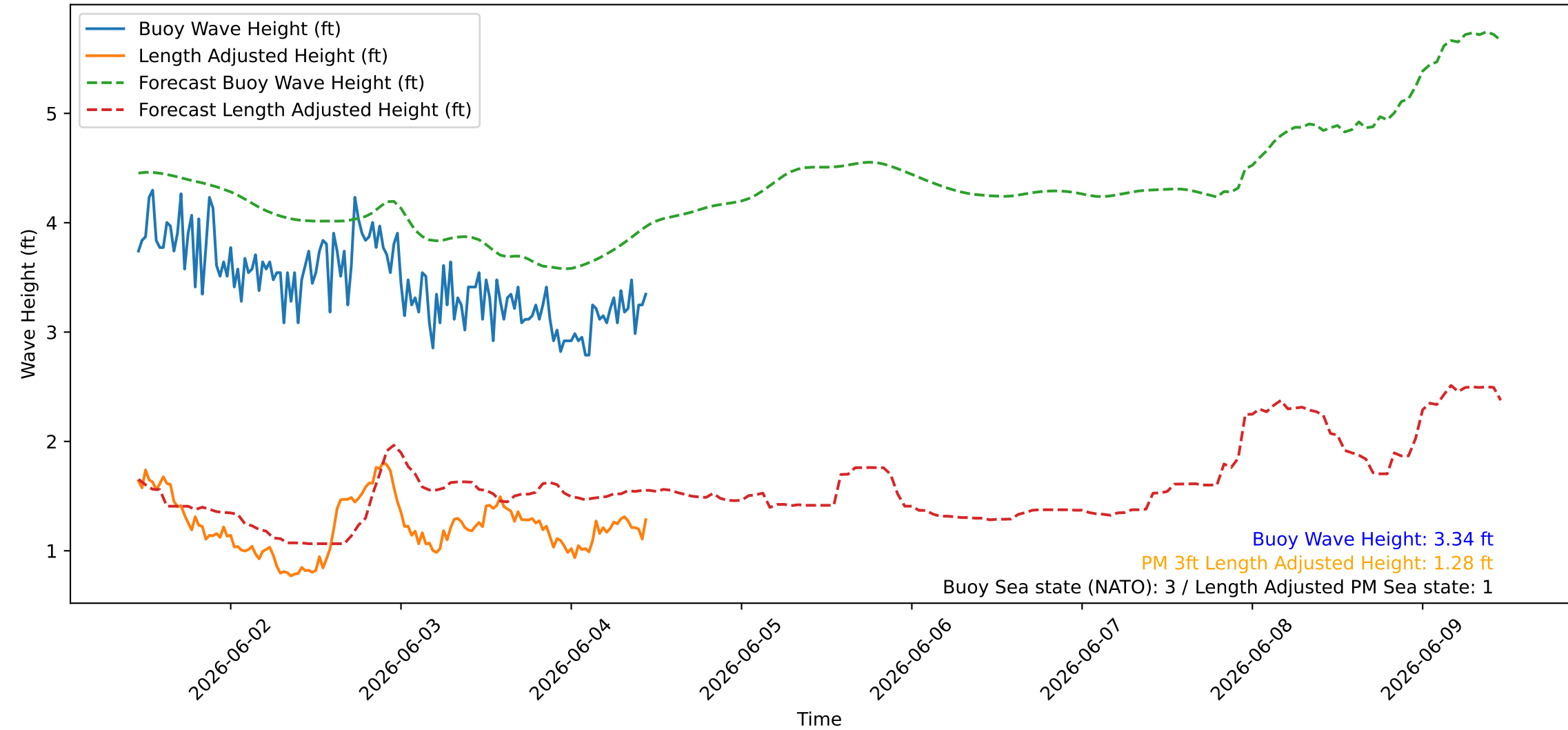
Wave Heights over Time for Green Beach at 2026-06-04 11:11:08
