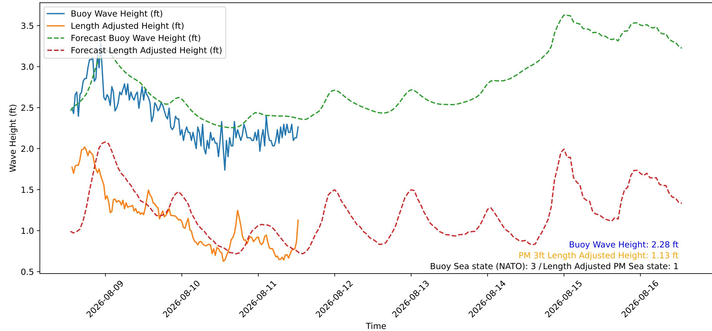
Wave Heights over Time for Red Beach at 2026-08-11 13:10:47
