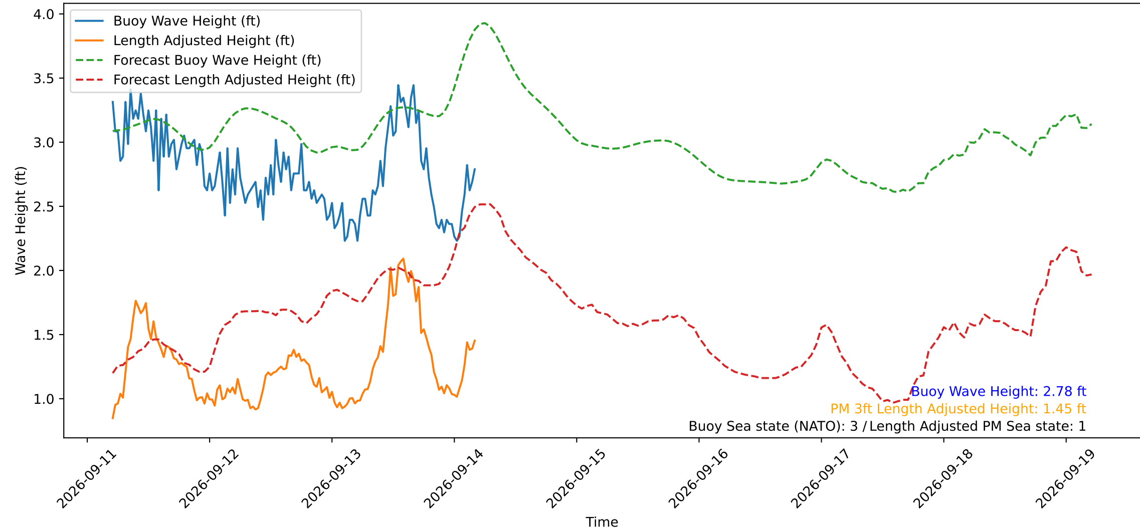
Wave Heights over Time for Red Beach at 2026-09-14 04:40:48
