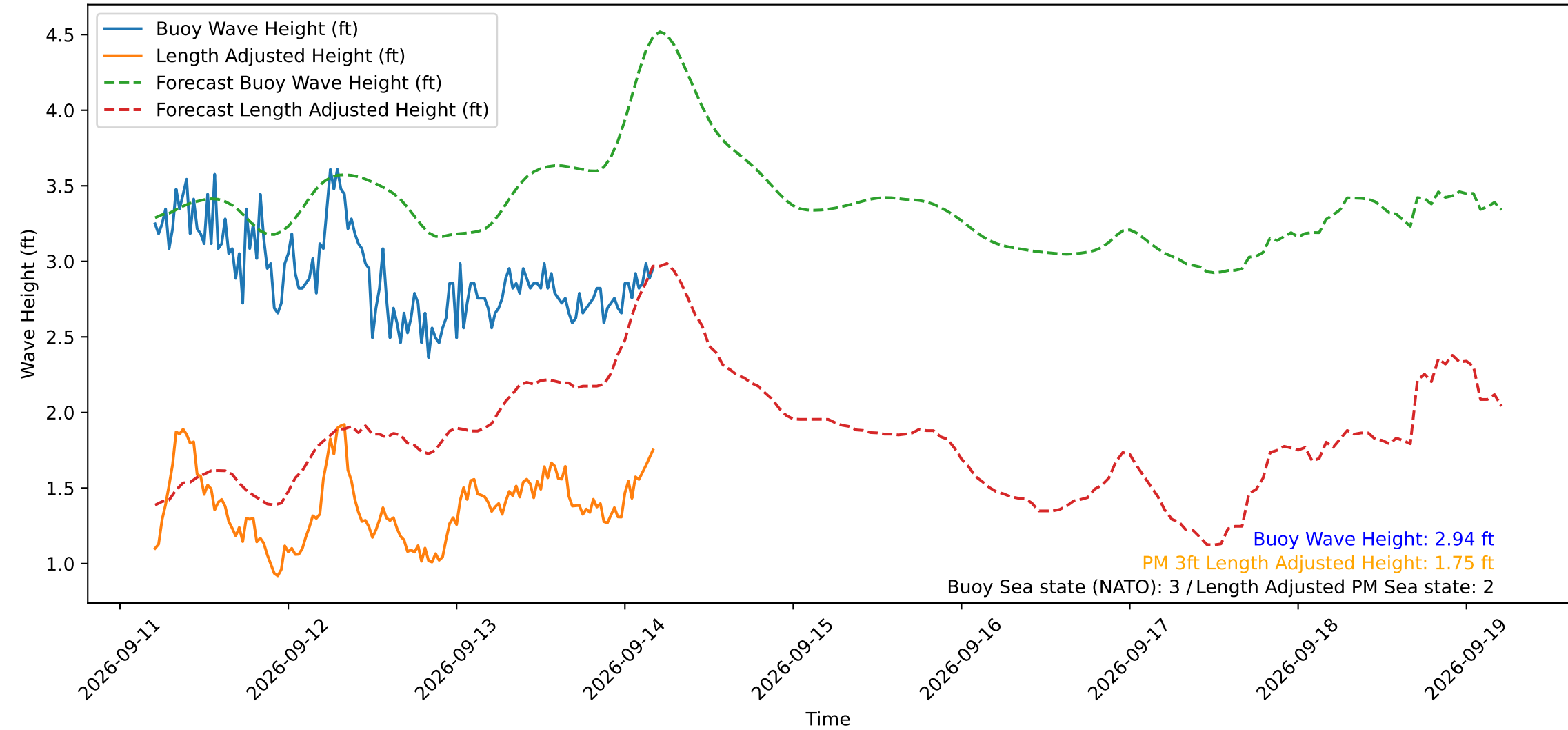
Wave Heights over Time for Green Beach at 2026-09-14 04:41:11
