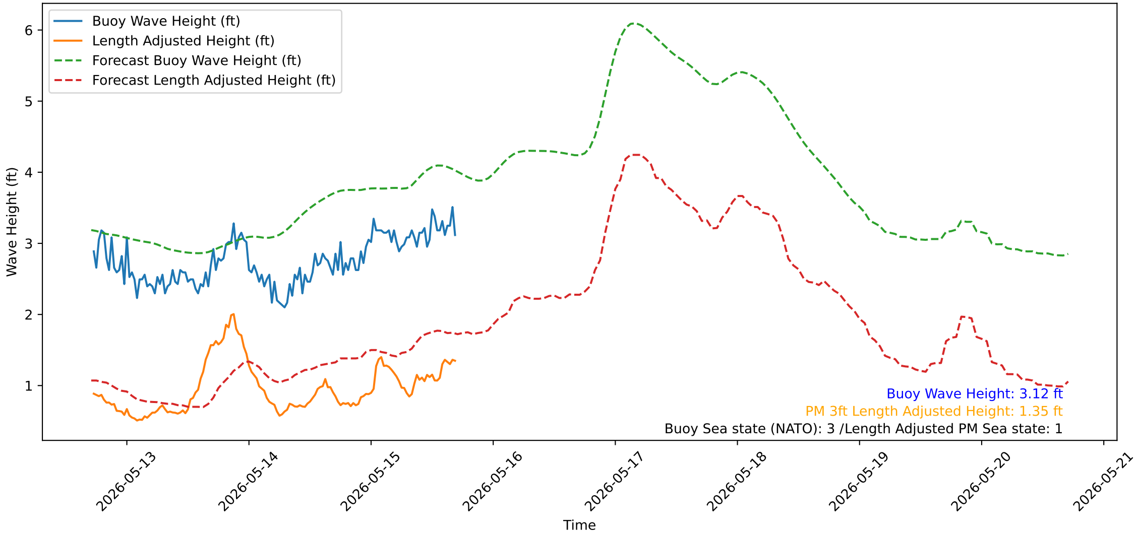
Wave Heights over Time for Green Beach at 2026-05-15 17:21:14
