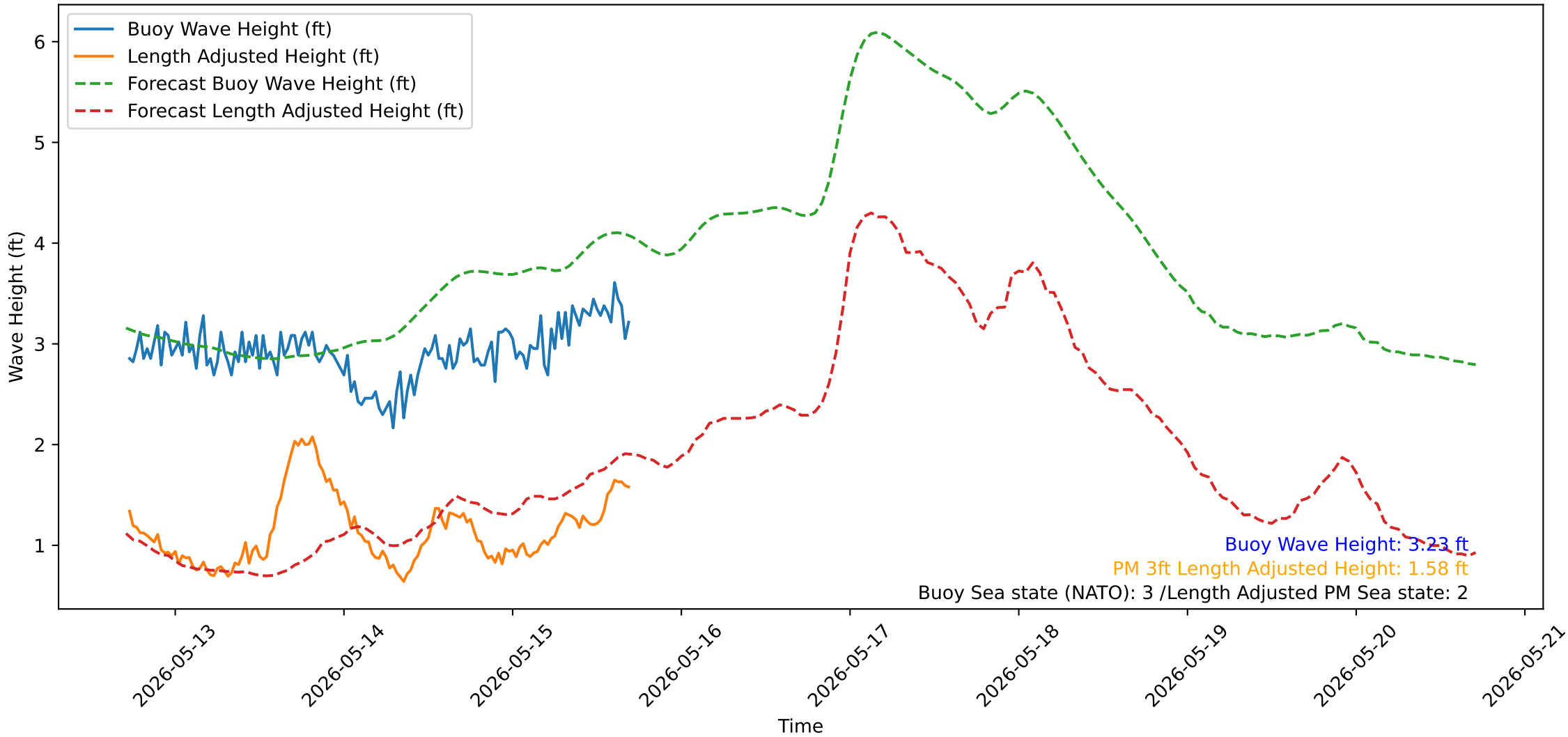
Wave Heights over Time for Oceanside Harbor at 2026-05-15 17:20:31
