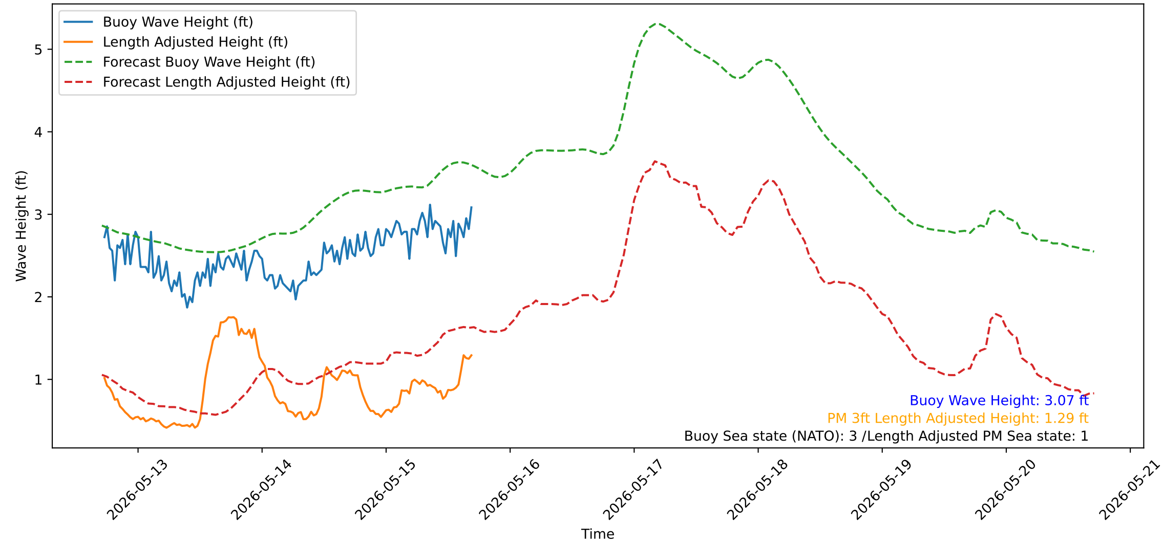
Wave Heights over Time for Red Beach at 2026-05-15 17:20:52
