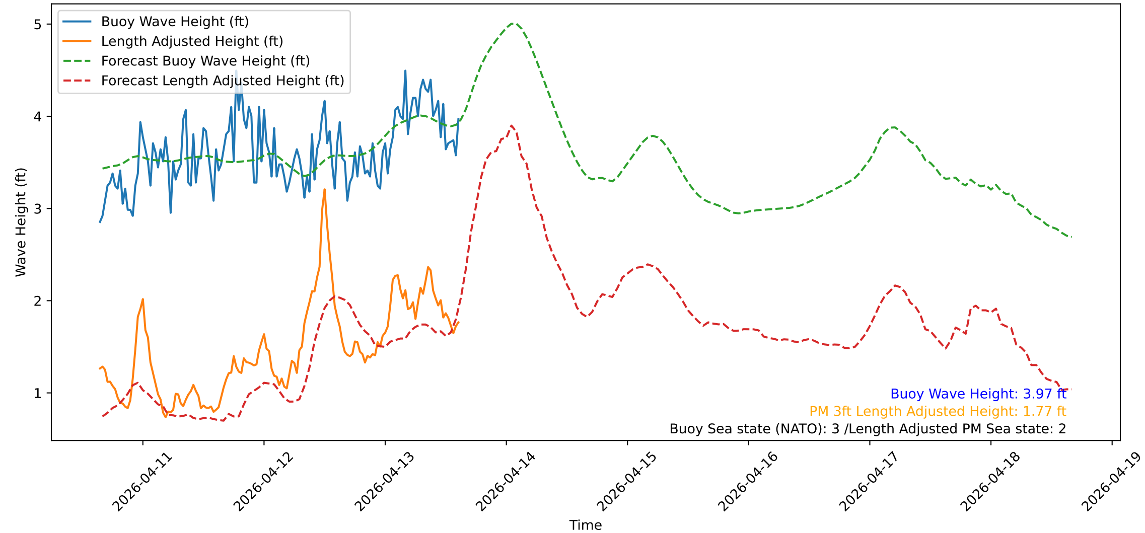
Wave Heights over Time for Green Beach at 2026-04-13 15:31:14
