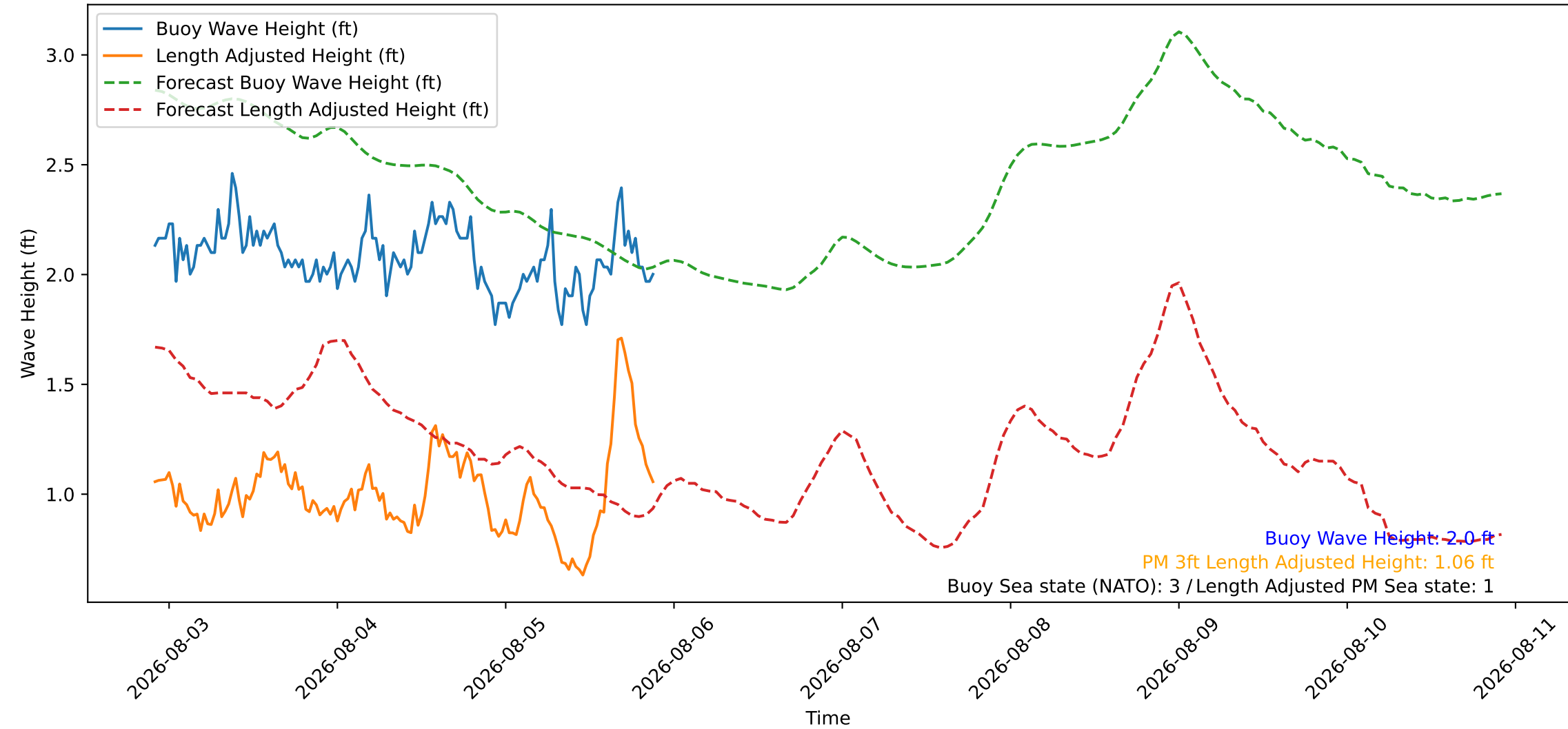
Wave Heights over Time for Red Beach at 2026-08-05 21:50:46
