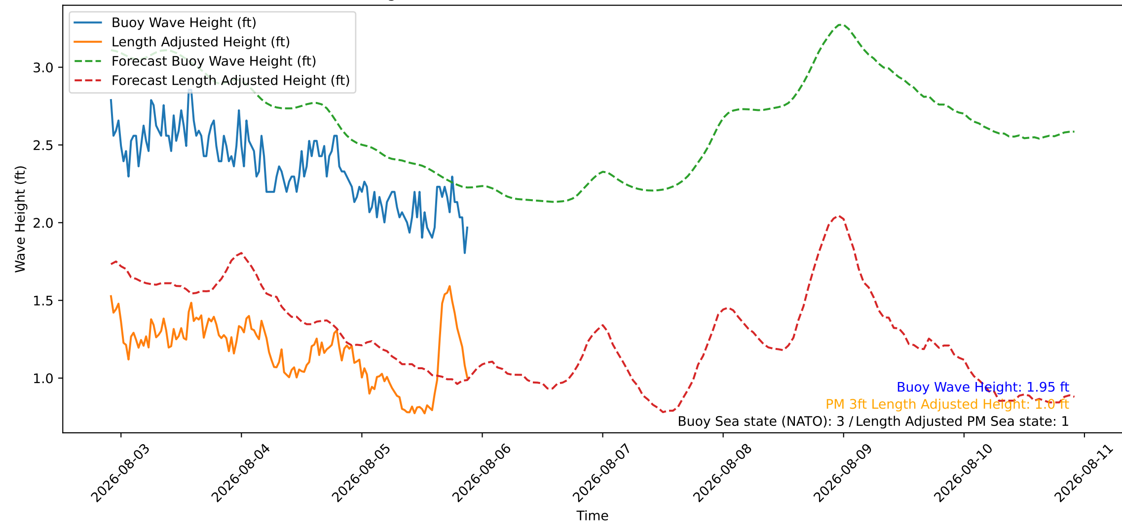
Wave Heights over Time for Oceanside Harbor at 2026-08-05 21:50:26
