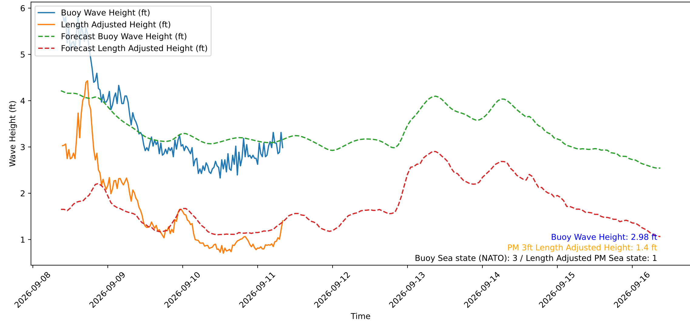
Wave Heights over Time for Red Beach at 2026-09-11 09:00:49
