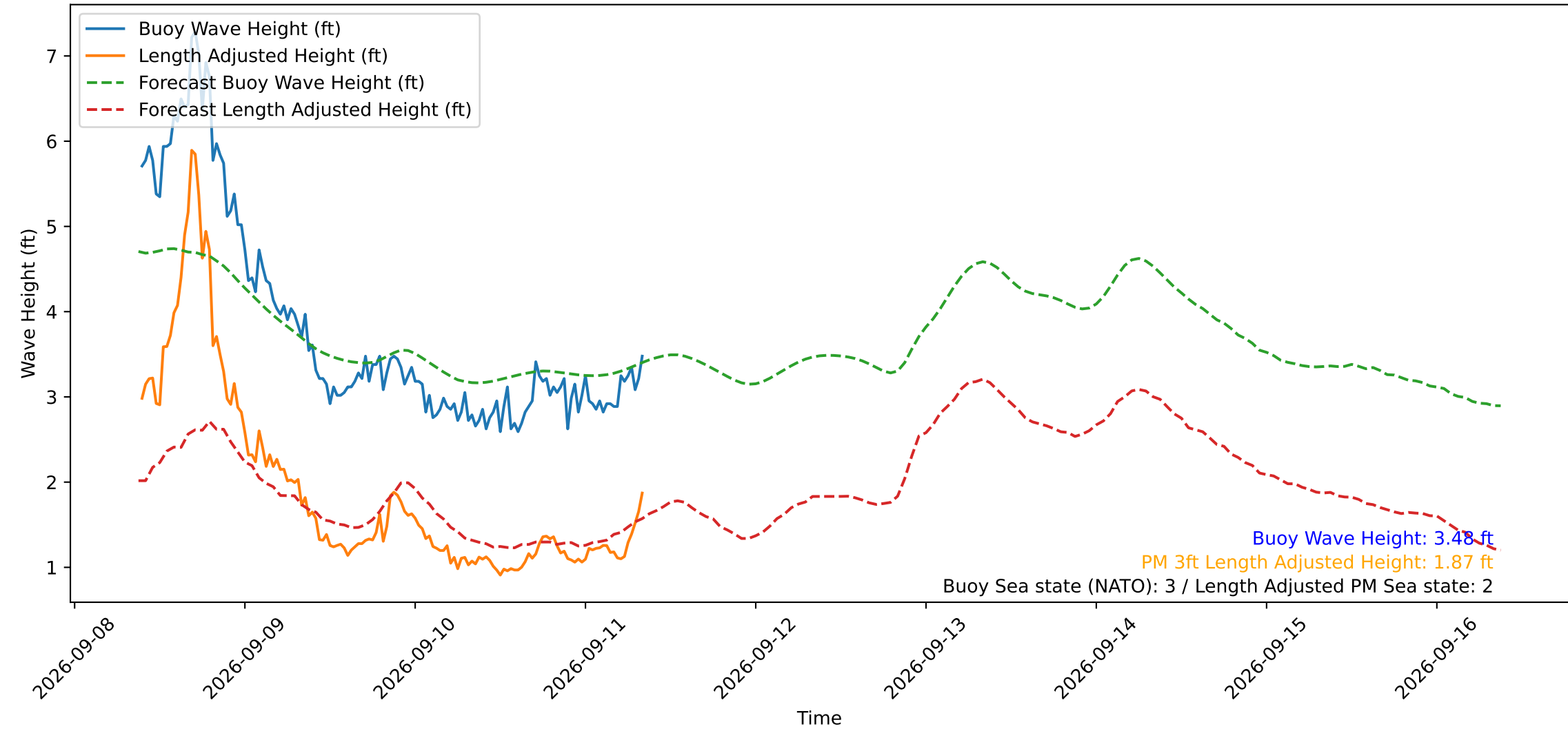
Wave Heights over Time for Green Beach at 2026-09-11 09:01:12
