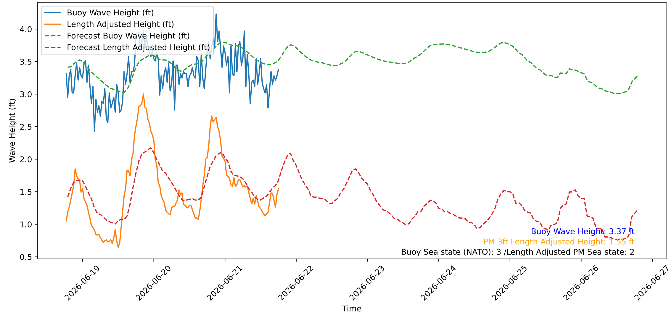
Wave Heights over Time for Green Beach at 2026-06-21 18:41:09
