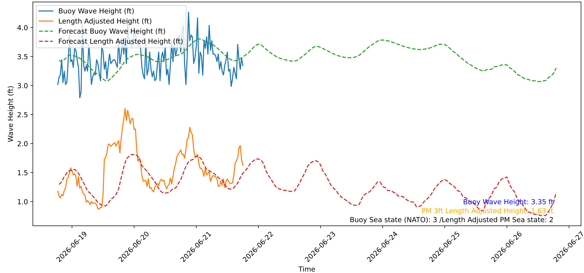
Wave Heights over Time for Oceanside Harbor at 2026-06-21 18:40:26
