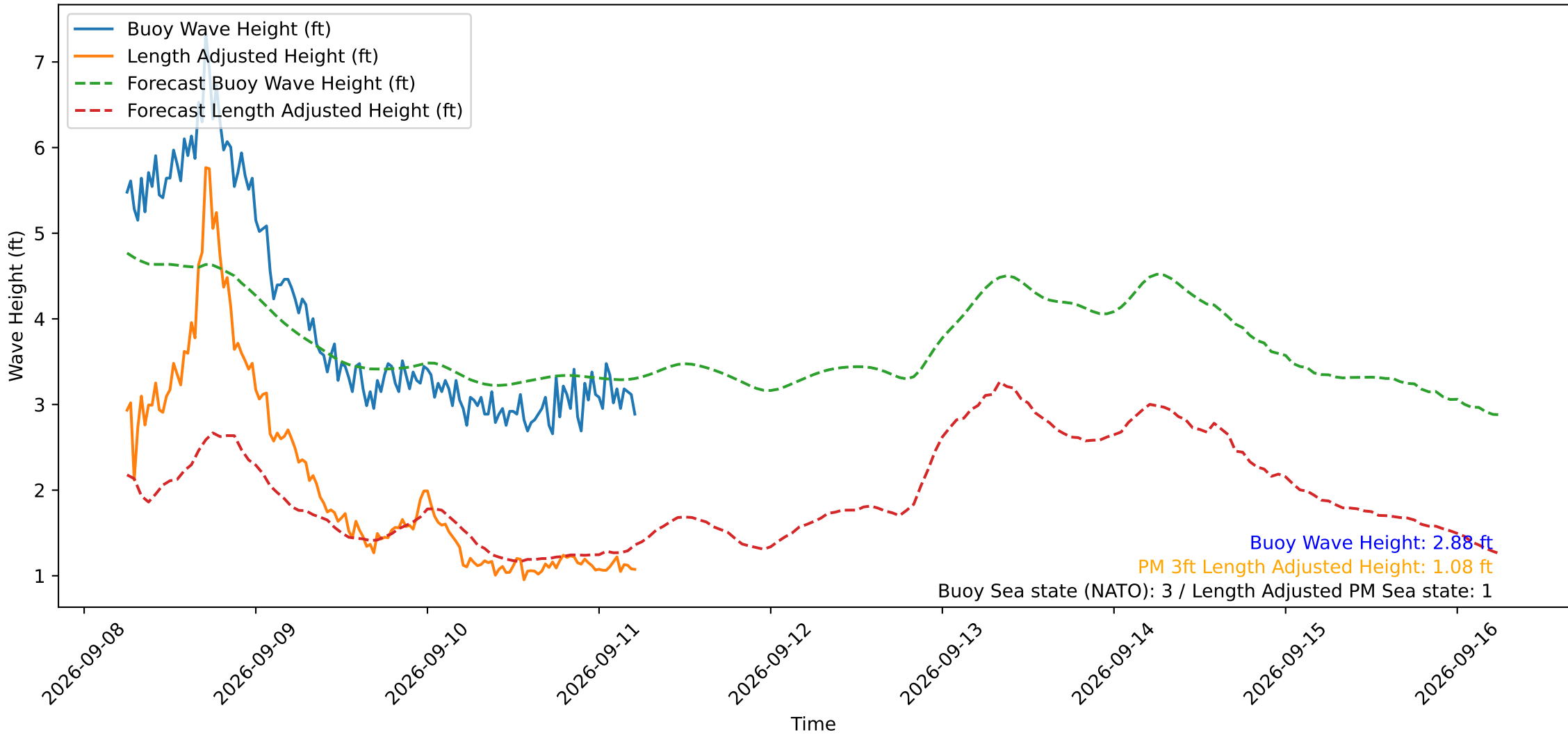
Wave Heights over Time for Oceanside Harbor at 2026-09-11 06:00:30
