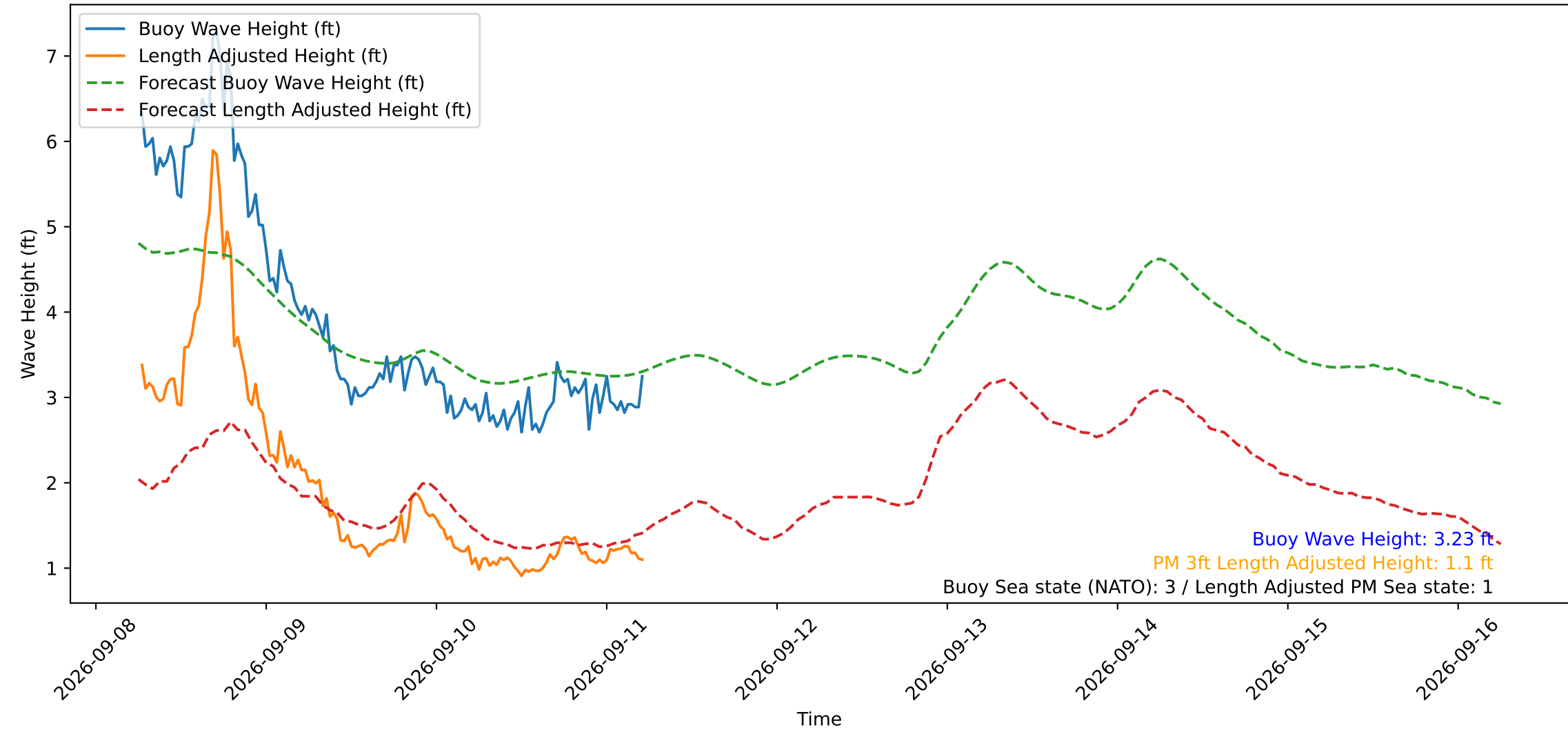
Wave Heights over Time for Green Beach at 2026-09-11 06:01:12
