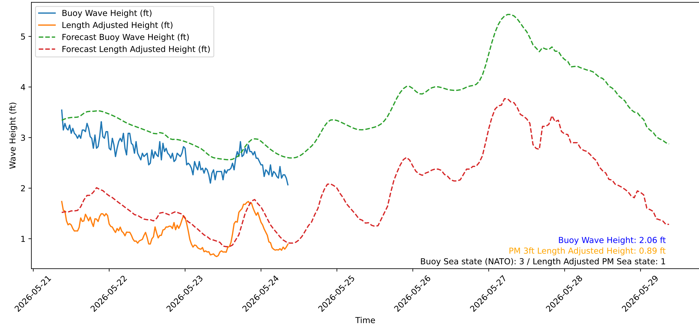
Wave Heights over Time for Green Beach at 2026-05-24 09:11:15
