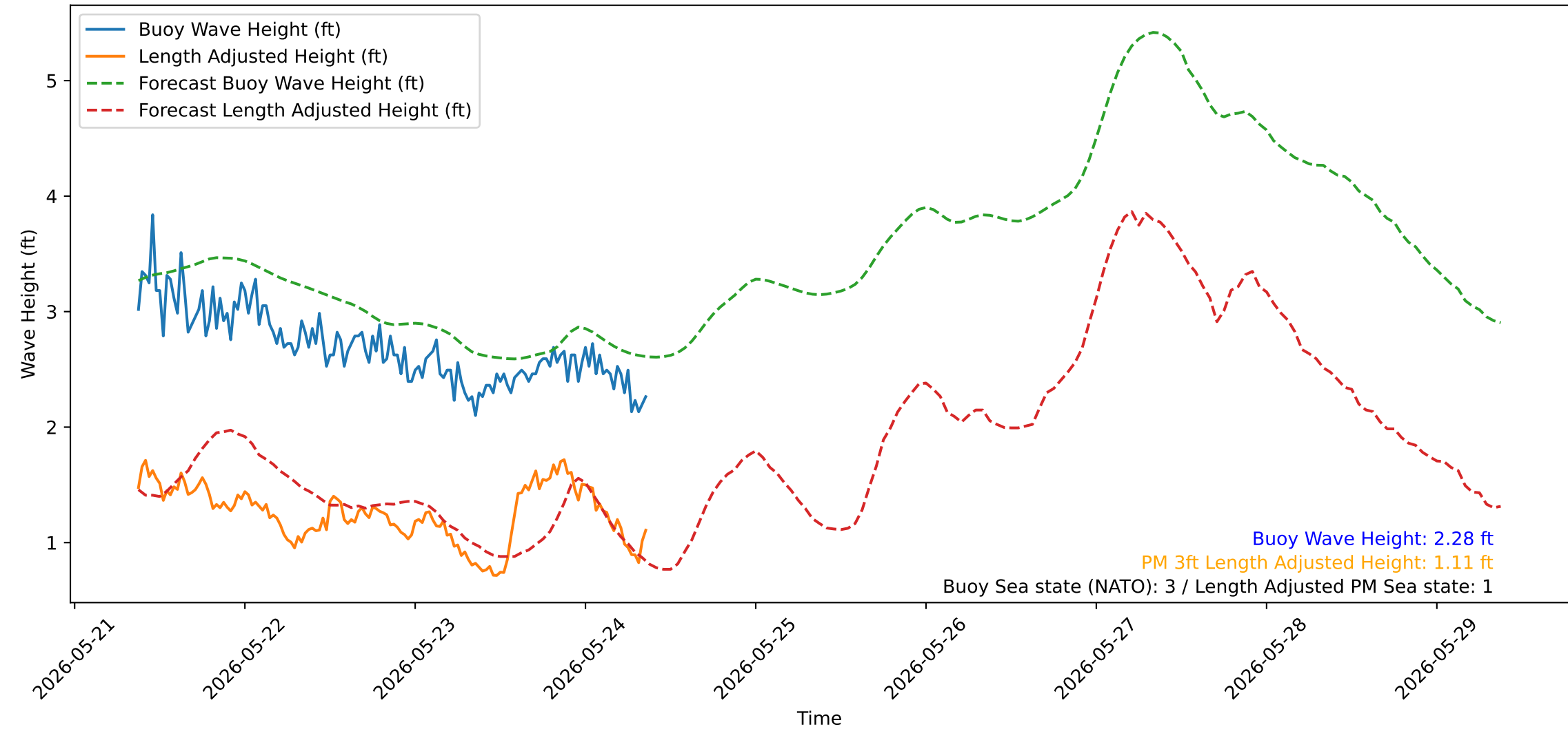
Wave Heights over Time for Oceanside Harbor at 2026-05-24 09:10:32
