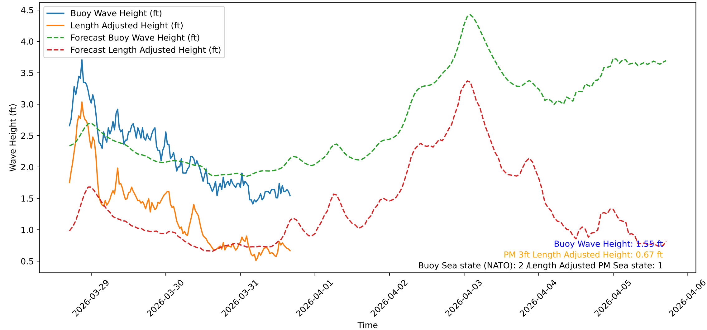
Wave Heights over Time for Green Beach at 2026-03-31 16:51:10
