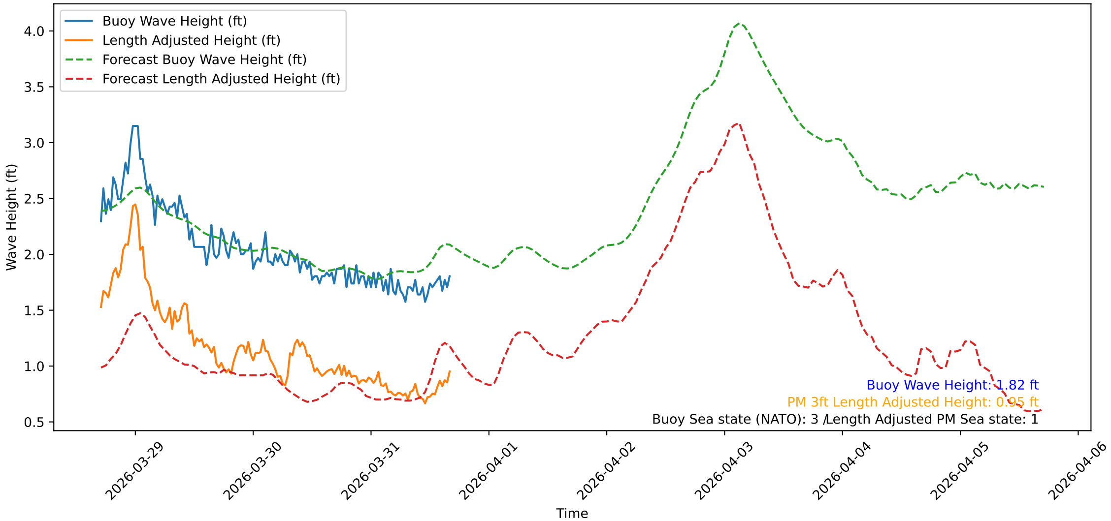
Wave Heights over Time for Oceanside Harbor at 2026-03-31 16:50:31
