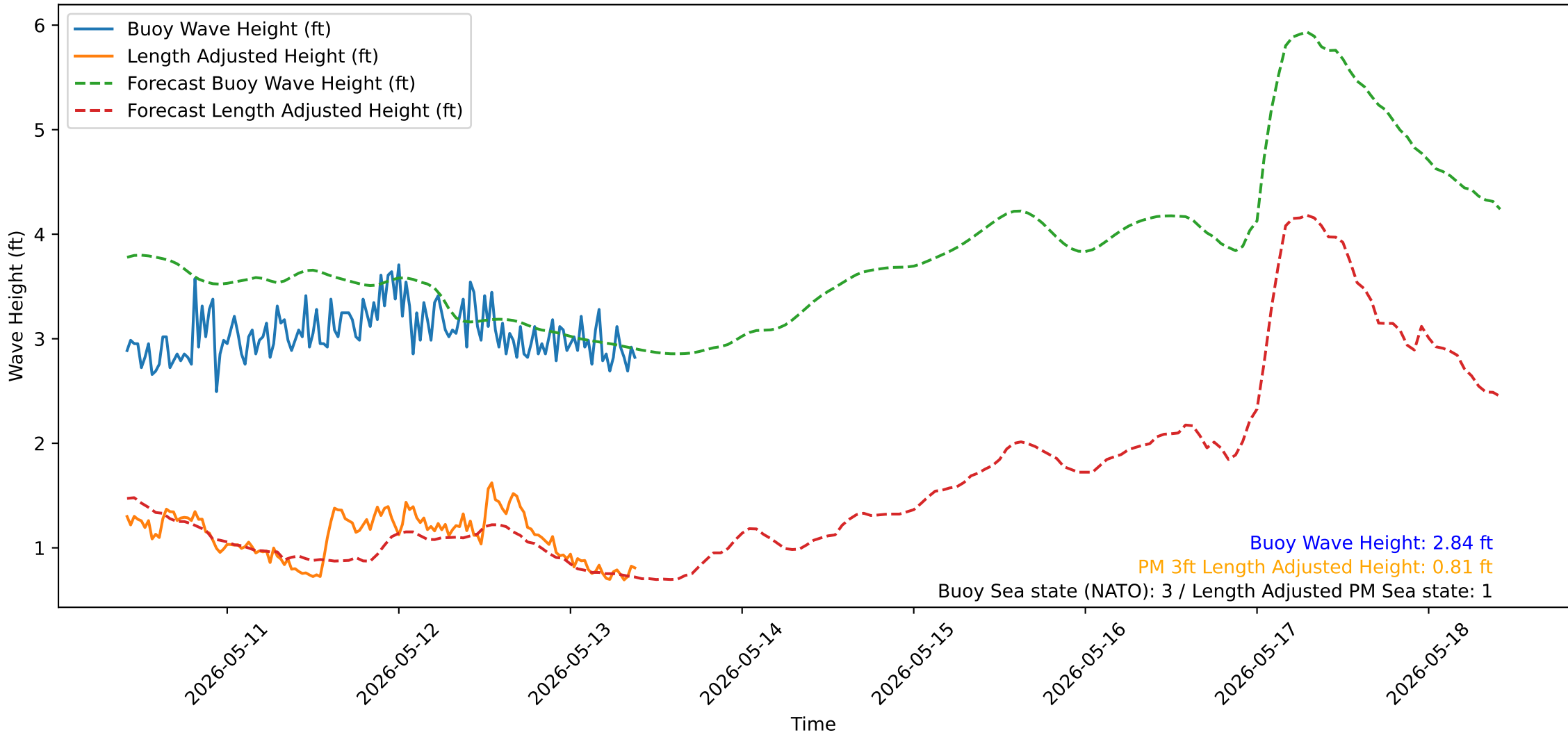
Wave Heights over Time for Oceanside Harbor at 2026-05-13 10:00:31
