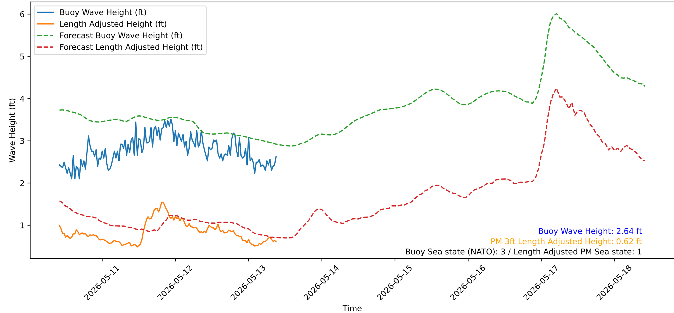
Wave Heights over Time for Green Beach at 2026-05-13 10:01:13
