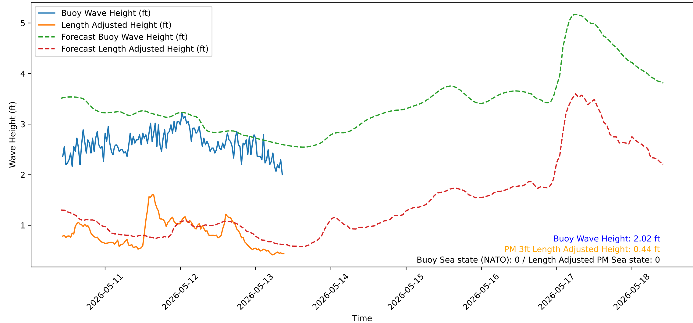
Wave Heights over Time for Red Beach at 2026-05-13 10:00:51
