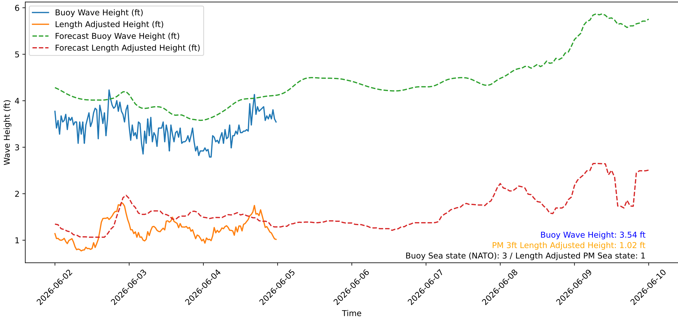
Wave Heights over Time for Green Beach at 2026-06-05 00:11:07
