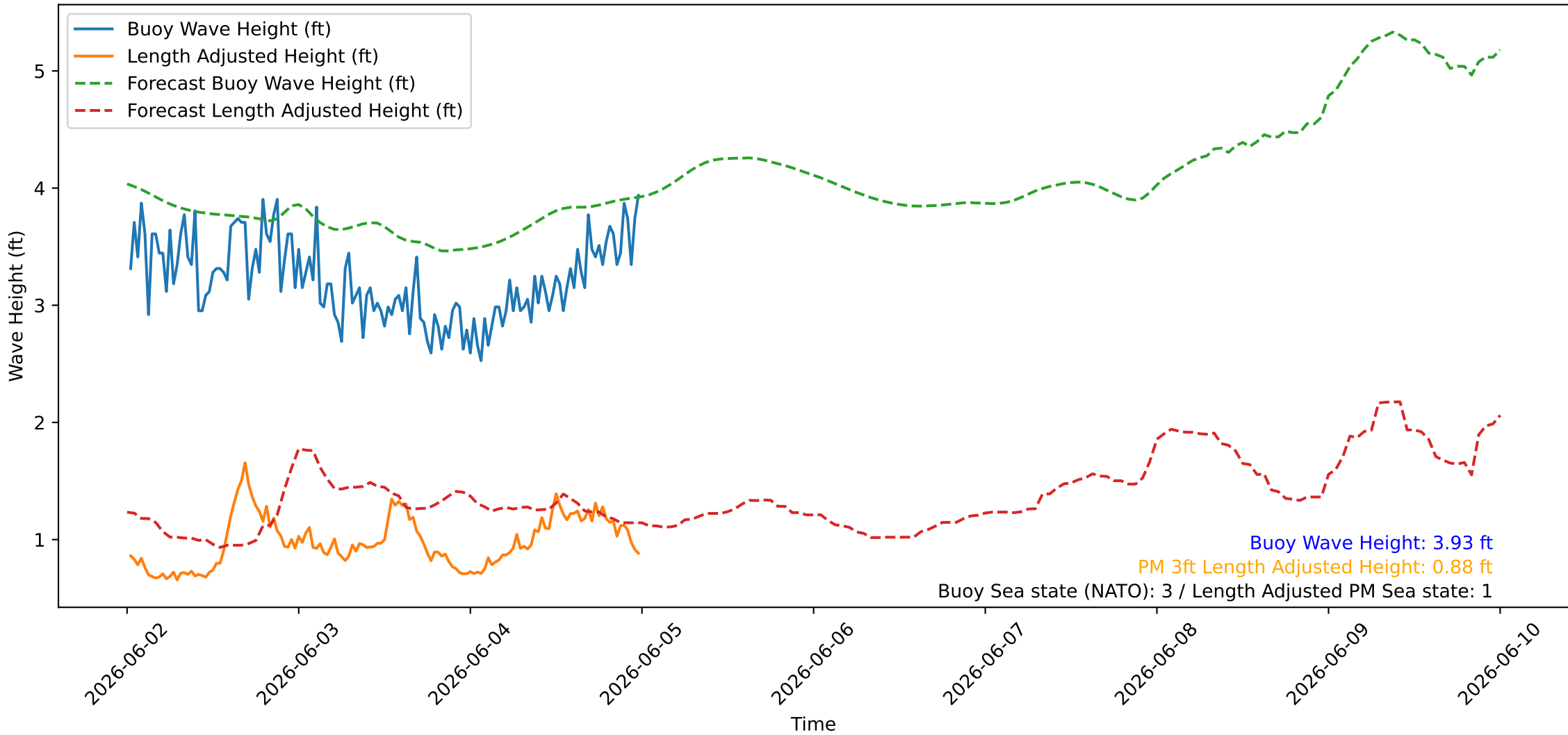
Wave Heights over Time for Red Beach at 2026-06-05 00:10:45
