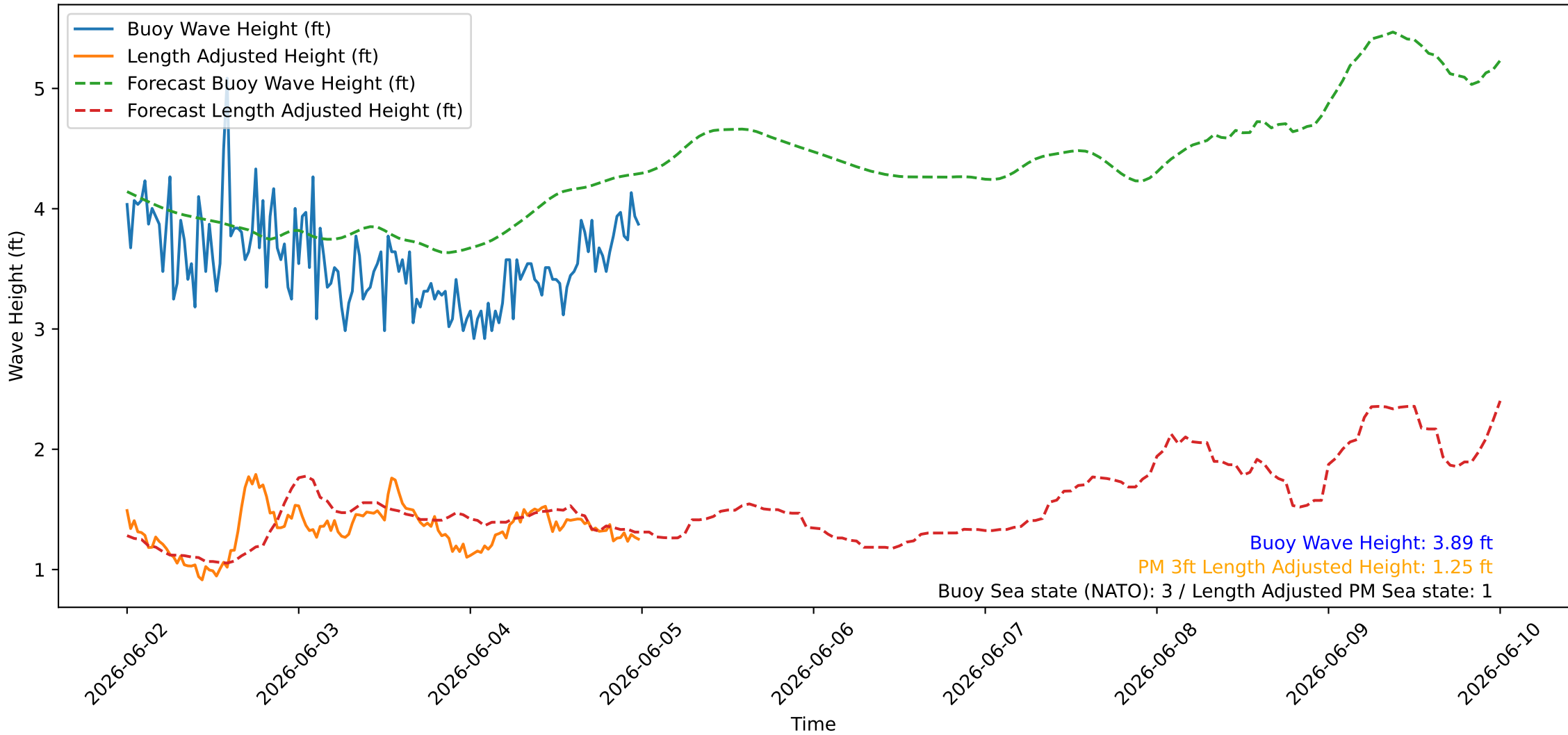
Wave Heights over Time for Oceanside Harbor at 2026-06-05 00:10:26
