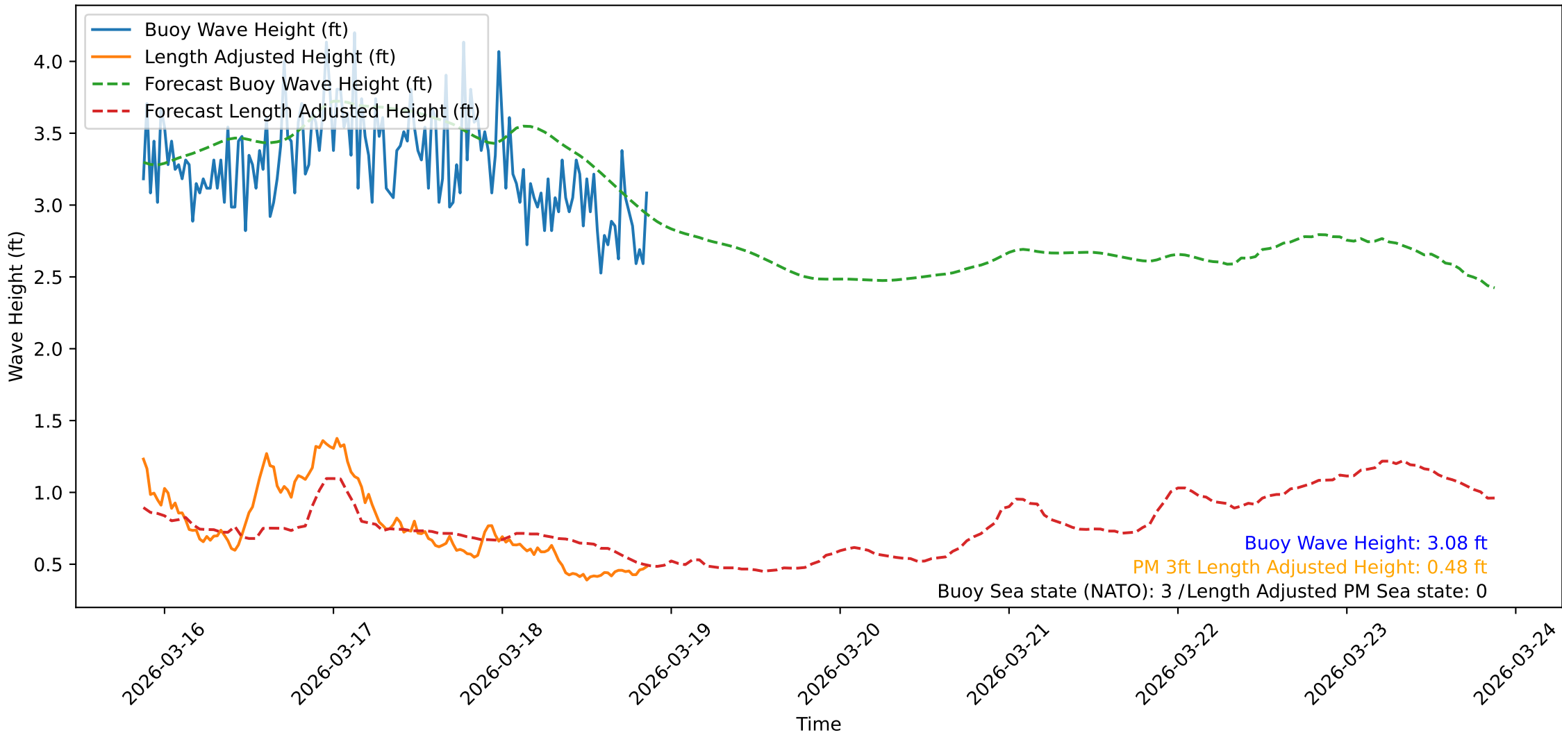
Wave Heights over Time for Green Beach at 2026-03-18 21:11:10
