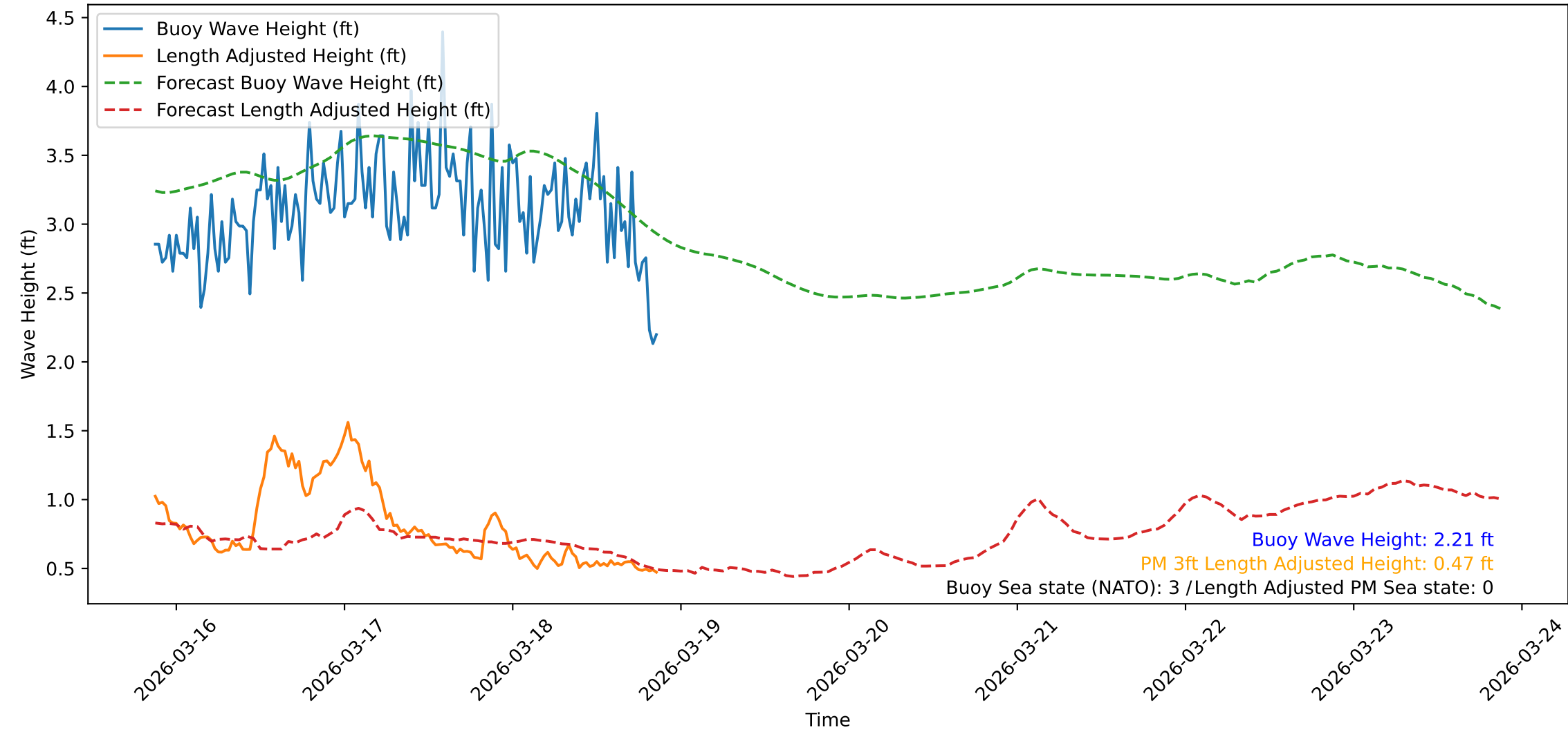
Wave Heights over Time for Oceanside Harbor at 2026-03-18 21:10:31
