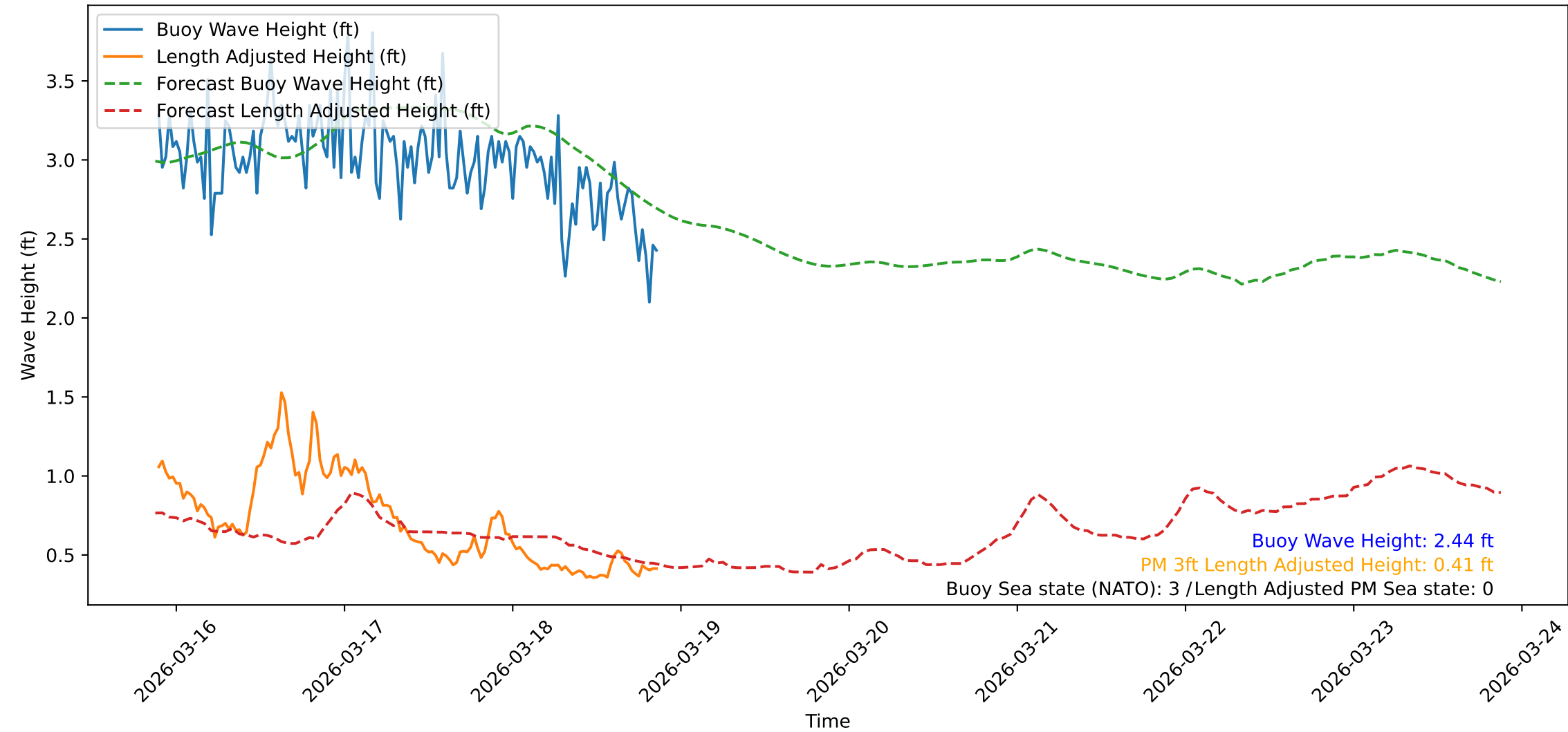
Wave Heights over Time for Red Beach at 2026-03-18 21:10:47
