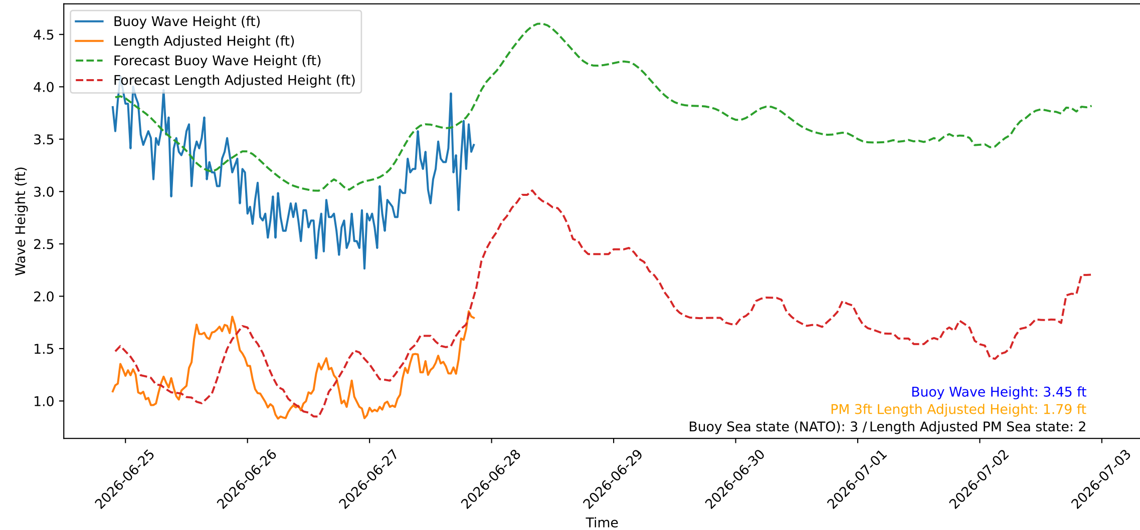
Wave Heights over Time for Green Beach at 2026-06-27 21:31:07
