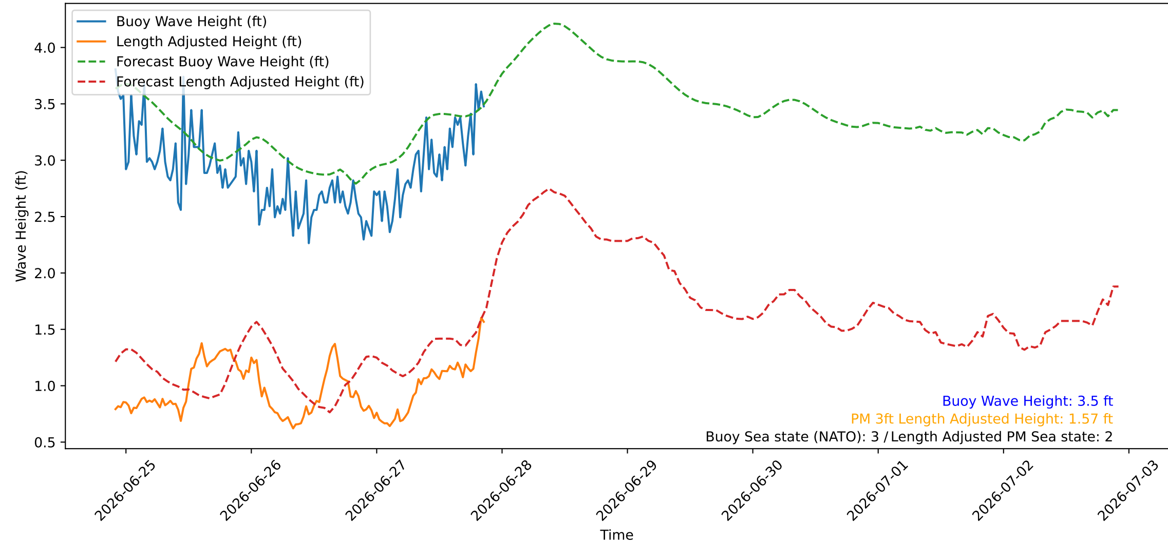
Wave Heights over Time for Red Beach at 2026-06-27 21:30:45
