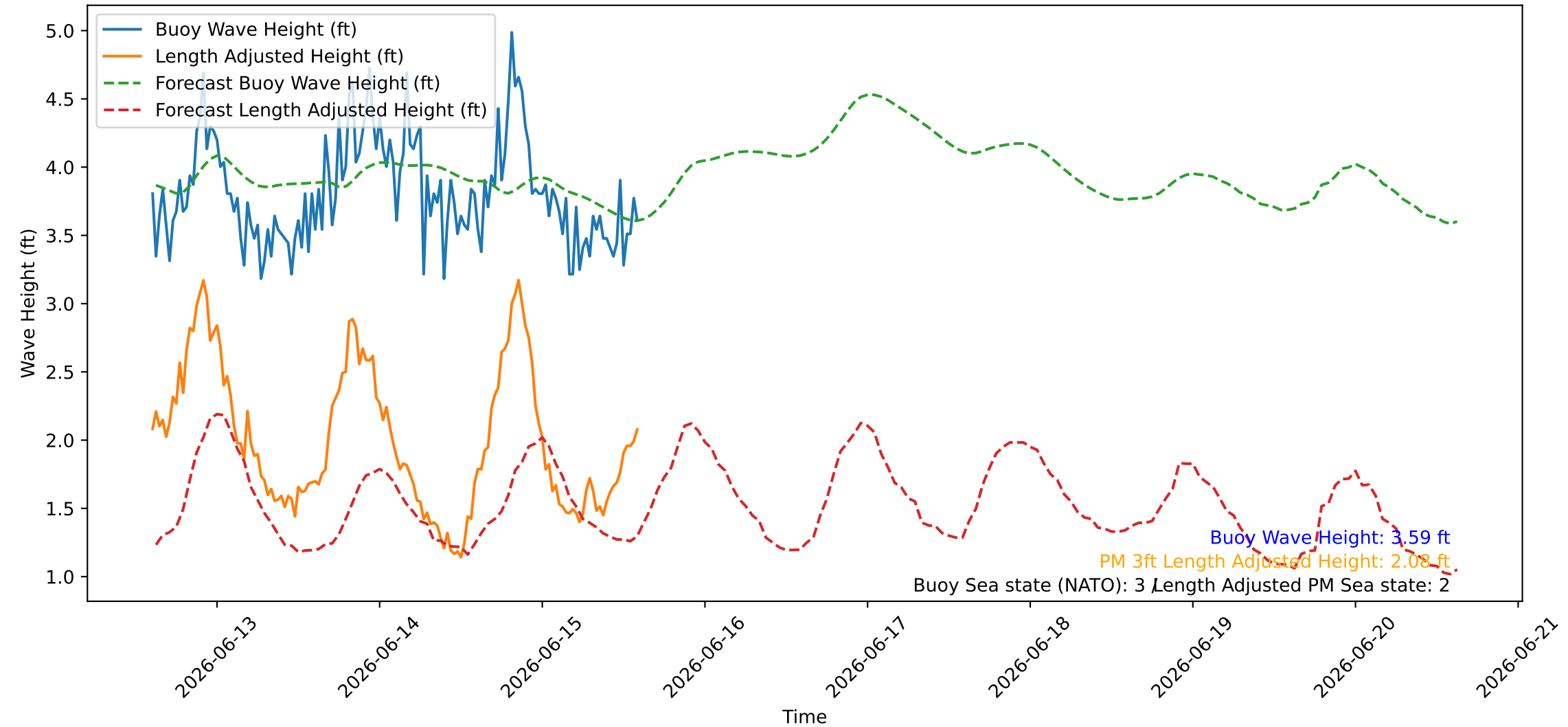
Wave Heights over Time for Oceanside Harbor at 2026-06-15 14:30:26
