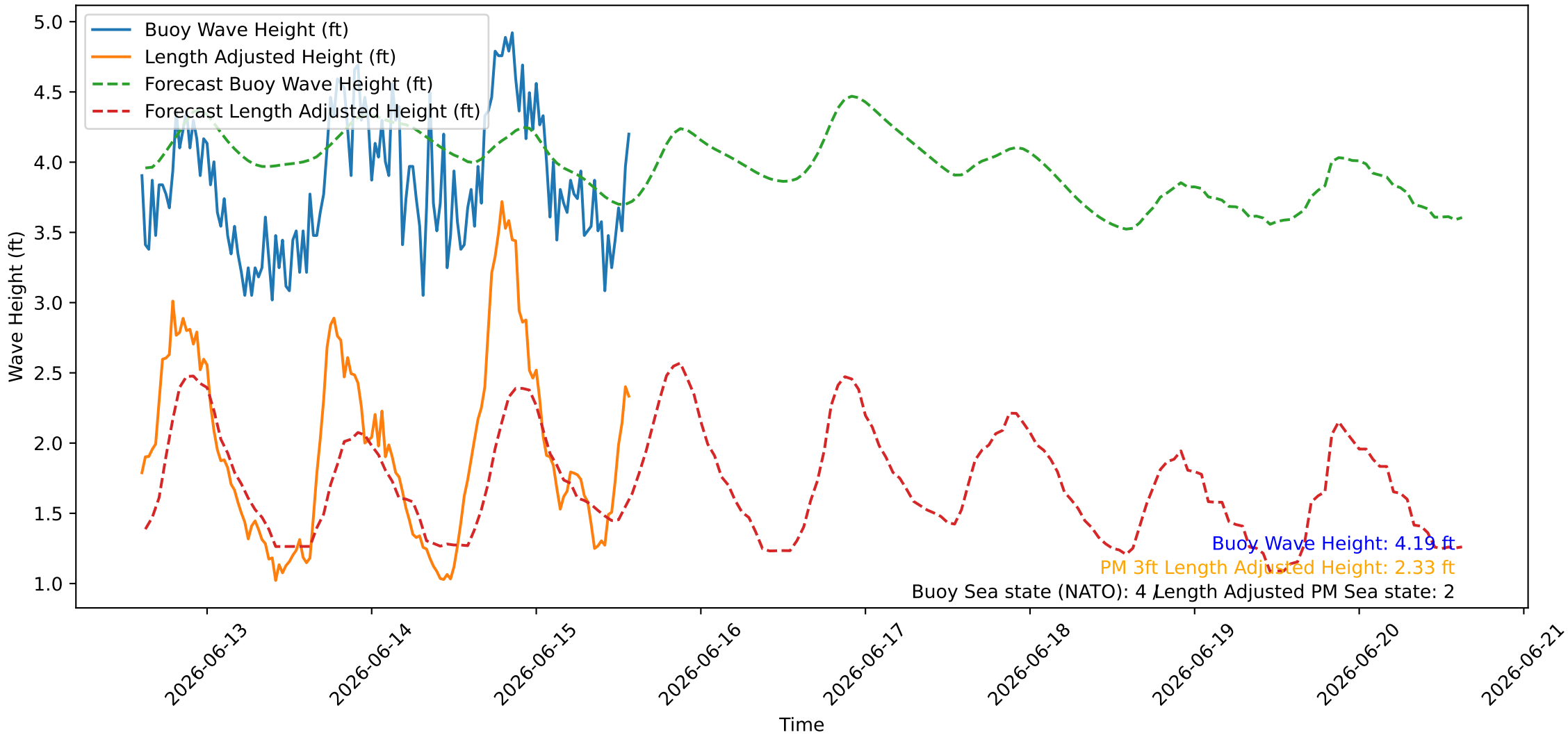
Wave Heights over Time for Green Beach at 2026-06-15 14:31:08
