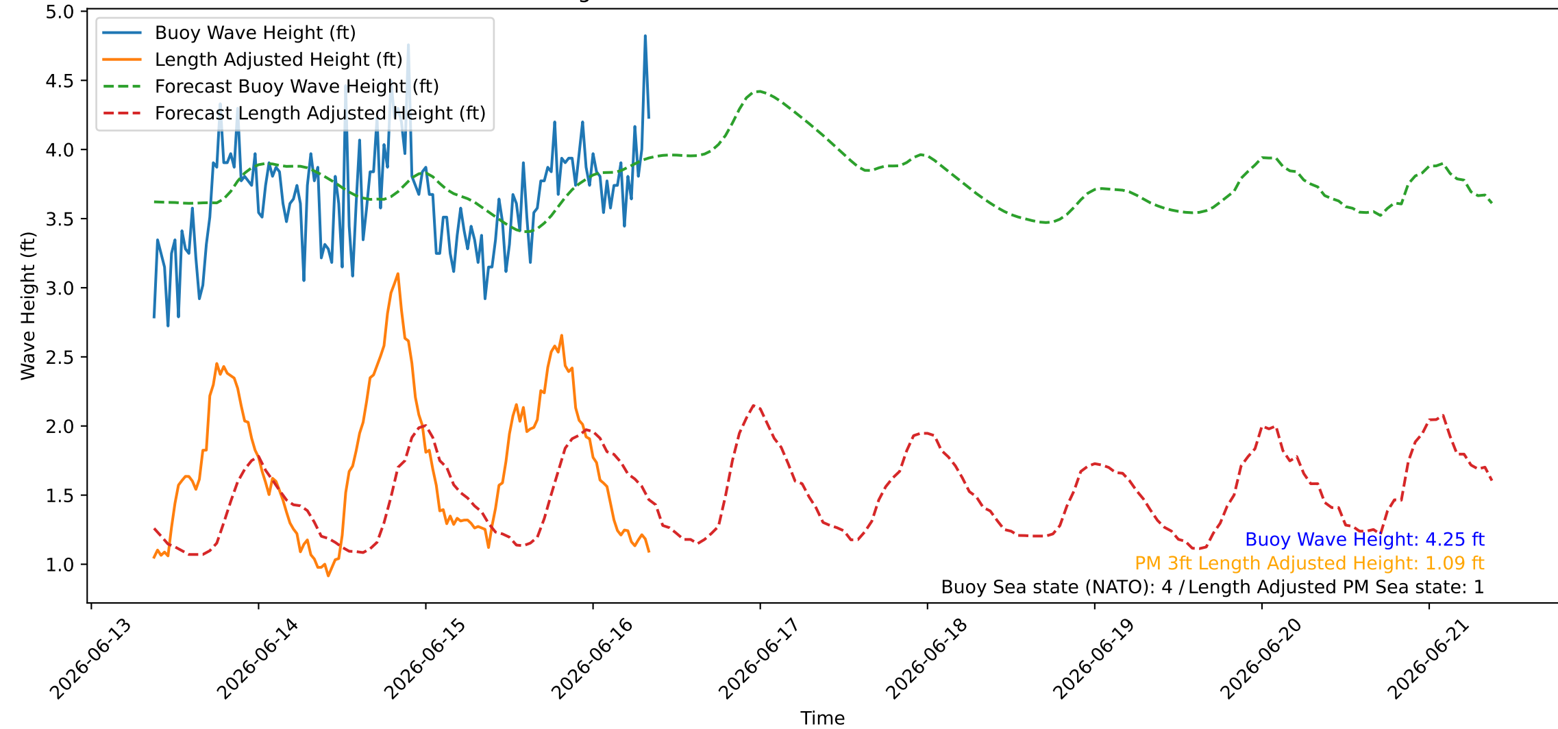
Wave Heights over Time for Red Beach at 2026-06-16 08:40:45
