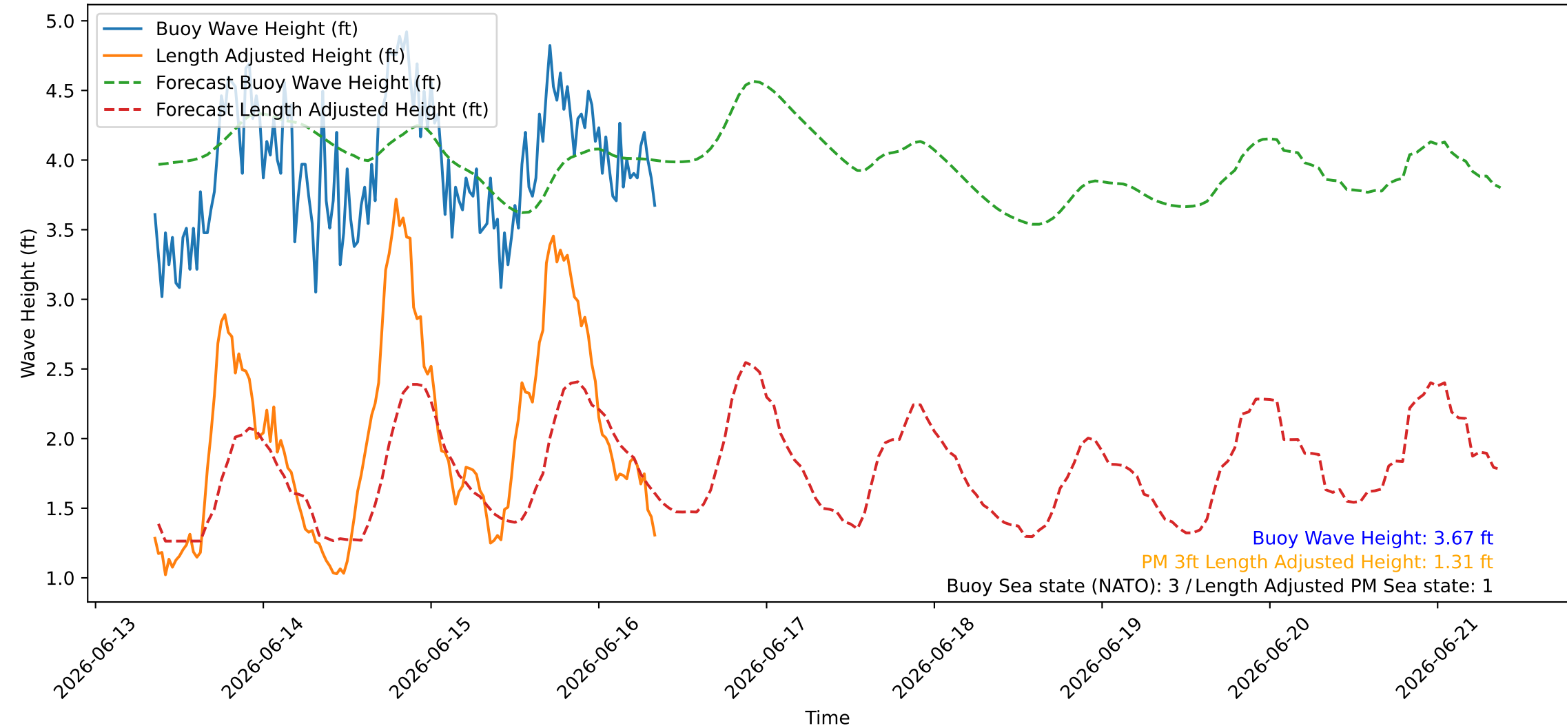
Wave Heights over Time for Green Beach at 2026-06-16 08:41:09
