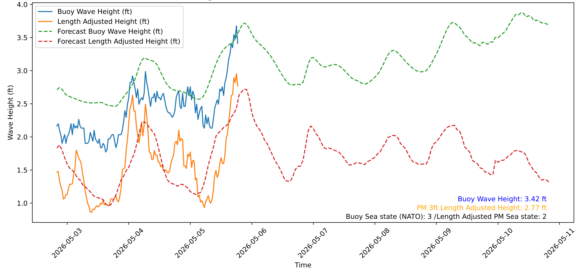
Wave Heights over Time for Green Beach at 2026-05-05 19:51:14
