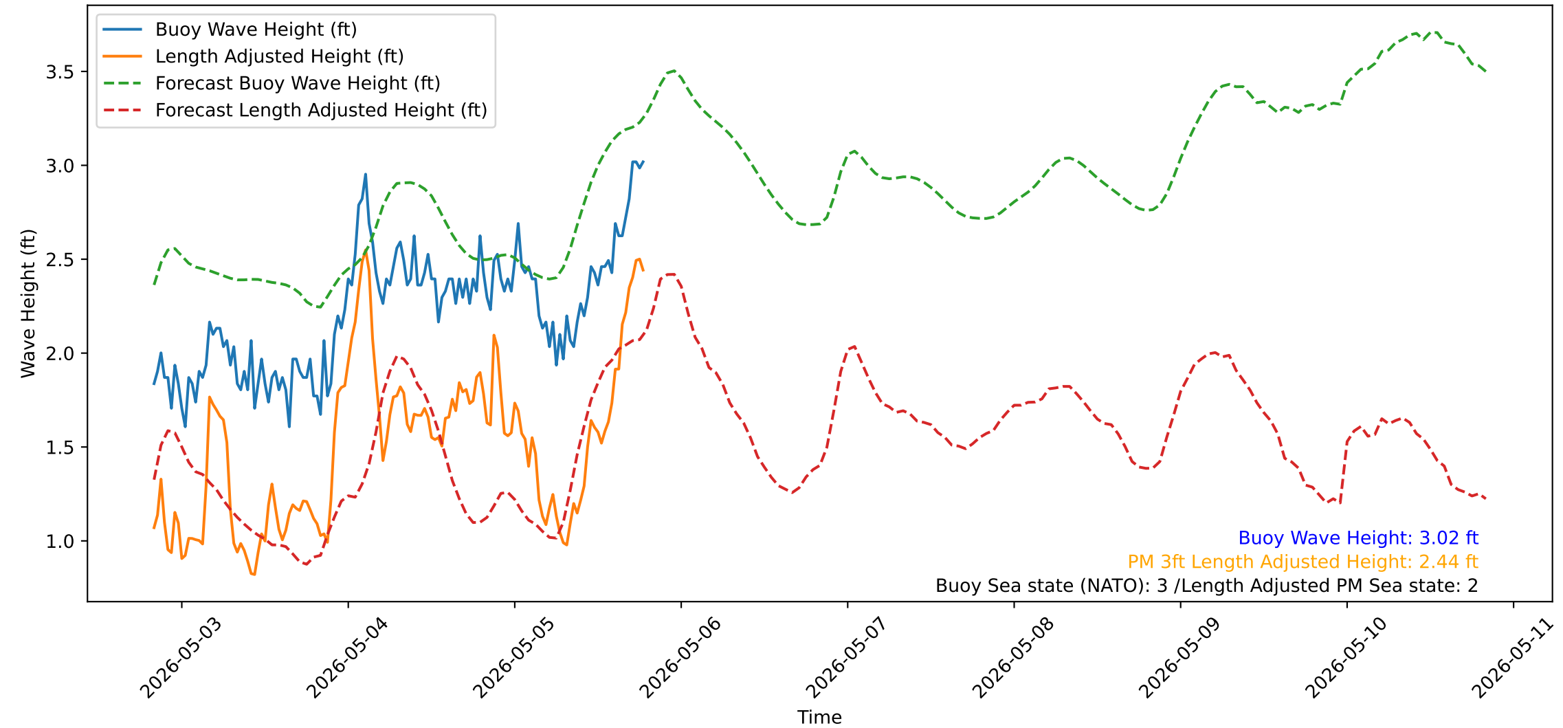
Wave Heights over Time for Red Beach at 2026-05-05 19:50:52
