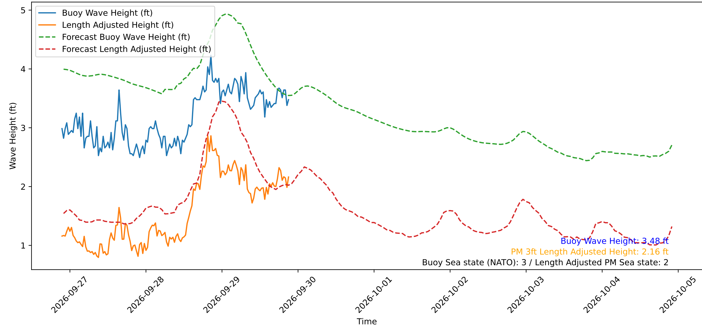
Wave Heights over Time for Oceanside Harbor at 2026-09-29 21:40:29
