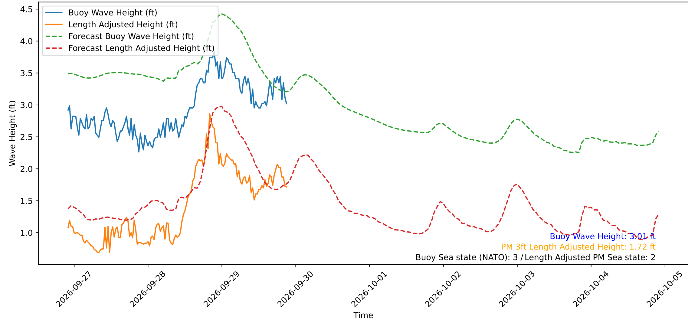
Wave Heights over Time for Red Beach at 2026-09-29 21:40:50
