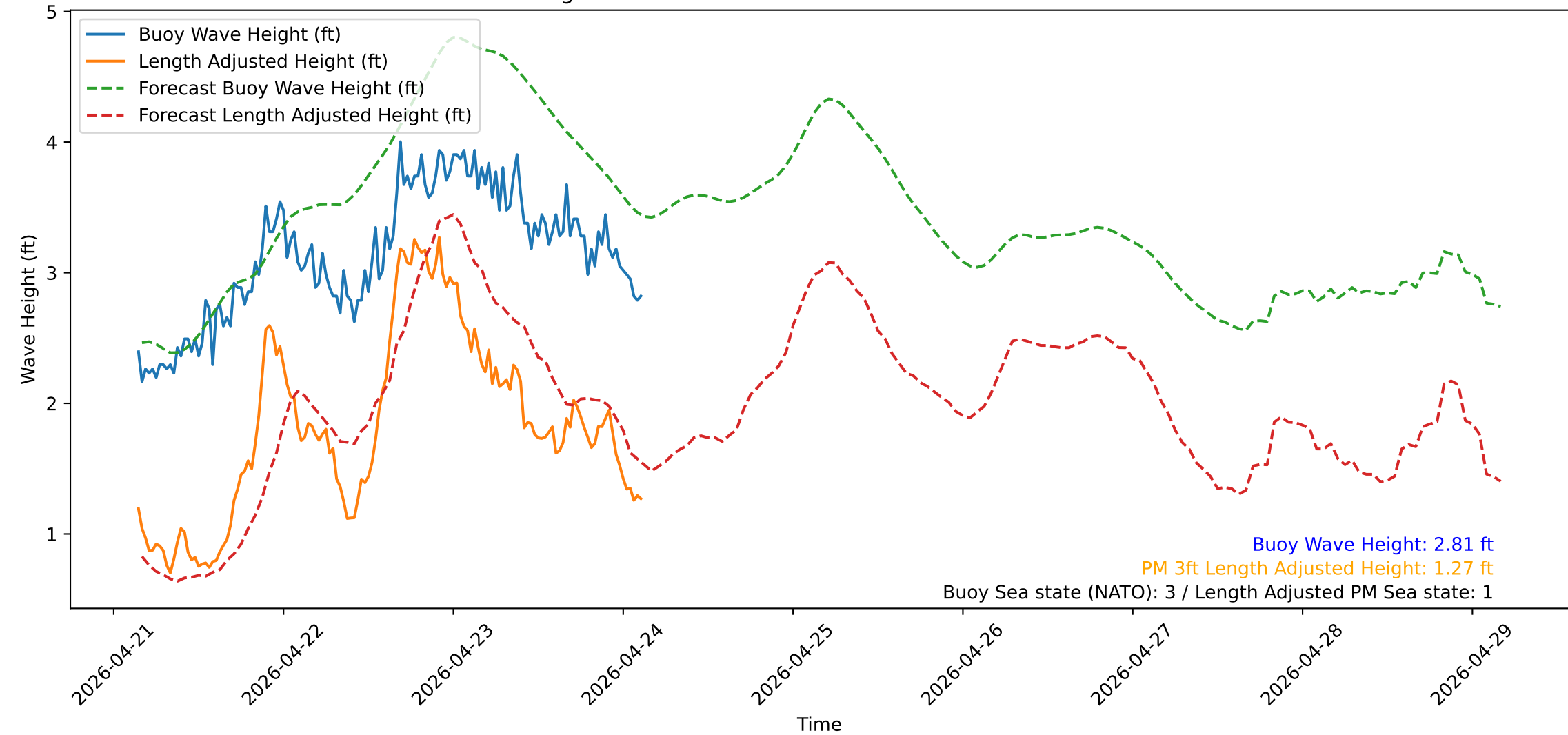
Wave Heights over Time for Green Beach at 2026-04-24 03:31:13
