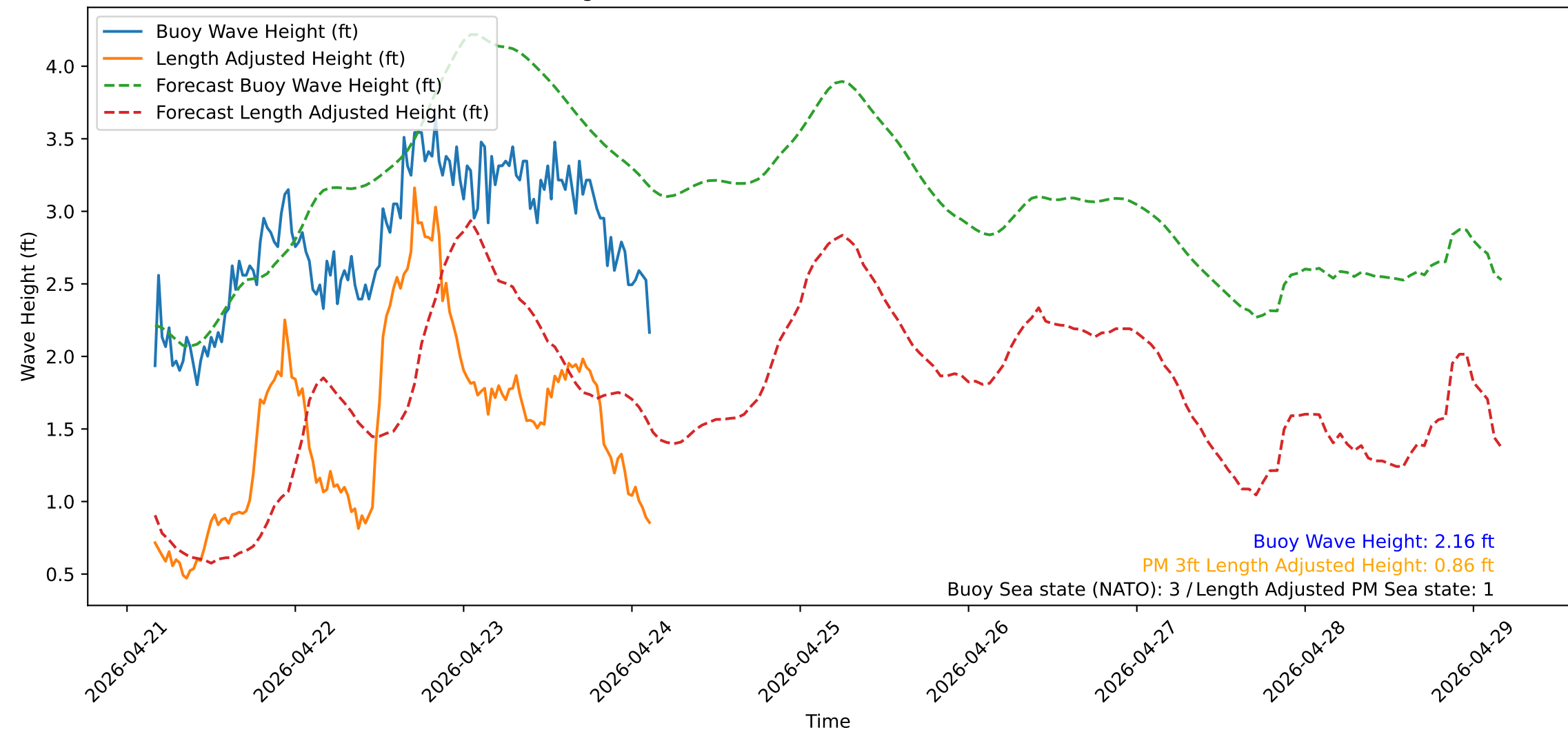
Wave Heights over Time for Red Beach at 2026-04-24 03:30:51
