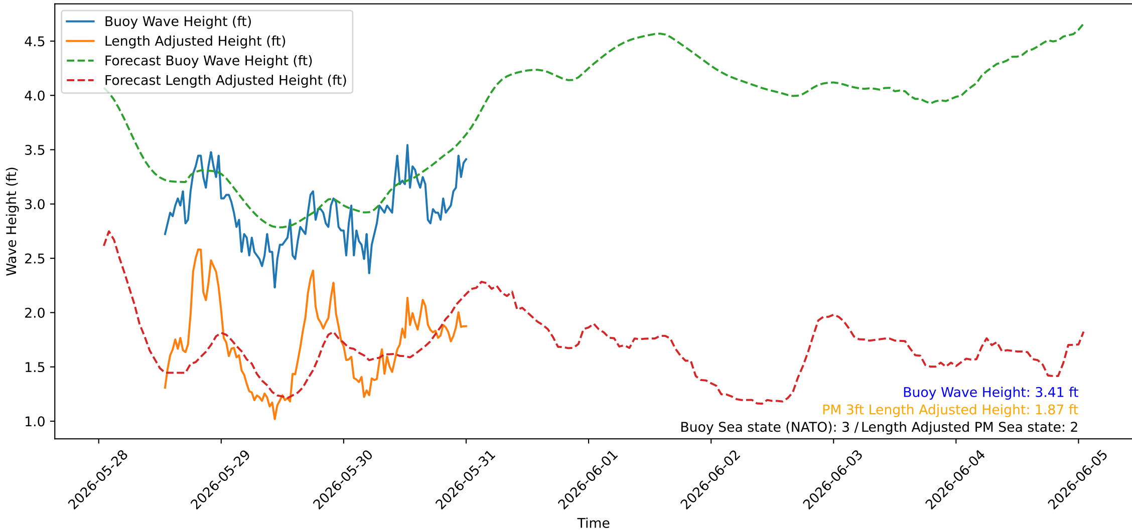
Wave Heights over Time for Oceanside Harbor at 2026-05-31 00:50:25
