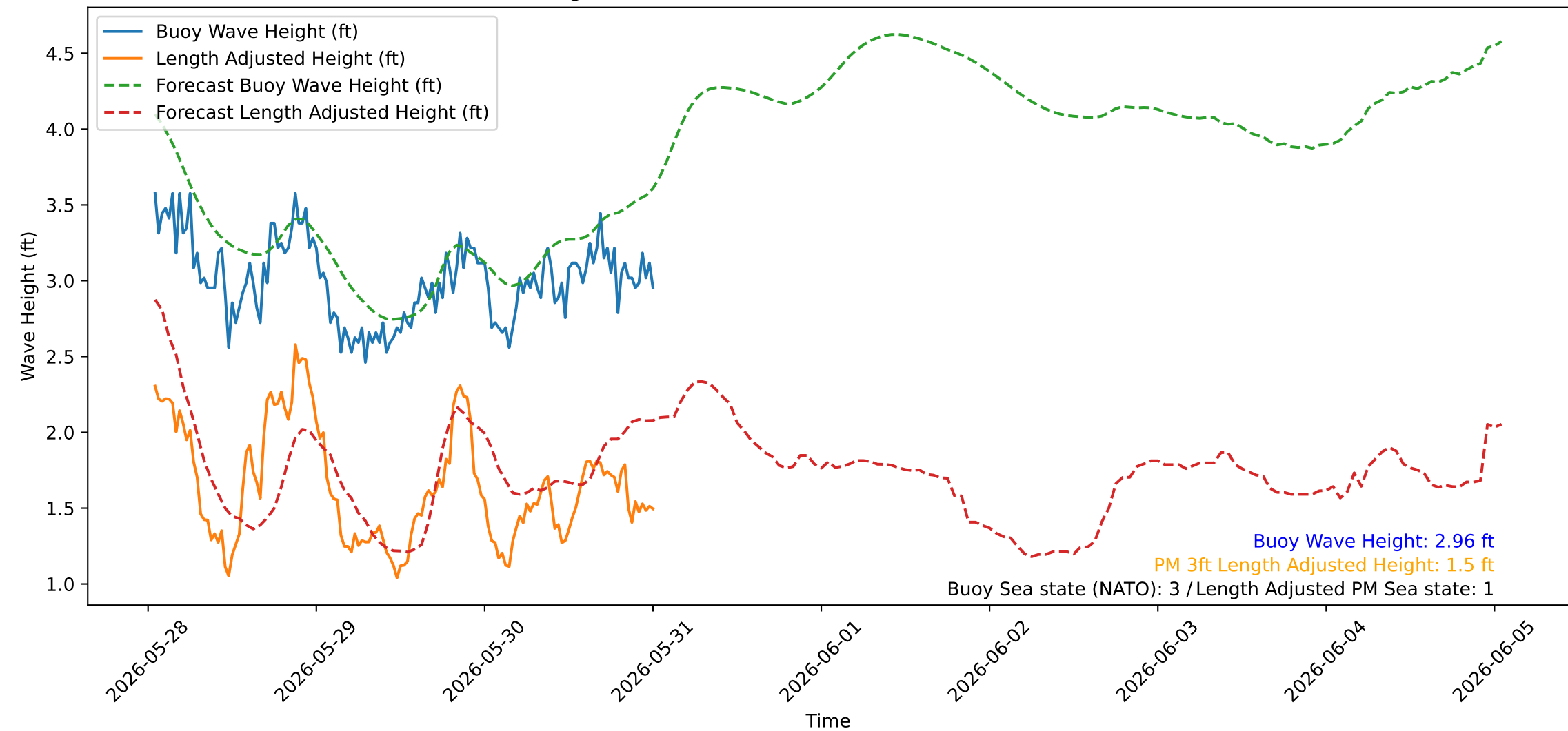
Wave Heights over Time for Green Beach at 2026-05-31 00:51:07
