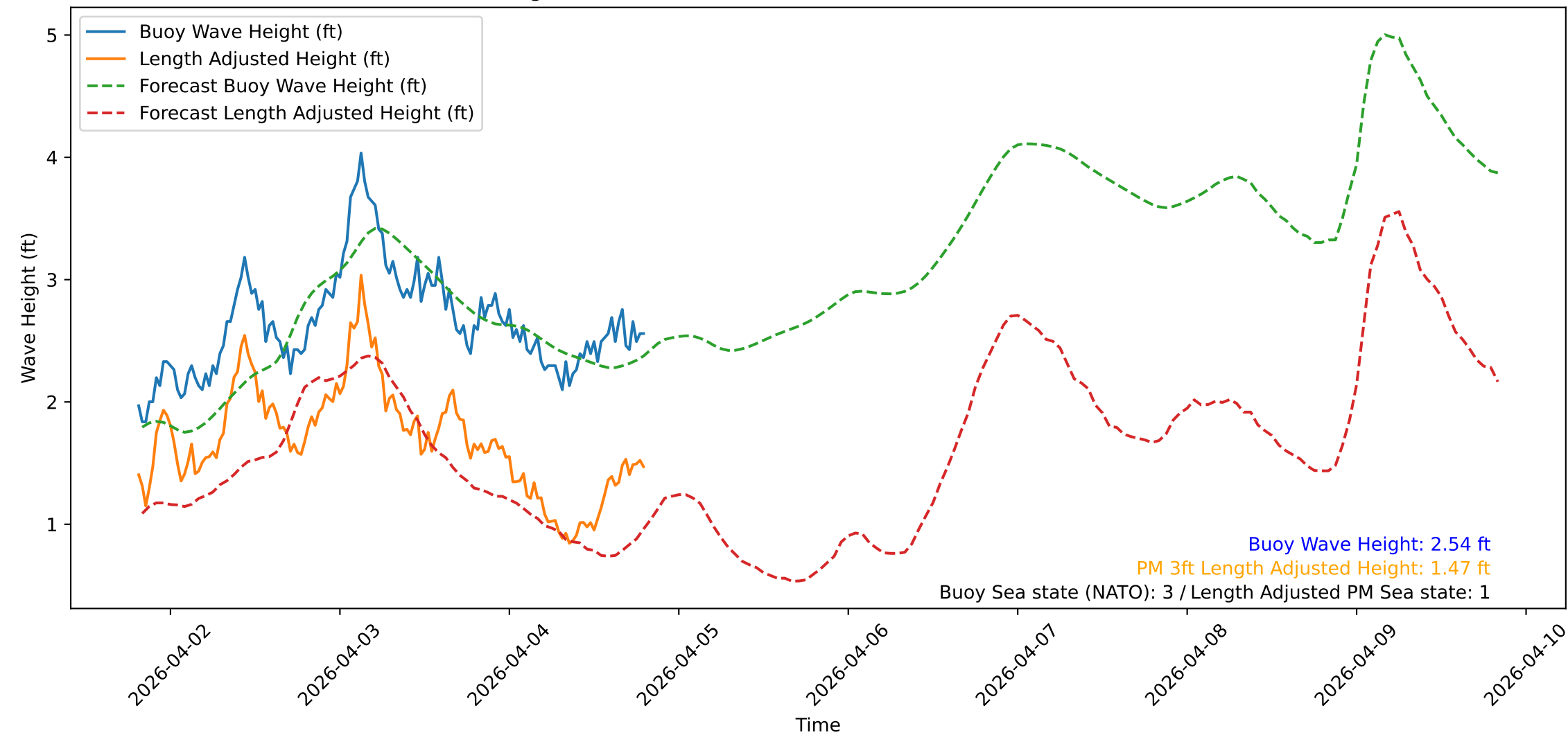
Wave Heights over Time for Oceanside Harbor at 2026-04-04 19:30:32
